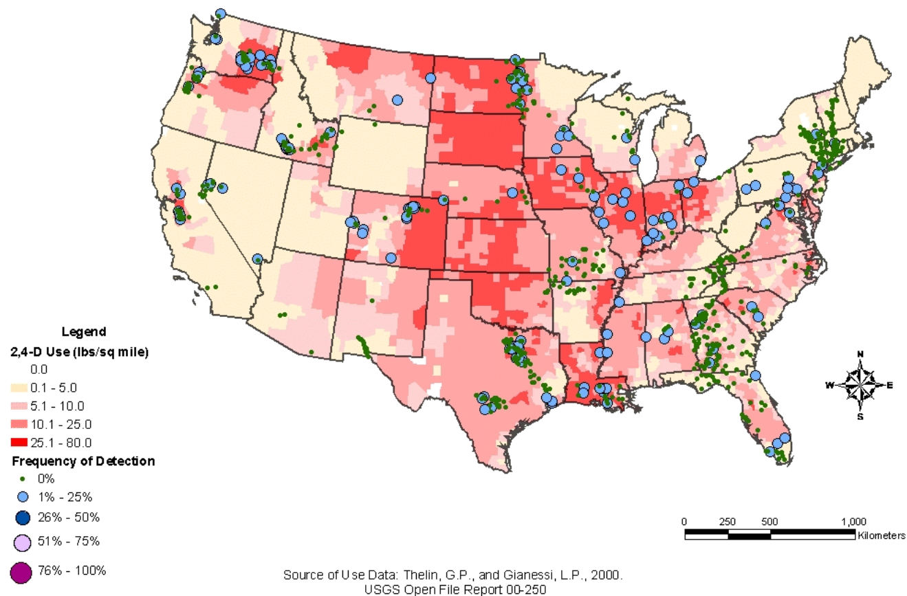
Figure 11 Frequency of Detection of 2,4-D at NAWQA Surface Water Locations Relative to 2,4-D County Level Use (USGS Open-File Report 00-250)
