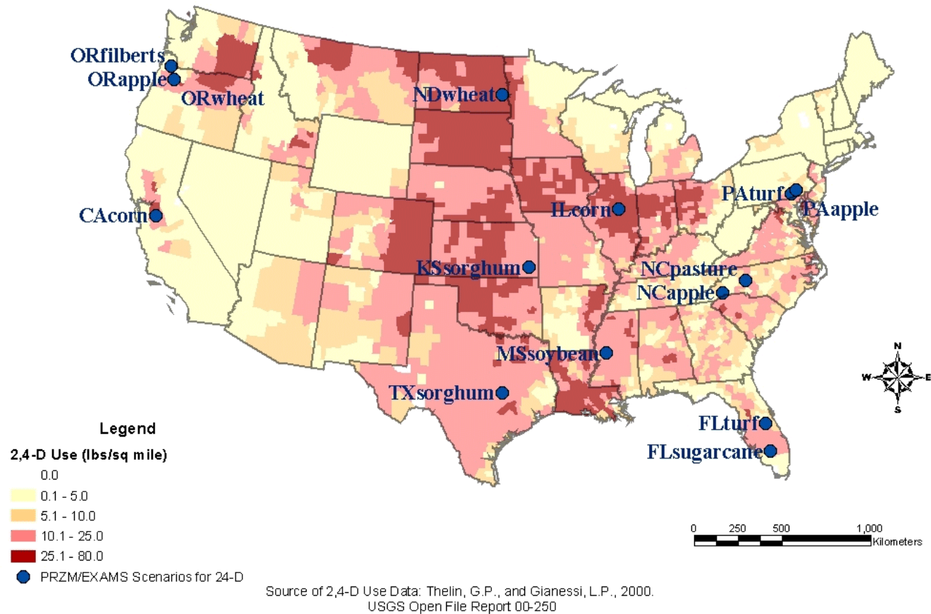
Figure 10. PRZM/EXAMS Scenarios Relative to 2,4-D County Level Use (USGS Open-File Report 00-250)
