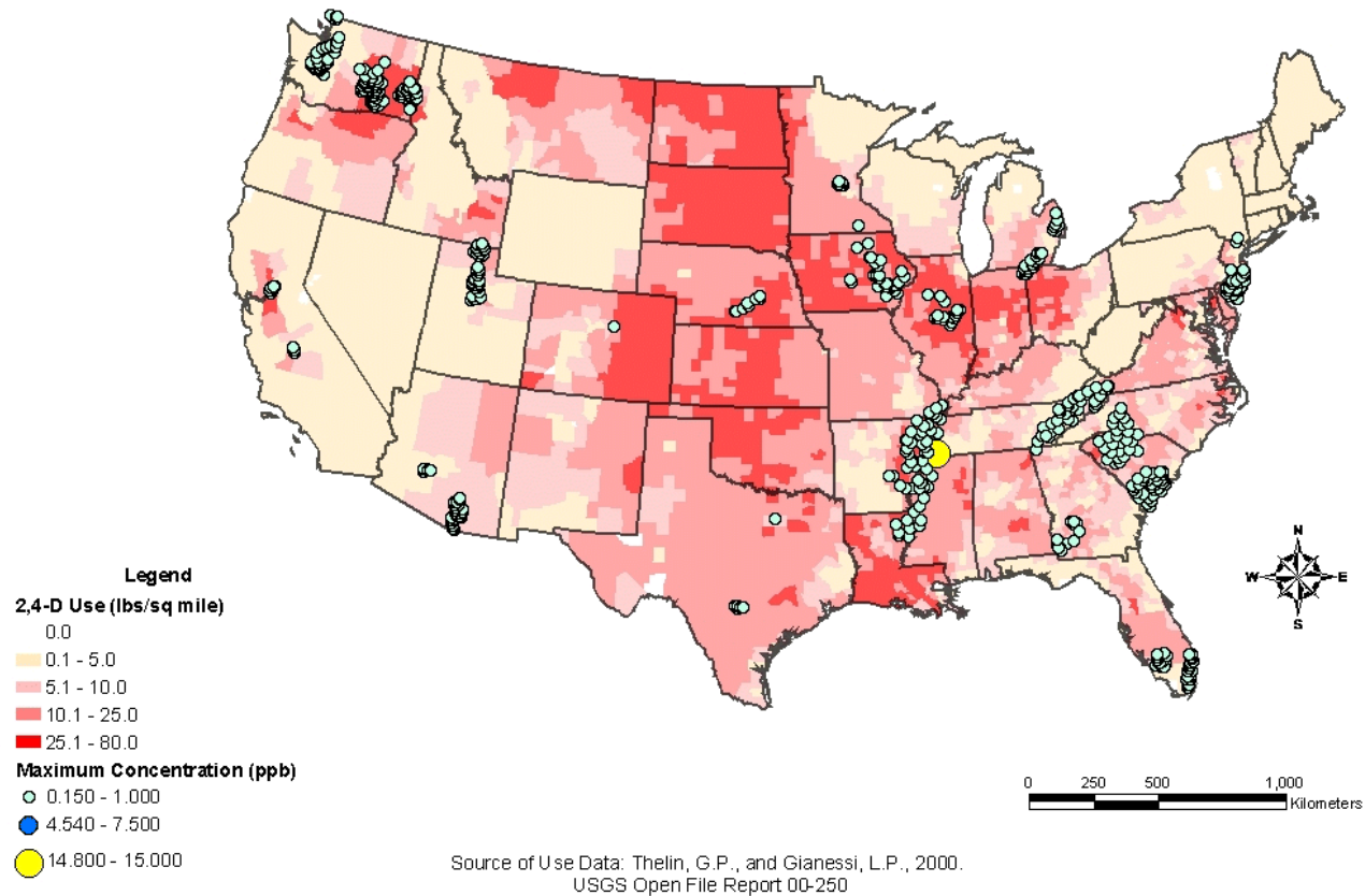
Figure 15. Concentration of 2,4-D in Groundwater Greater than 0.15 ppb at NAWQA Groundwater Locations Relative to 2,4-D County Level Use (USGS Open-File Report 00-250)
