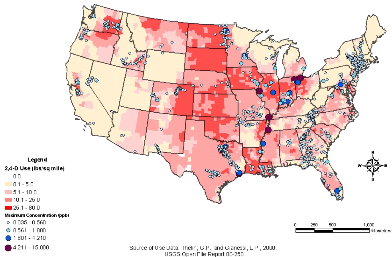
Figure 12. Maximum Concentrations of 2,4-D Greater Than 0.035 ppb at NAWQA Surface Water Locations Relative to 2,4-D County Level Use (USGS Open-File Report 00-250)
