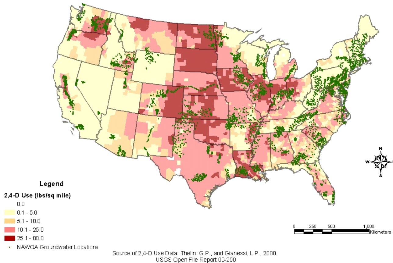
Figure 8. NAWQA Groundwater Locations Relative to 2,4-D County Level Use (USGS Open-File Report 00-250)
