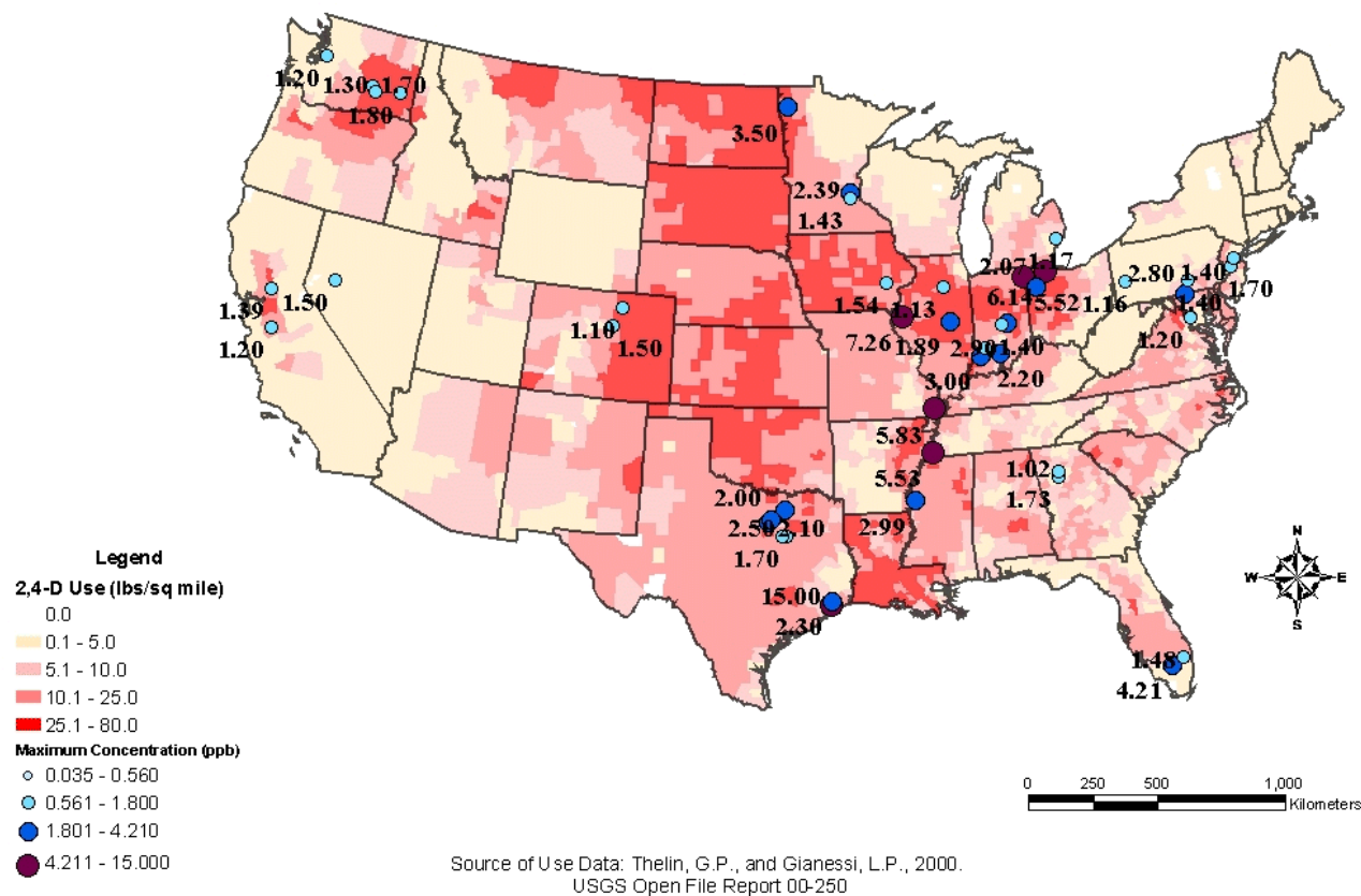
Figure 13. Maximum Concentrations of 2,4-D Greater than 1.0 ppb at NAWQA Surface Water Locations Relative to 2,4-D County Level Use (USGS Open-File Report 00-250)
