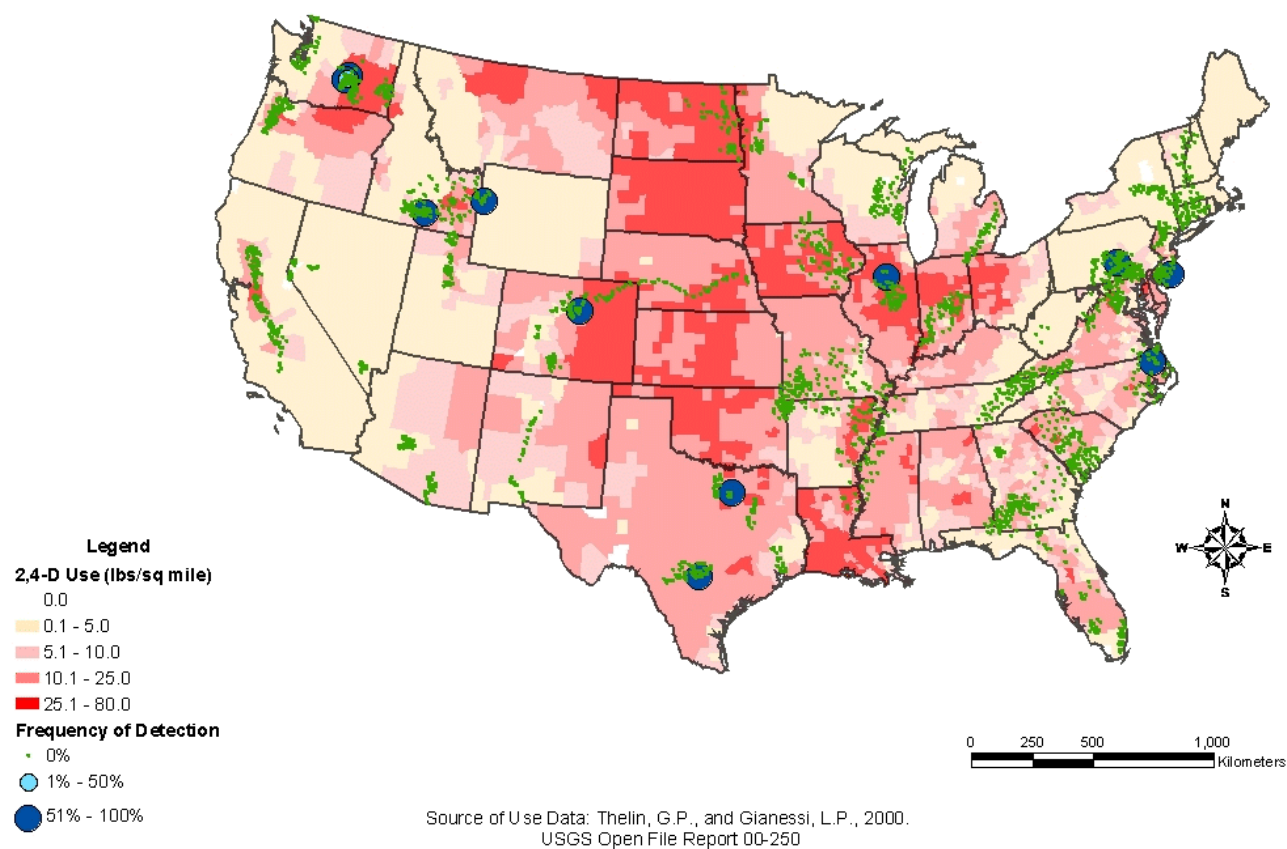
Figure 14. Frequency of Detection of 2,4-D at NAWQA Groundwater Locations Relative to 2,4-D County Level Use (USGS Open-File Report 00-250)
