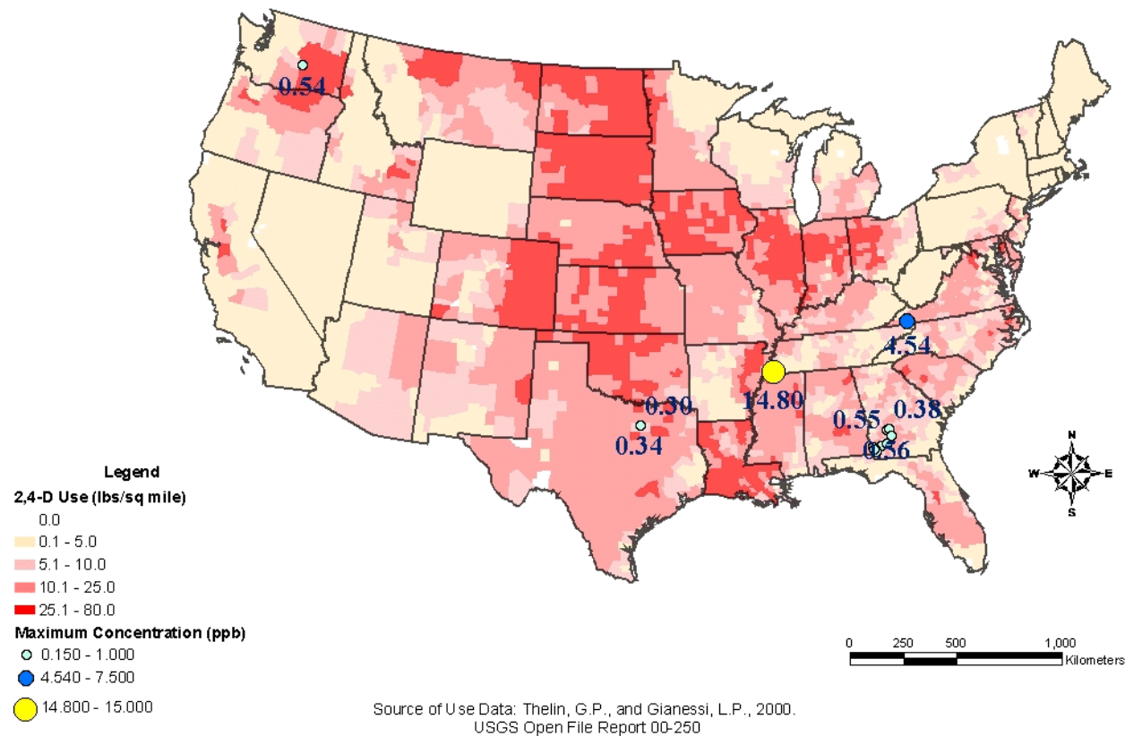
Figure 16. Concentration of 2,4-D in Groundwater Greater than 0.25 ppb at NAWQA Groundwater Locations Relative to 2,4-D County Level Use (USGS Open-File Report 00-250)
