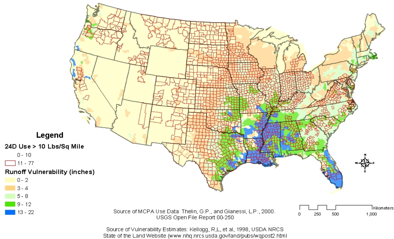
Figure 3. Runoff Vulnerability (Kellogg, et al, 1998) versus 2,4-D County Level Use Greater than 10 lbs/sq mile (USGS Open File Report 00-250)
