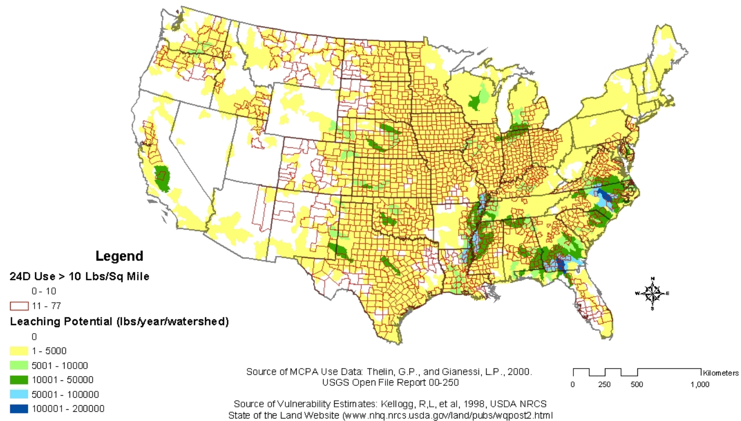
Figure 4. Leaching Potential (Kellogg, et al, 1998) versus 2,4-D County Level Use Greater than 10 lbs/sq mile (USGS Open File Report 00-250)
