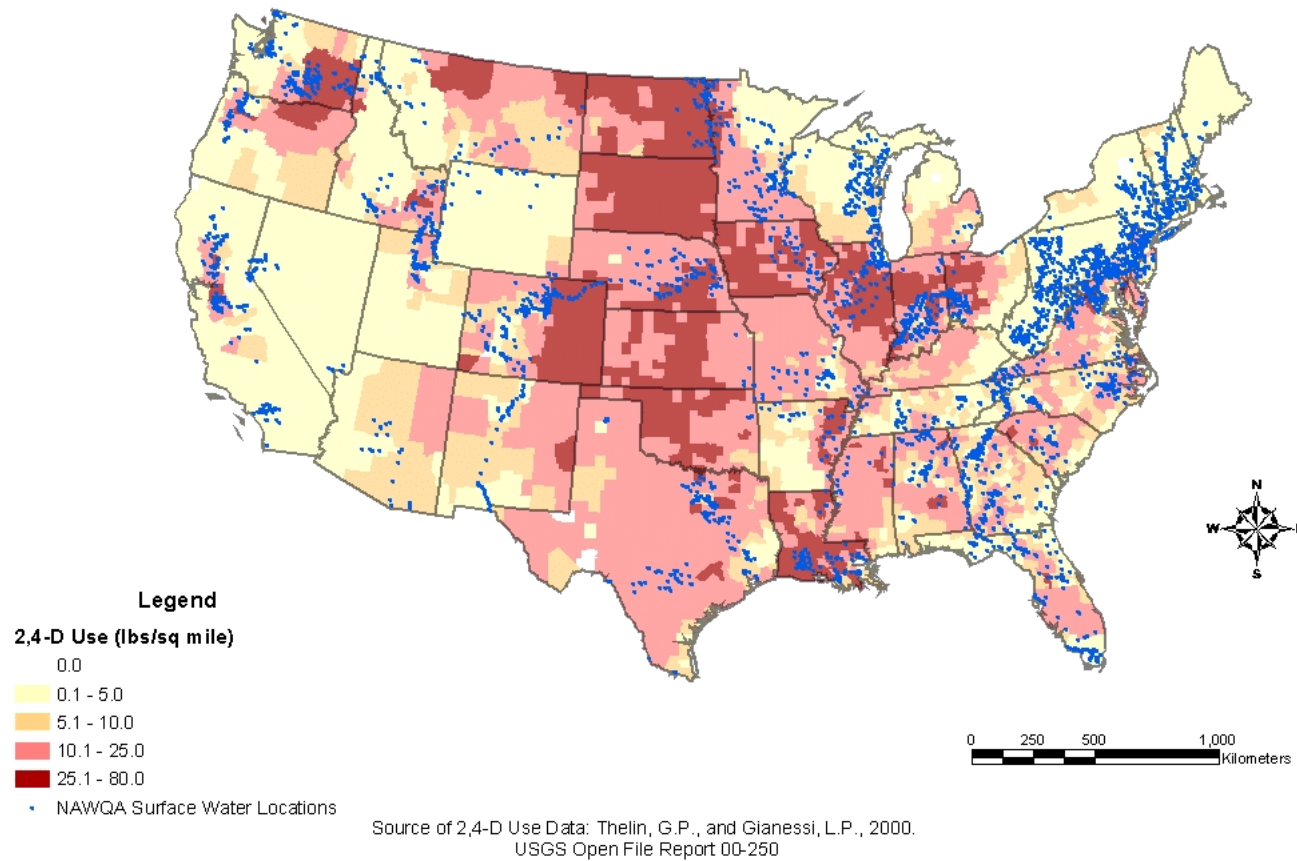
Figure 5. NAWQA Surface Water Locations Relative to Total 2,4-D County Level Use (USGS Open-File Report 00-250)
