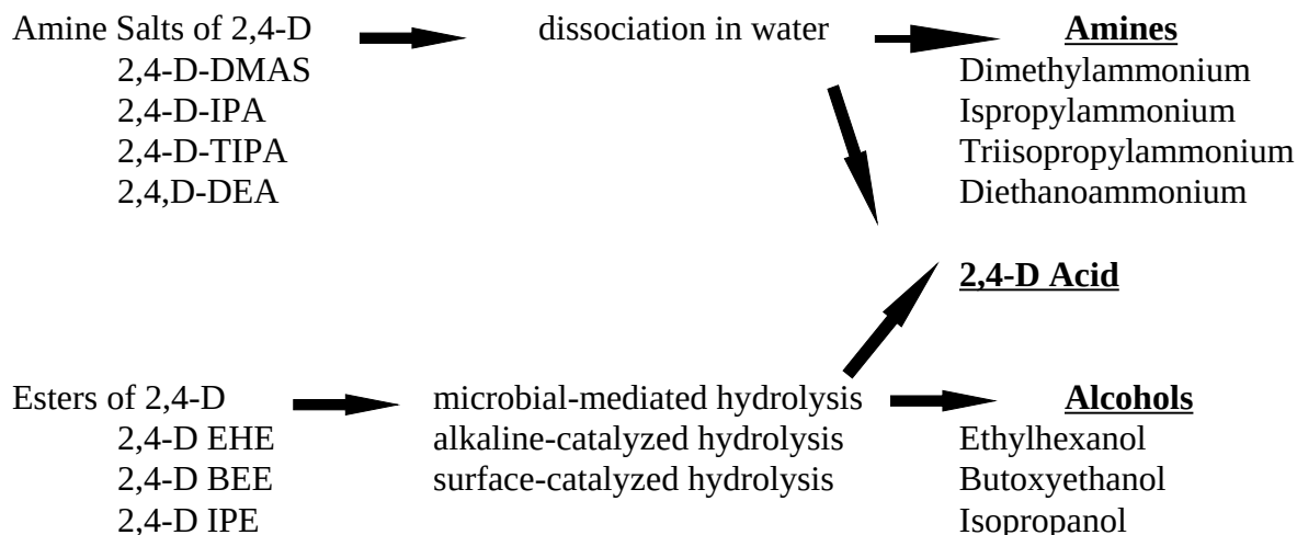
Figure 1. Schematic of Bridging Strategy of 2,4-D amine salts and 2,4-D esters to 2,4-D
