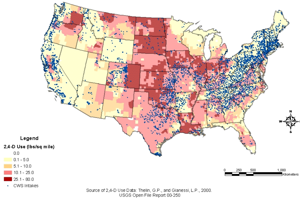
Figure 1. Community Water System (CWS) Intakes from Surface Water versus 2,4-D County Level Use Information (USGS Open File Report 00-250)
