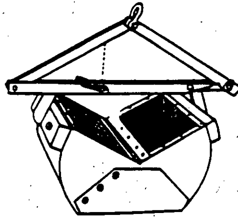
Figure B-3. Common Sediment Samplers
