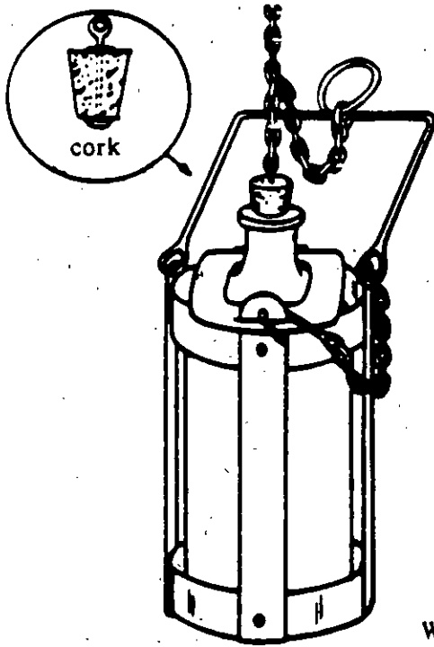
1000-ml(1-quart) weighted- bottle catcher
