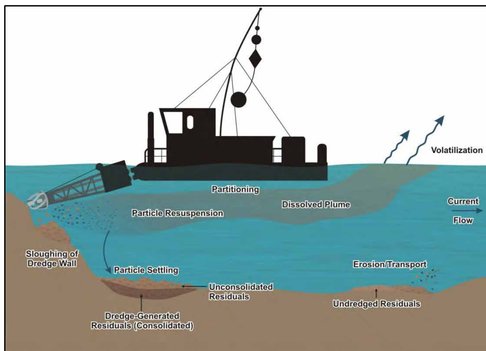
Figure 1-1. Conceptual Model of Sediment Residuals During a Typical Dredging Operation
