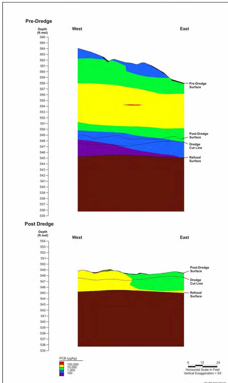
Figure 3-24. Comparison of Pre- and Post-Dredge Cross-Section t-PCBs in Sediment at T172
