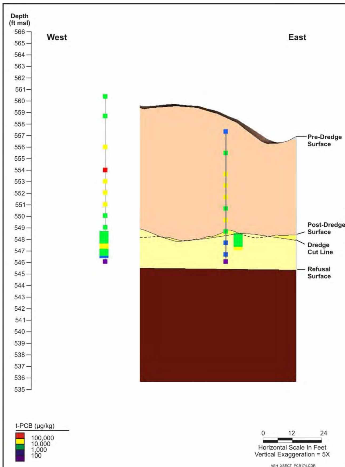
Figure 3-35. Cross-Section of T174 Showing Estimated Dredge Cut Line vs. Post-Dredge Bathymetry
