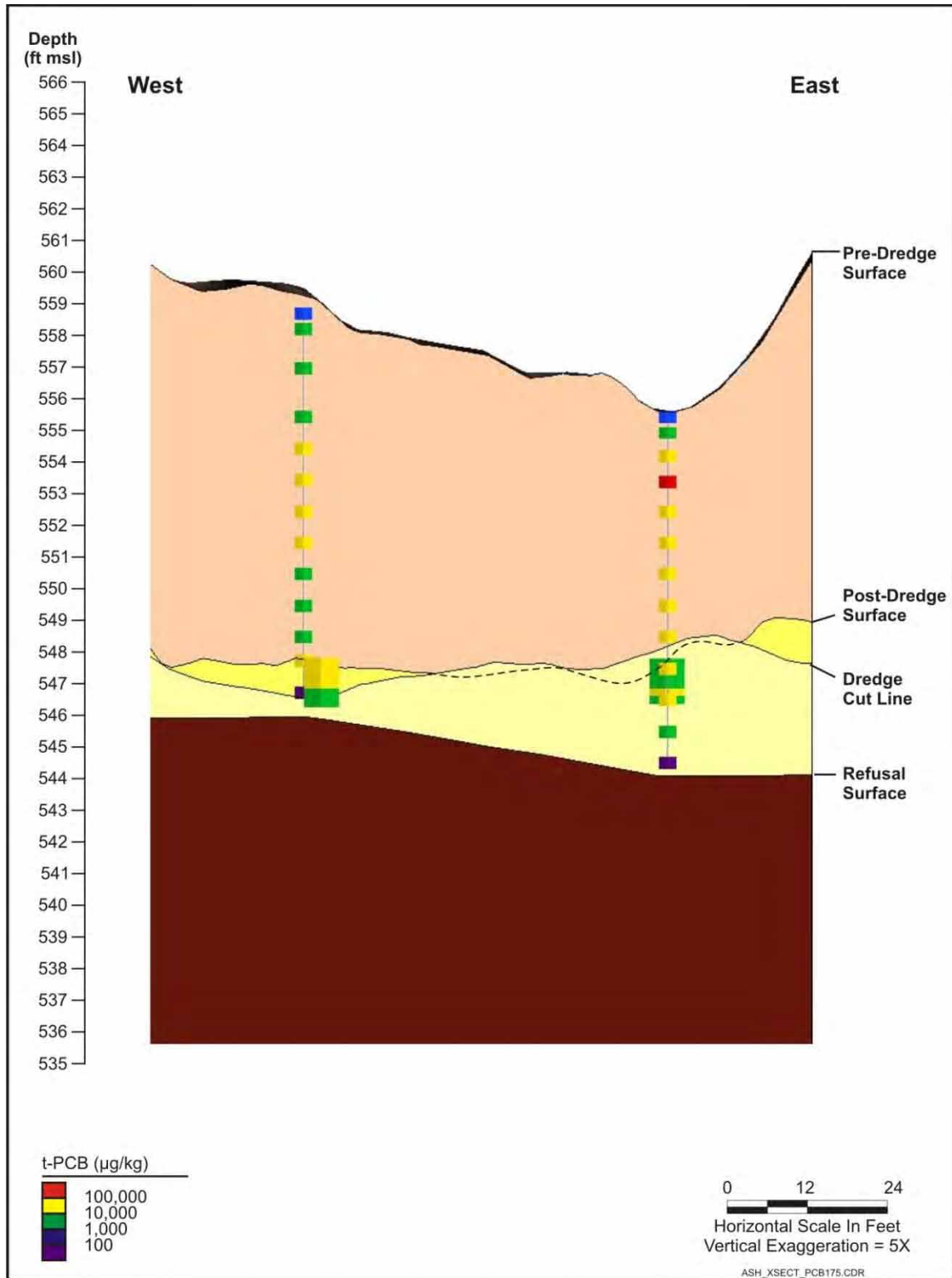
Figure 3-34. Cross-Section of T175 Showing Estimated Dredge Cut Line vs. Post-Dredge Bathymetry
