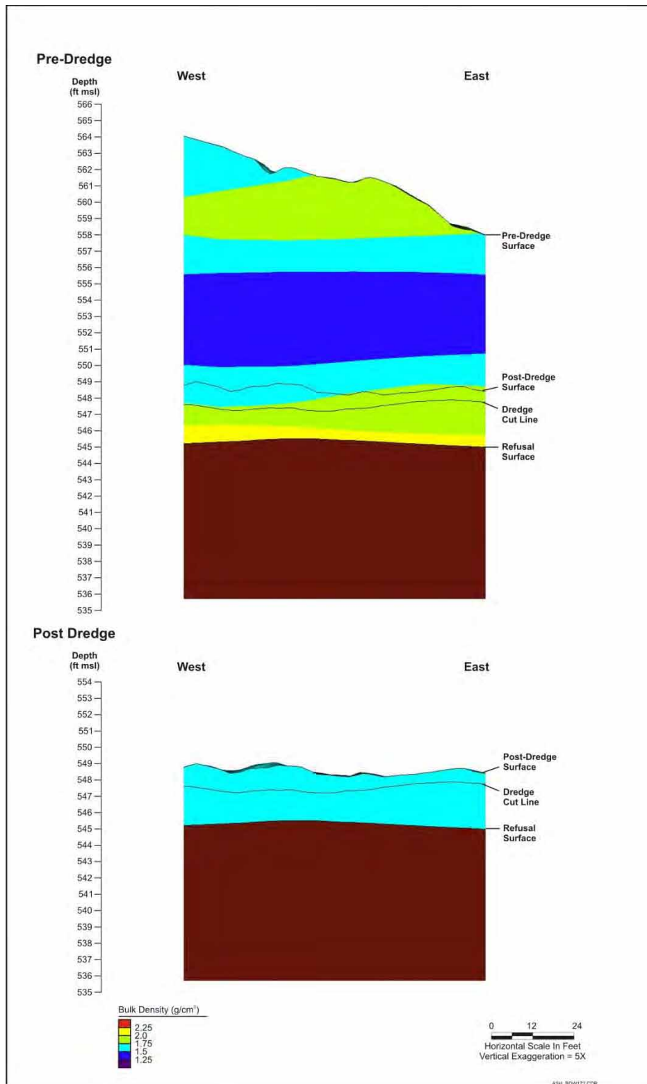
Figure 3-4. Comparison of Pre- and Post-Dredge Dry Bulk Densities in Sediment at T172
