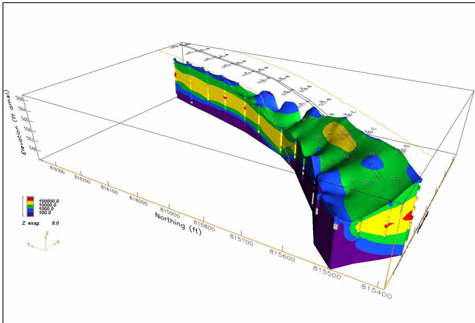
Figure 3-5. Pre-Dredge Sediment t-PCB Concentration Profiles in the Study Area (> 0 ppb)
