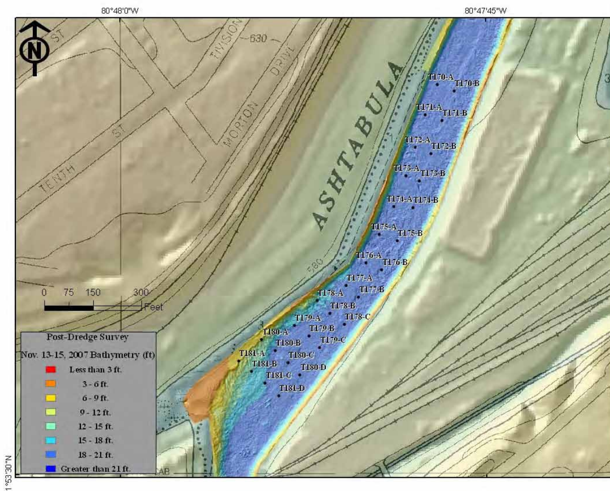
Figure 3-26. Post-Dredge Bathymetric Survey Results of the Study Area
