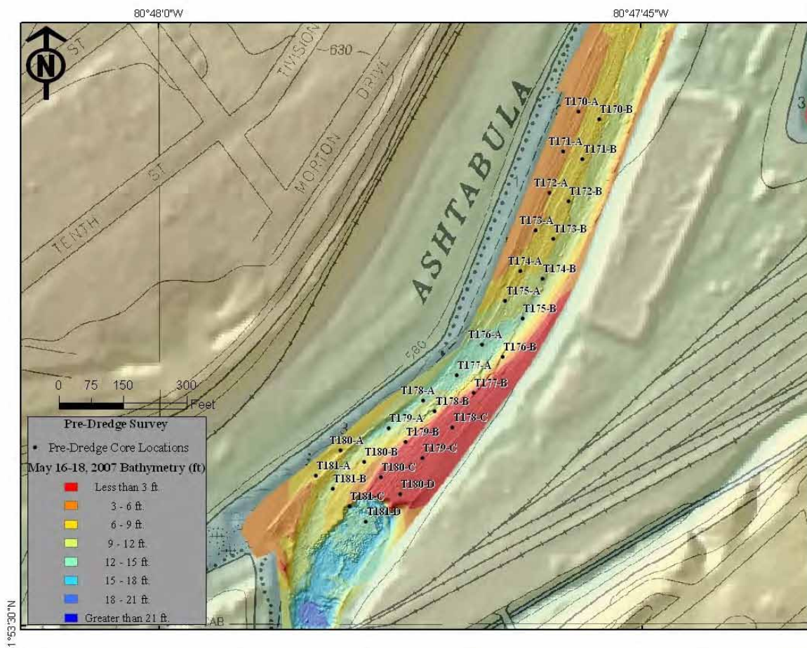
Figure 3-25. Pre-Dredge Bathymetric Survey Results for the Study Area
