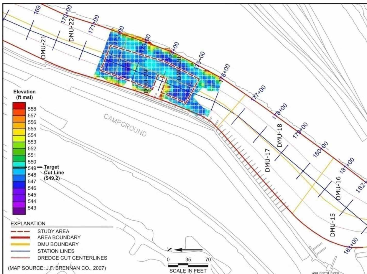
Figure 3-33. Estimated Dredge Cut Line in Between T176 and 172 in the Study Area
