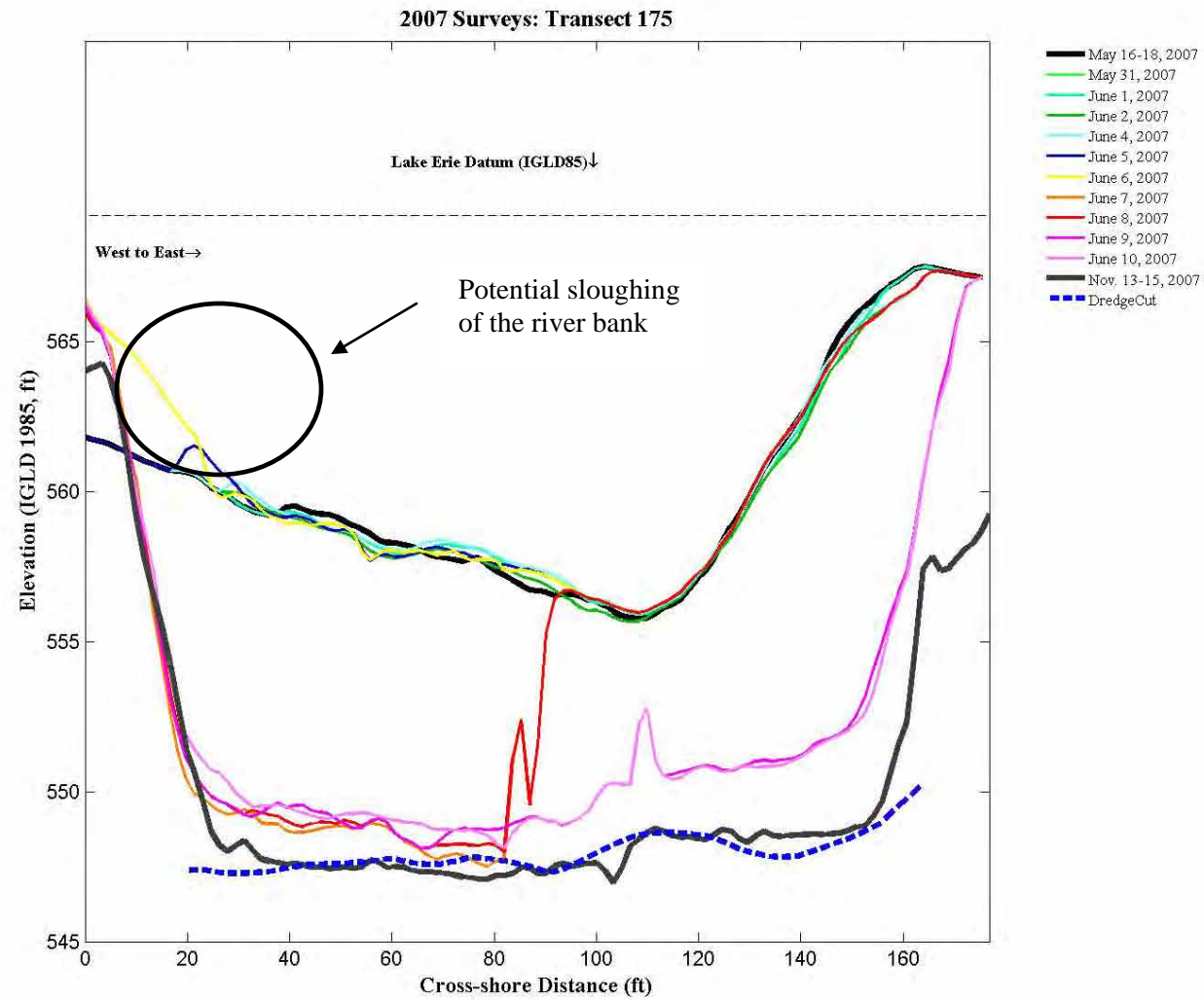
Figure 3-27. Cross-Section View at T175 Showing the Change in Bathymetry During Dredging
