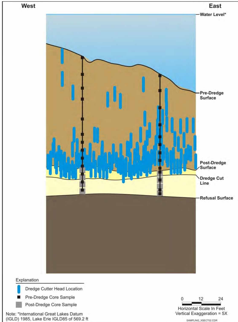
Figure 3-31. Conceptual Model River Cross-Section Showing the XYZ Dredge Cutter-Head Position and Approximated Cut Line
