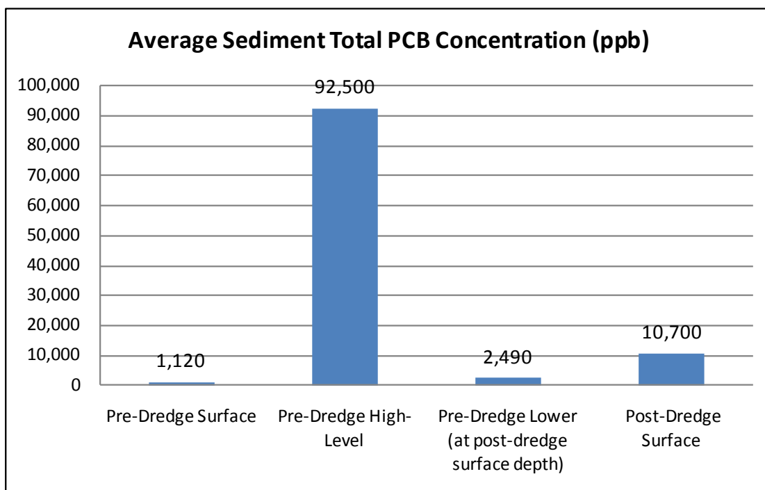
Figure 3-13. Average t-PCB Concentrations in Pre-Dredge Surface, High-Level, and Lower Sediments and Post-Dredge Surface Sediments. Pre-Dredge Lower Sediments are from the Same Elevations as Post-Dredge Surface Sediments. Based on Data in Table 3-2.
