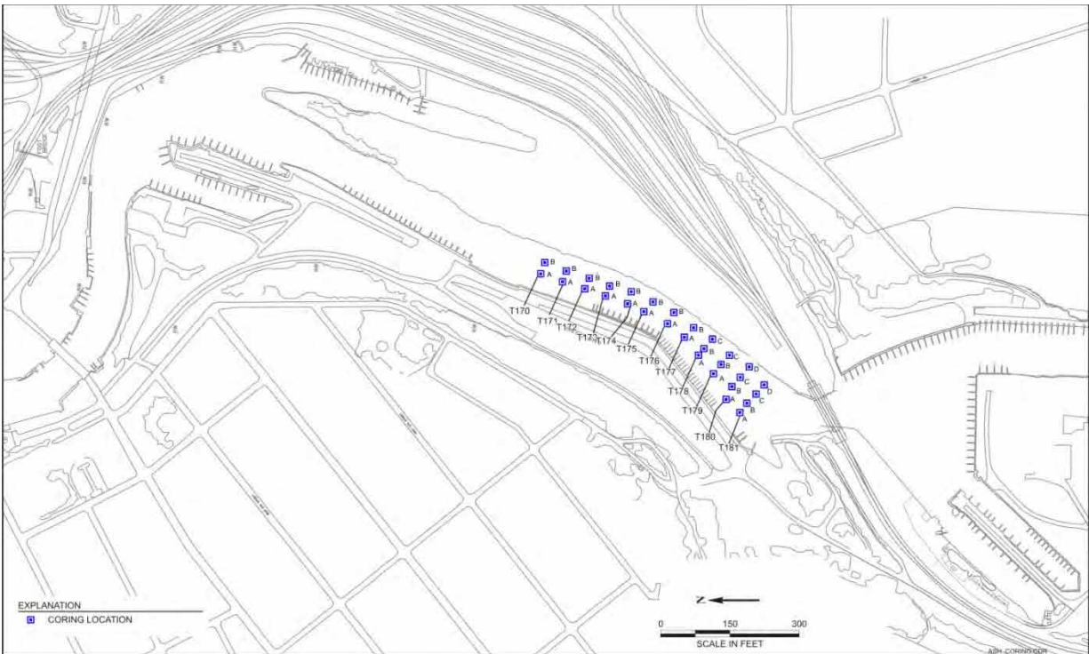
Figure 2-2. Sediment Core Sample Locations in the Ashtabula River Study Area for Phase 1 and 3 (Pre- and Post-Dredging, respectively)
