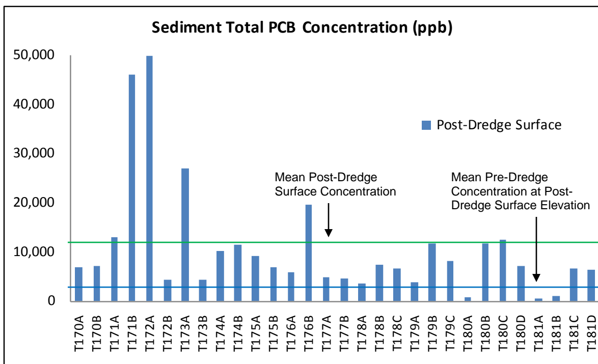
Figure 3-15. The Total PCB Concentration in the Post-Dredge Surface Sediments at the Sediment Coring Locations Presented in Table 3-2. The Mean Concentration is Also Presented along with the Mean Pre-Dredge Concentration from the Same Elevation.
