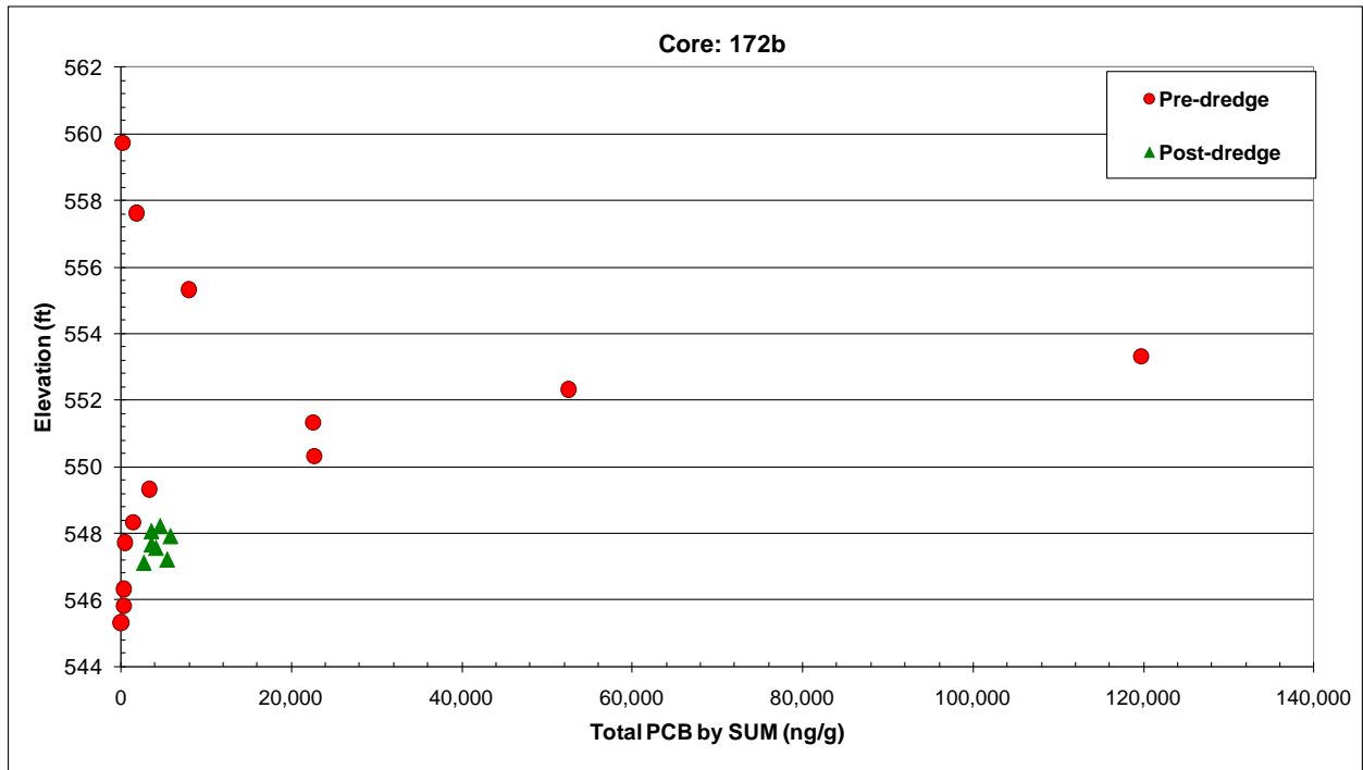
Figure 3-16. Total PCB Concentrations in Pre- and Post-Dredge Core Samples from Locations T170B and T172B
