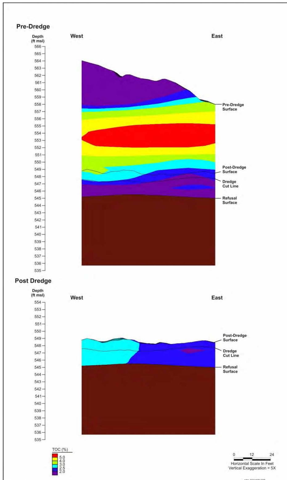
Figure 3-3. Comparison of Pre- and Post-Dredge TOC Concentrations in Sediment at T172
