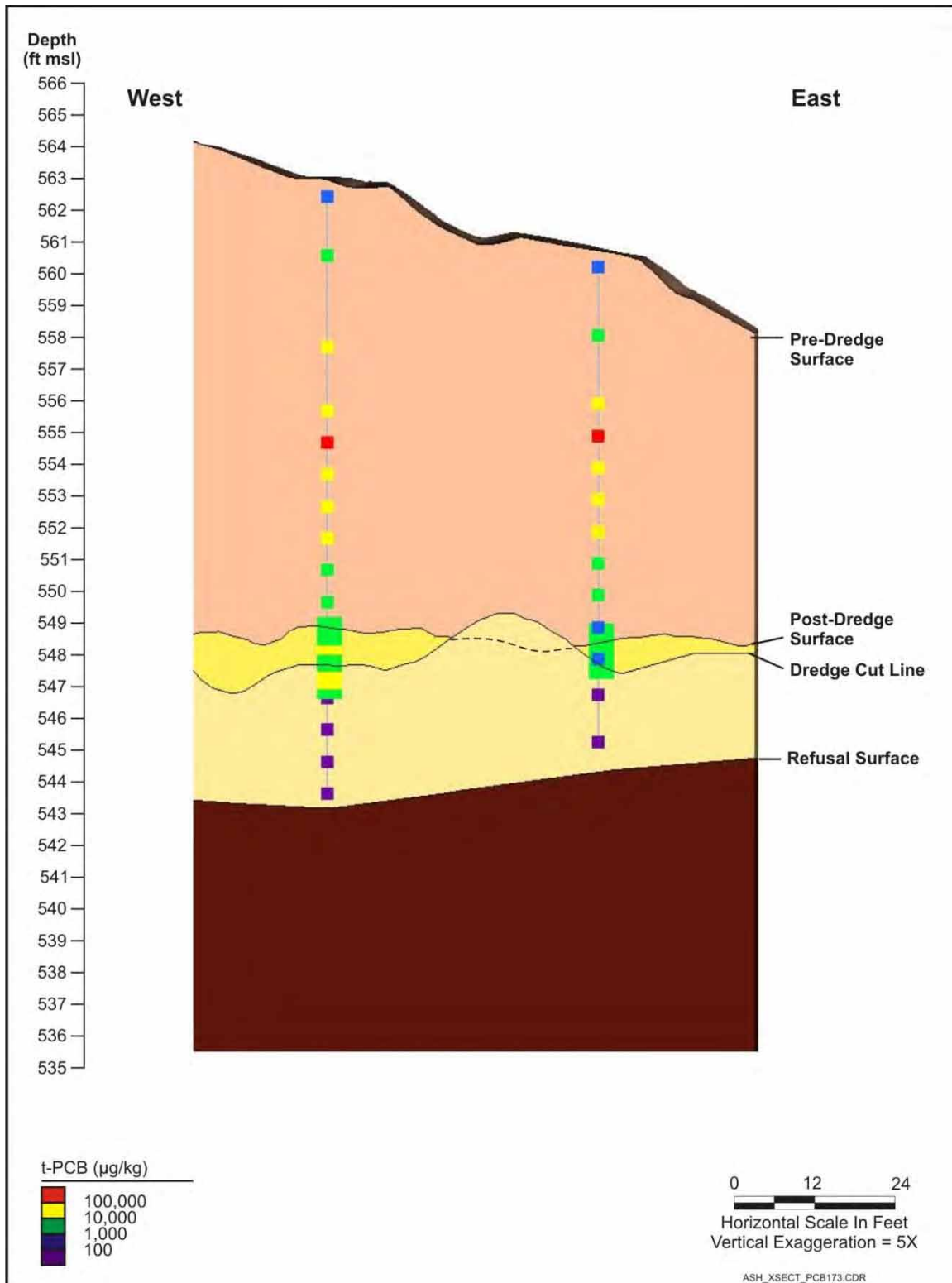
Figure 3-36. Cross-Section of T173 Showing Estimated Dredge Cut Line vs. Post-Dredge Bathymetry
