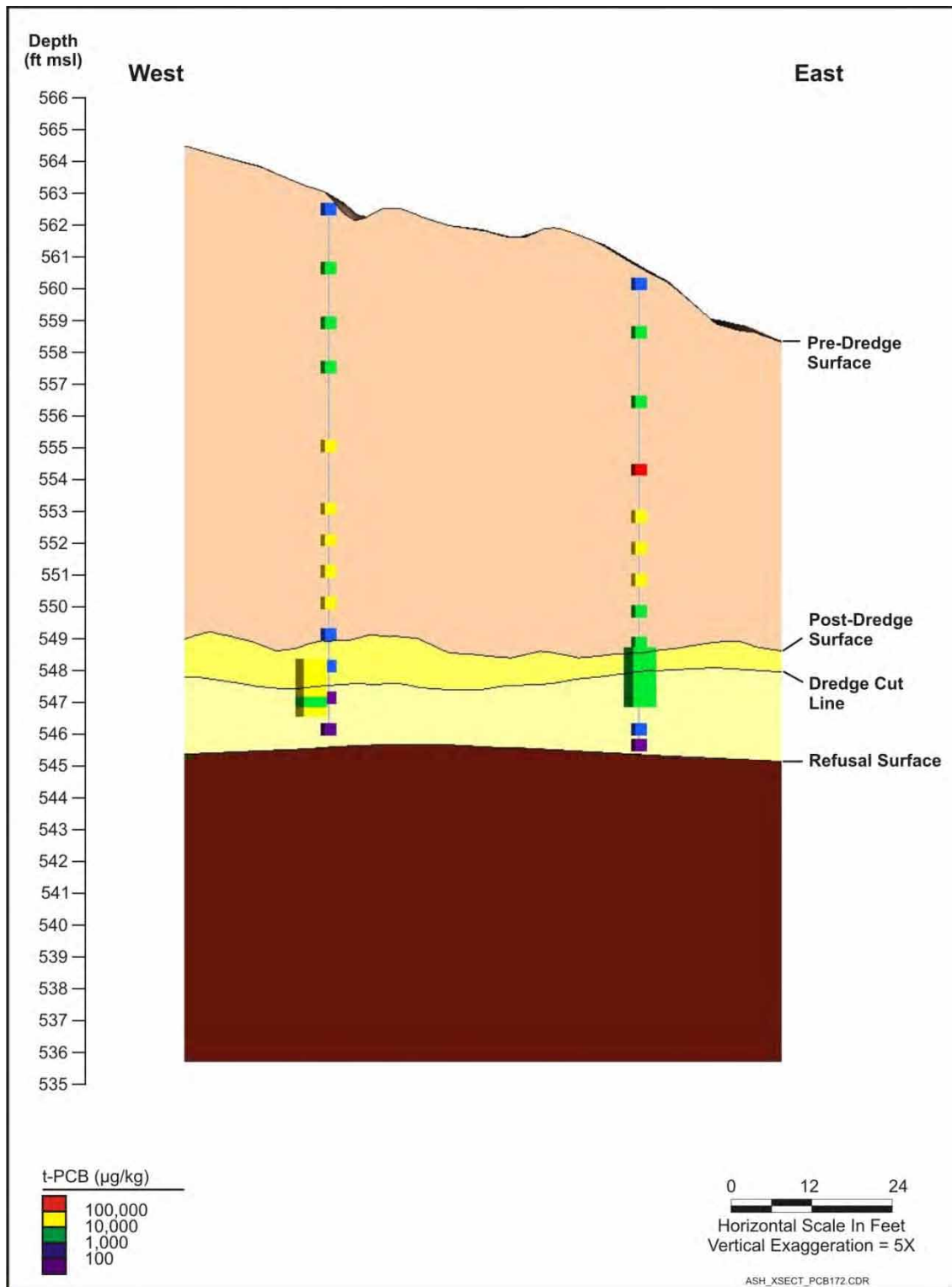
Figure 3-37. Cross-Section of T172 Showing Estimated Dredge Cut Line vs. Post-Dredge Bathymetry
