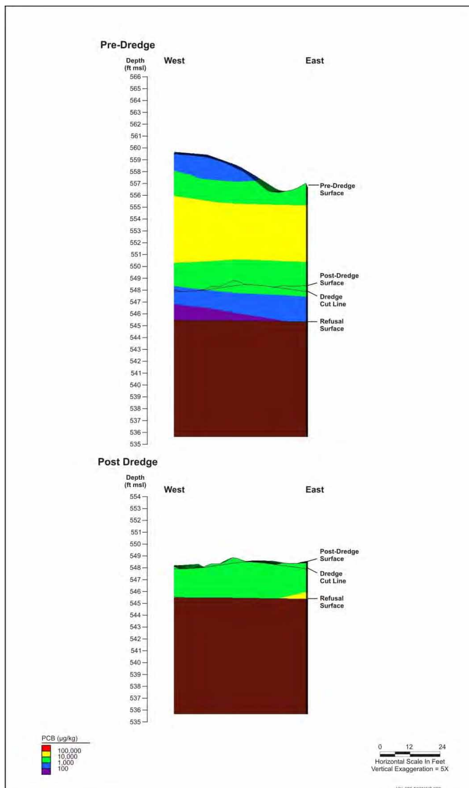
Figure 3-22. Comparison of Pre- and Post-Dredge Cross-Section t-PCBs in Sediment at T174
