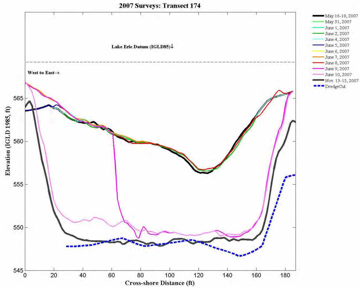
Figure 3-28. Cross-Section View at T174 Showing the Change in Bathymetry During Dredging
