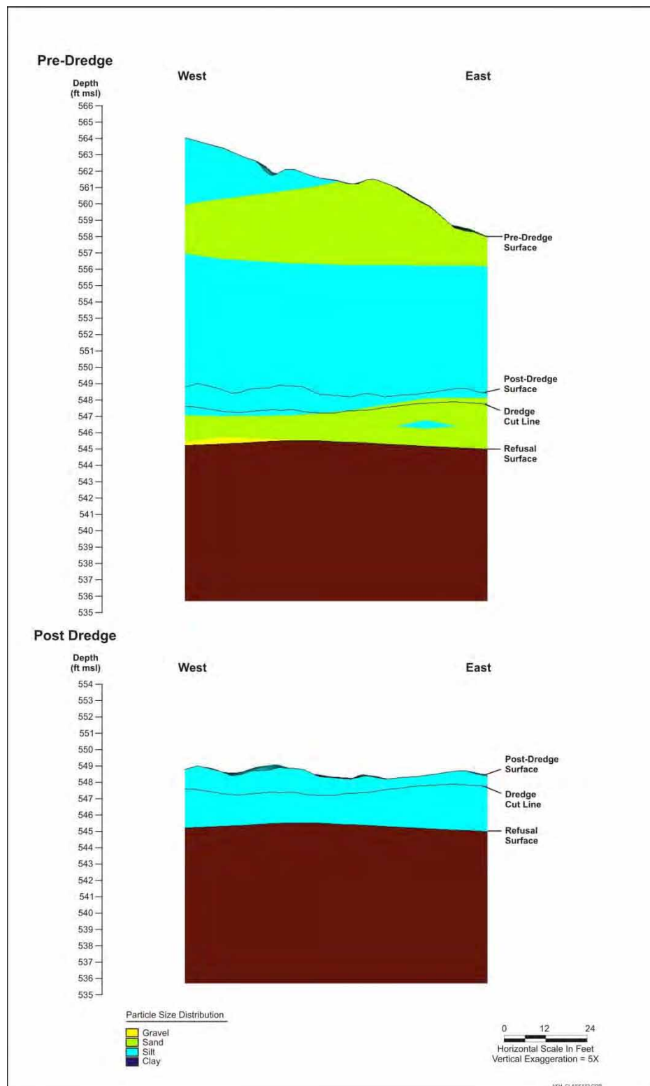
Figure 3-2. Comparison of Pre- and Post-Dredge Particle Size Distributions in Sediment at T172
