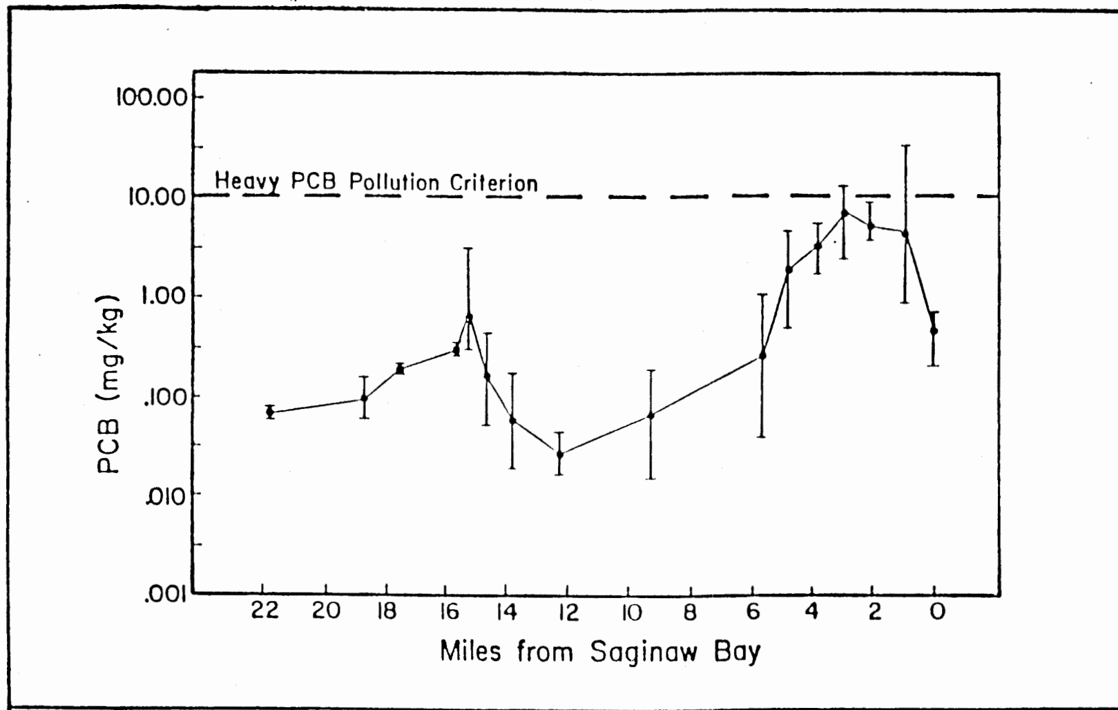
Figure III-62. PCB distribution in surficial sediments of the Saginaw River, transect means and ranges, 1980-1981 (LTI, 1983).
