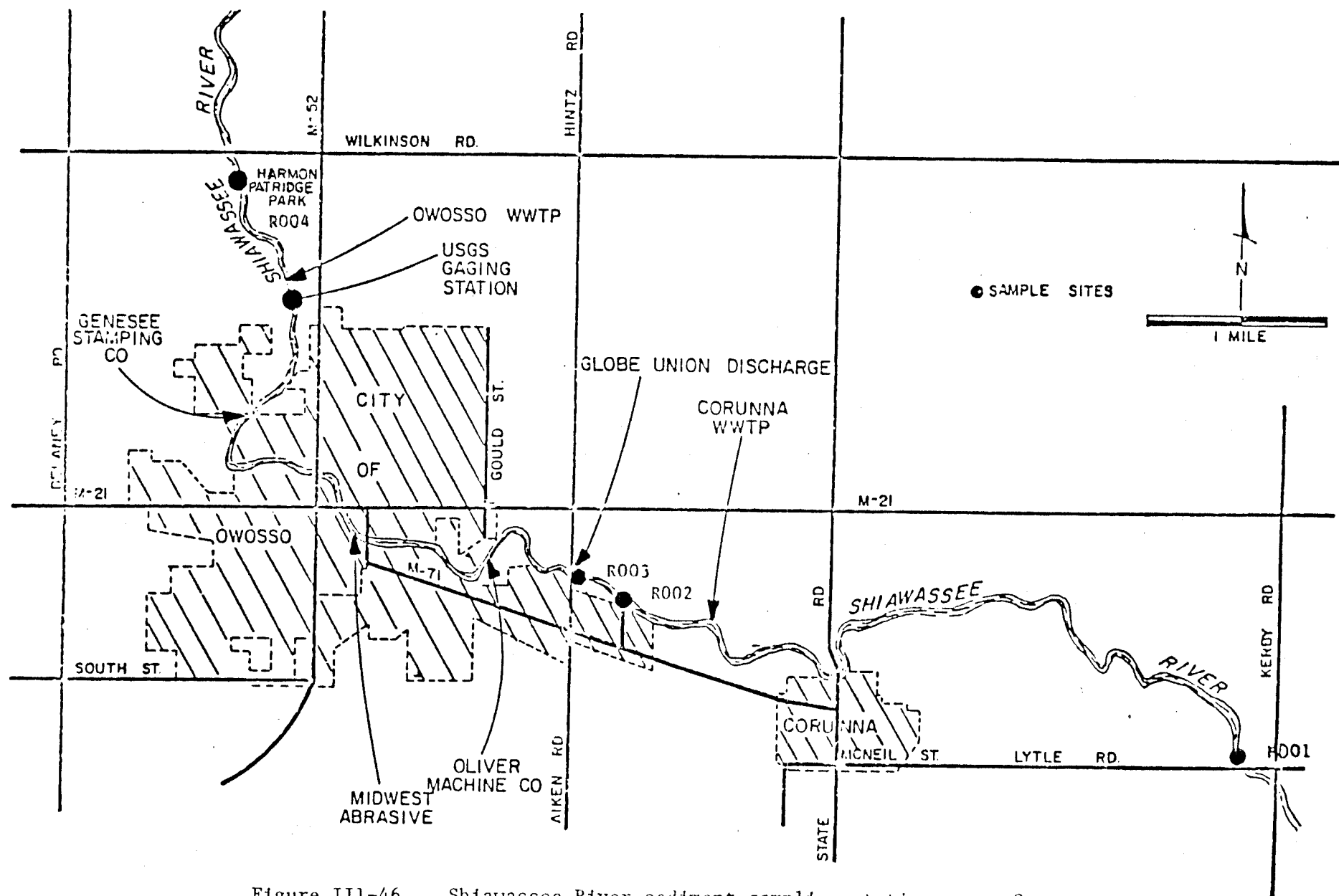
Figure III-46. Shiawassee River sediment sampling stations near Owosso, 1980 (MDNR, 1980).
