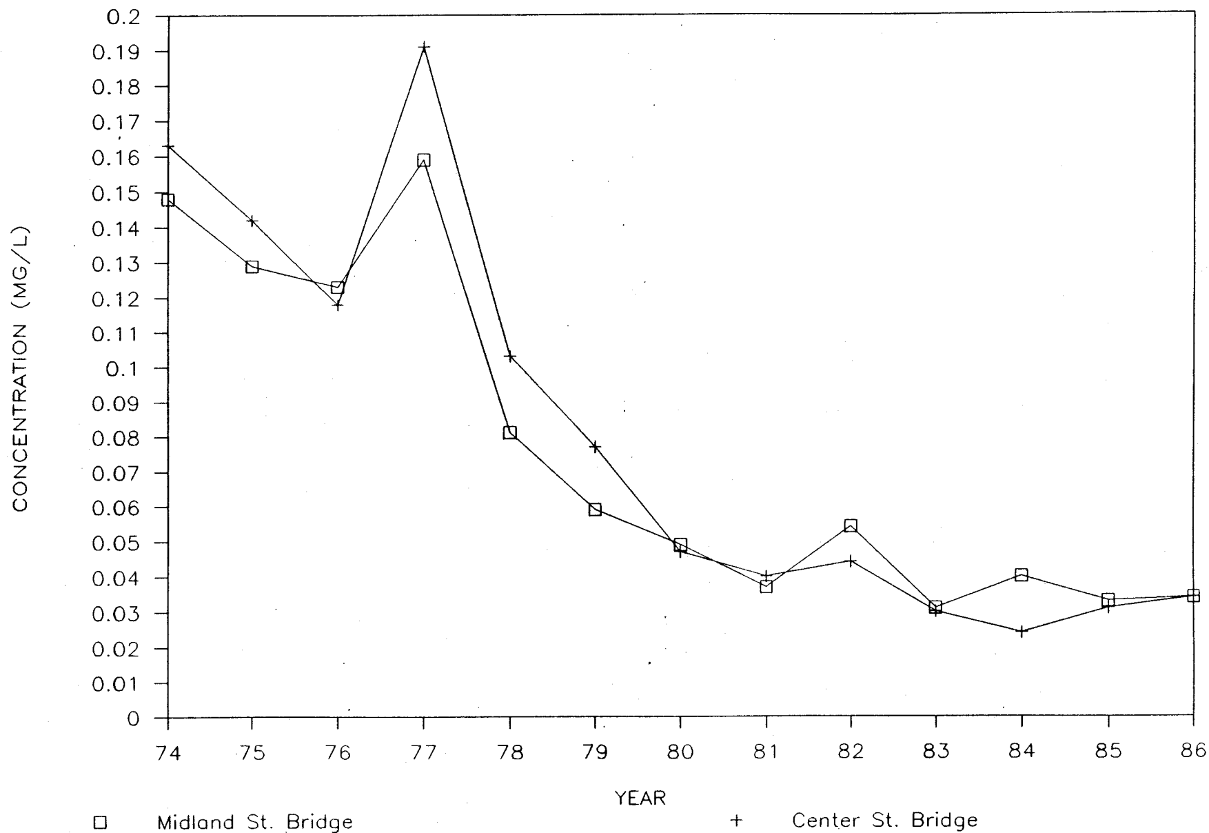
Figure III-22. Annual average orthophosphorus concentrations in Saginaw River water samples, 1974-1986.
