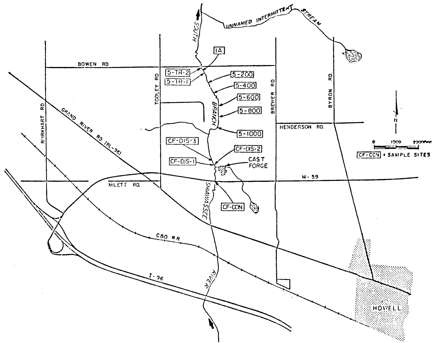
Figure III-42. South branch Shiawassee River sediment survey sampling locations, August, 1977 (MDNR, 1977).
