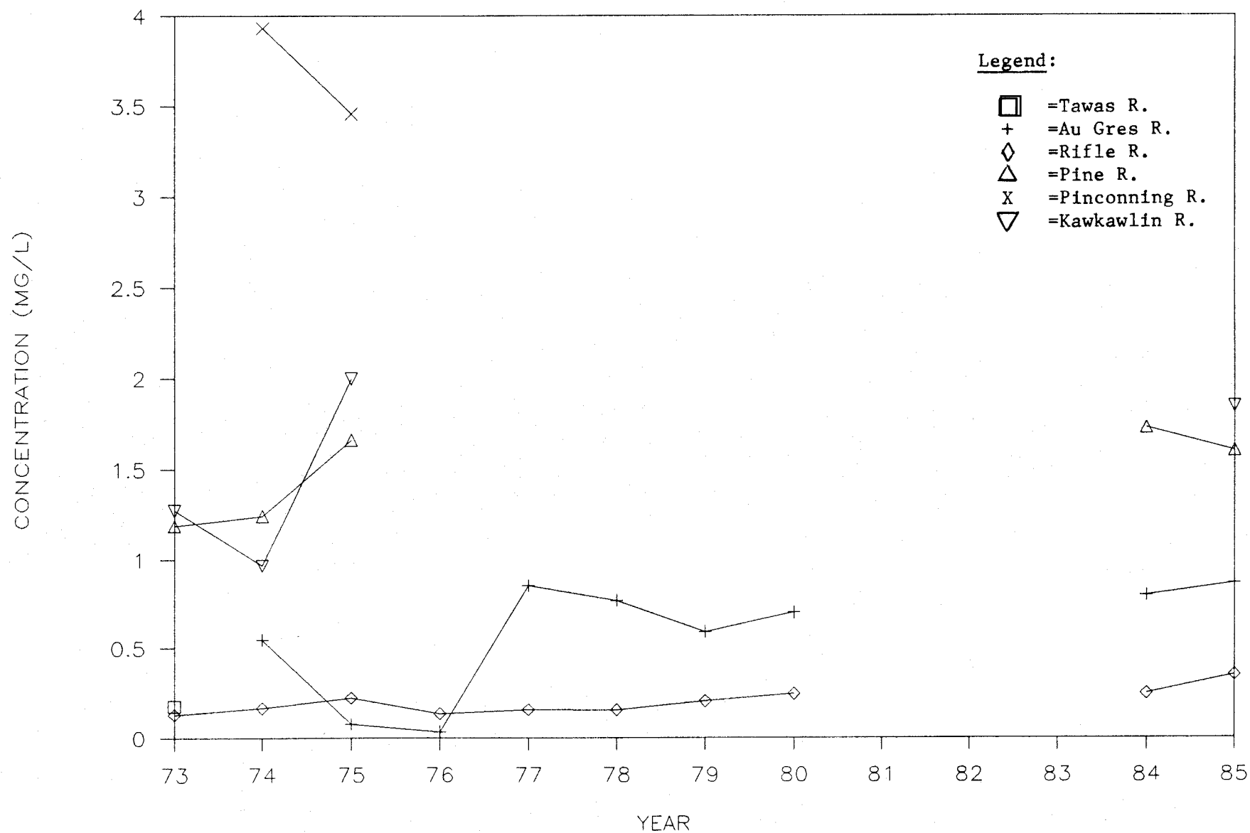
Figure III-33. Annual average nitrate-nitrite concentrations in Saginaw Bay west coastal basin tributaries, 1973-1985.
