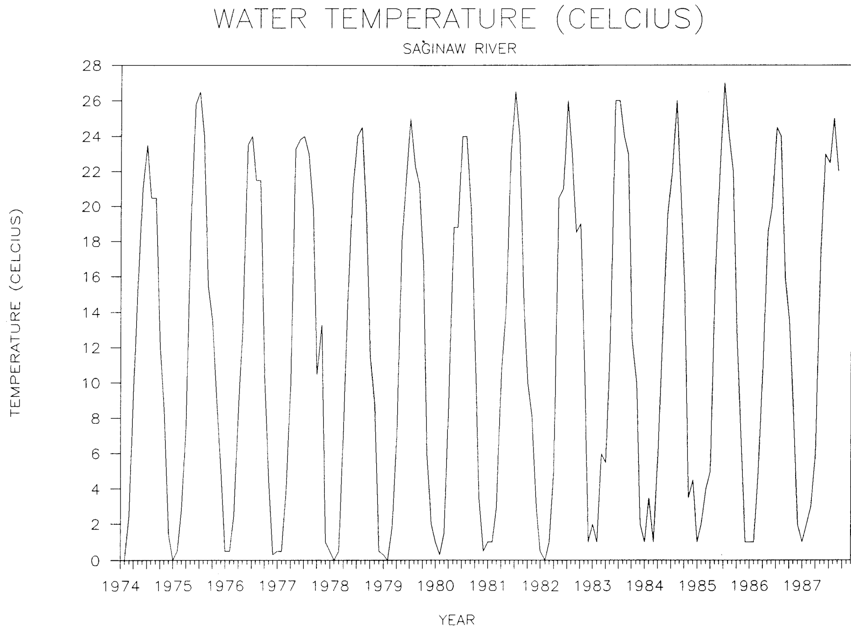
Figure III-3. Monthly water temperatures in the Saginaw River, 1974-1987.
