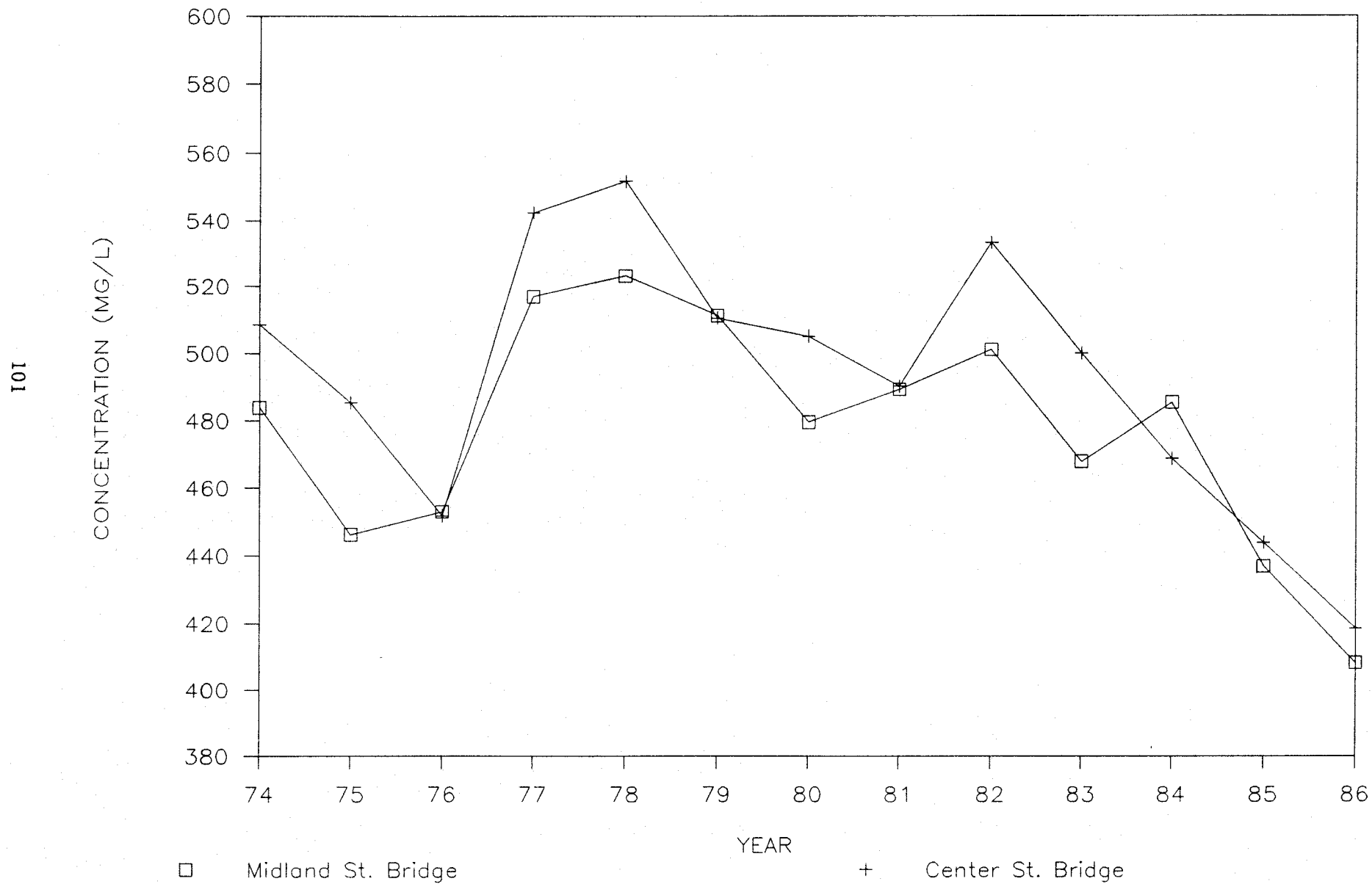
Figure III-17. Annual average total solids concentrations in Saginaw River water samples, 1974-1986.
