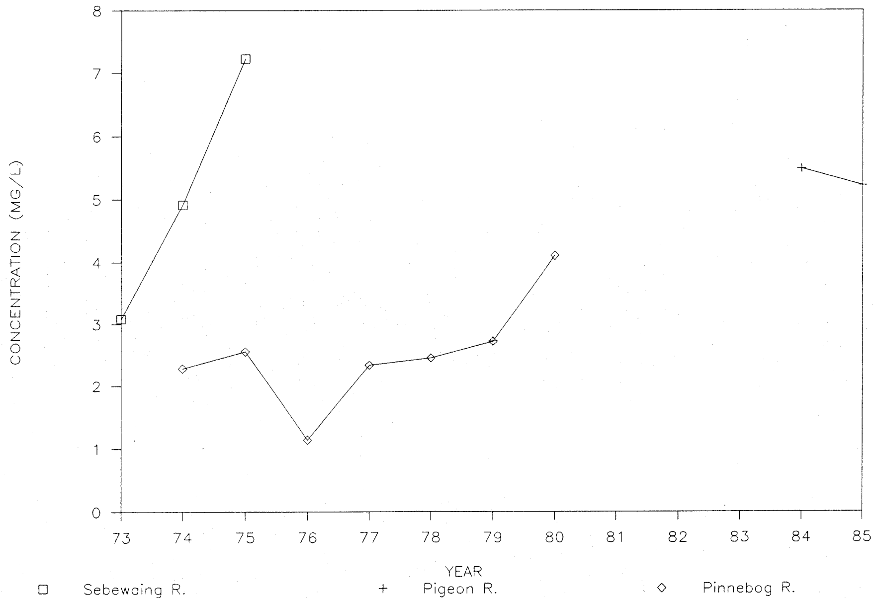
Figure III-34. Annual average nitrate-nitrite concentrations in Saginaw Bay east coastal basin tributaries, 1973-1985.
