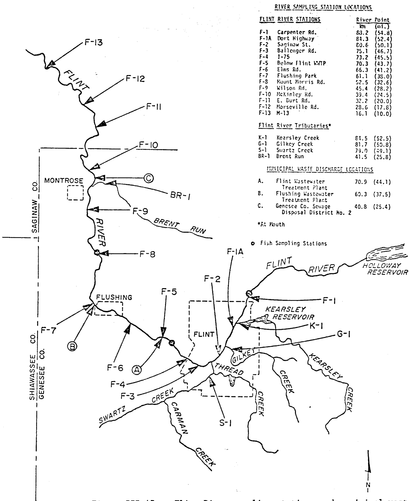
Figure III-47. Flint River sampling stations and municipal waste discharges, 1974.
