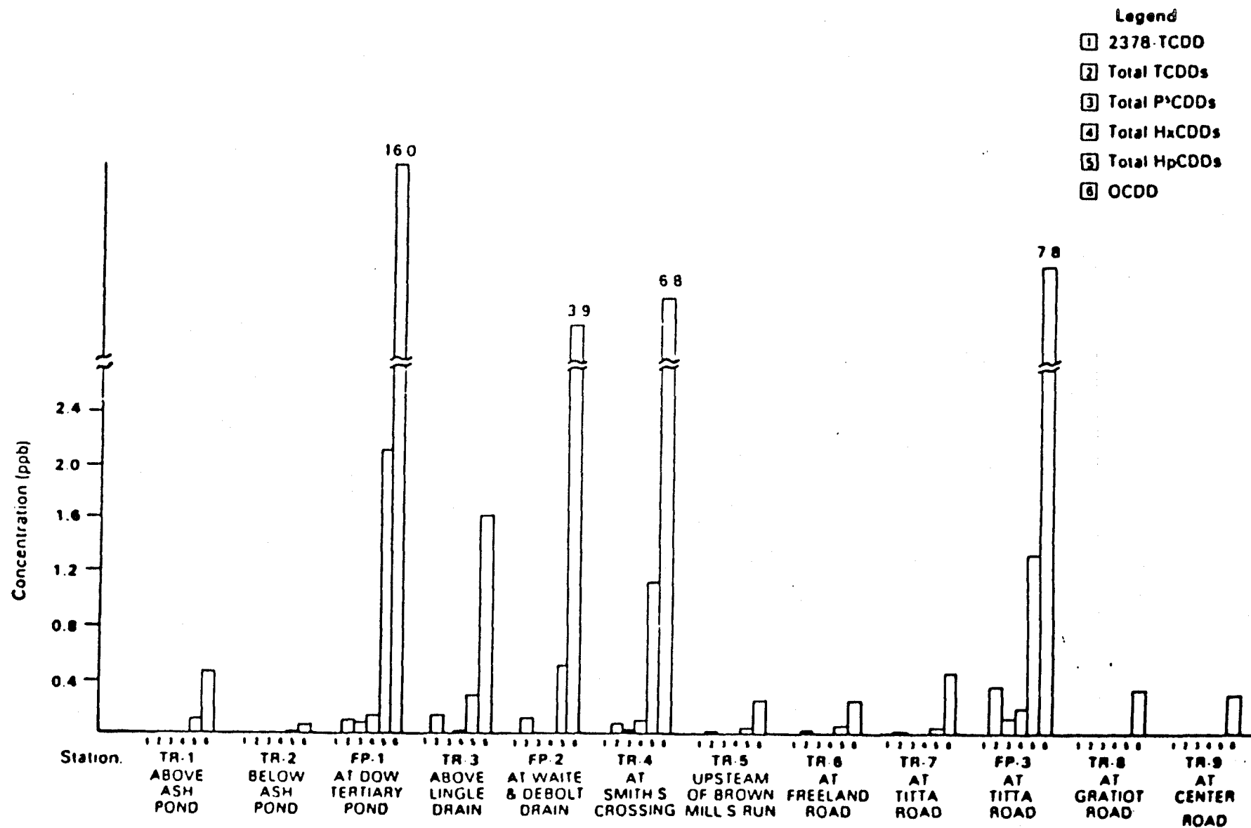
Figure III-51. PCDDs (ug/kg) in Tittabawasee River sediment and flood plain samples, July 1984 (USEPA, 1986).
