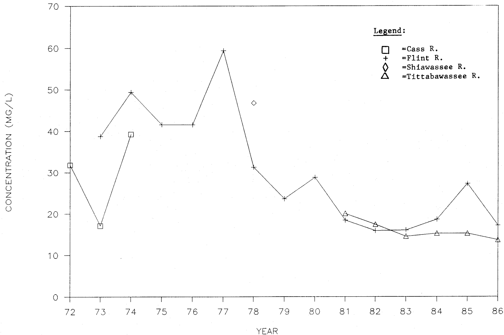
Figure III-14. Annual average suspended solids concentrations in Saginaw River tributaries, 1972-1986.
