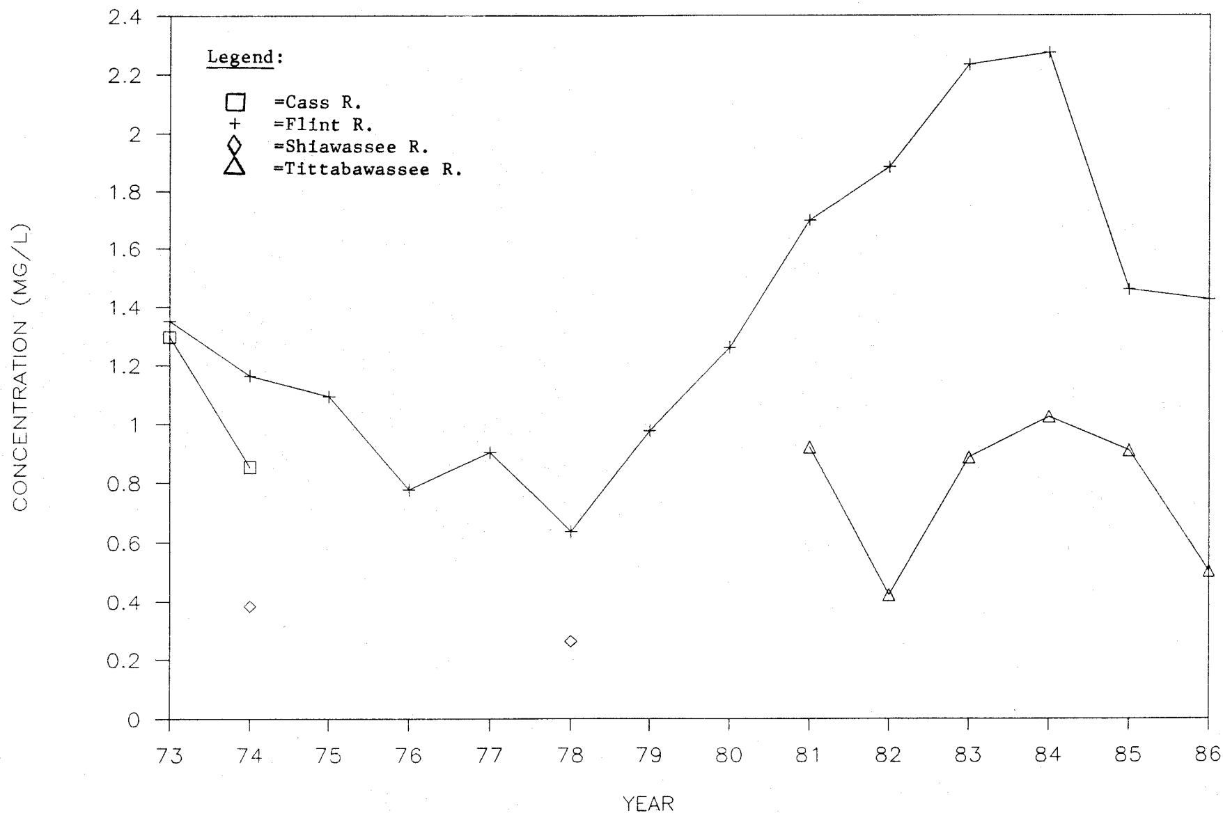
Figure III-32. Annual average nitrate-nitrite concentrations in Saginaw River tributaries, 1973-1986.
