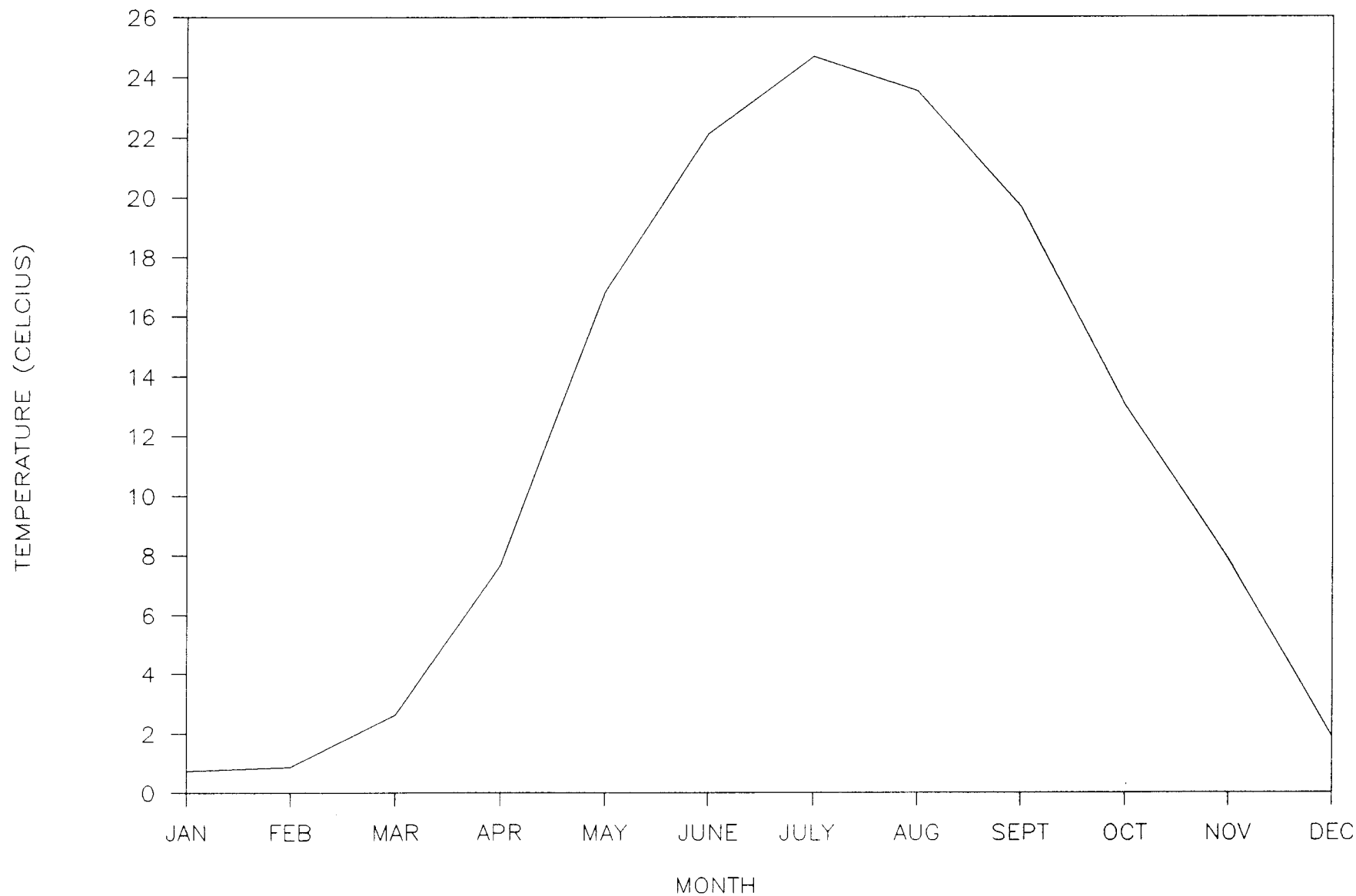
Figure III-2. Average monthly water temperatures in the Saginaw River, 1974-1987.
