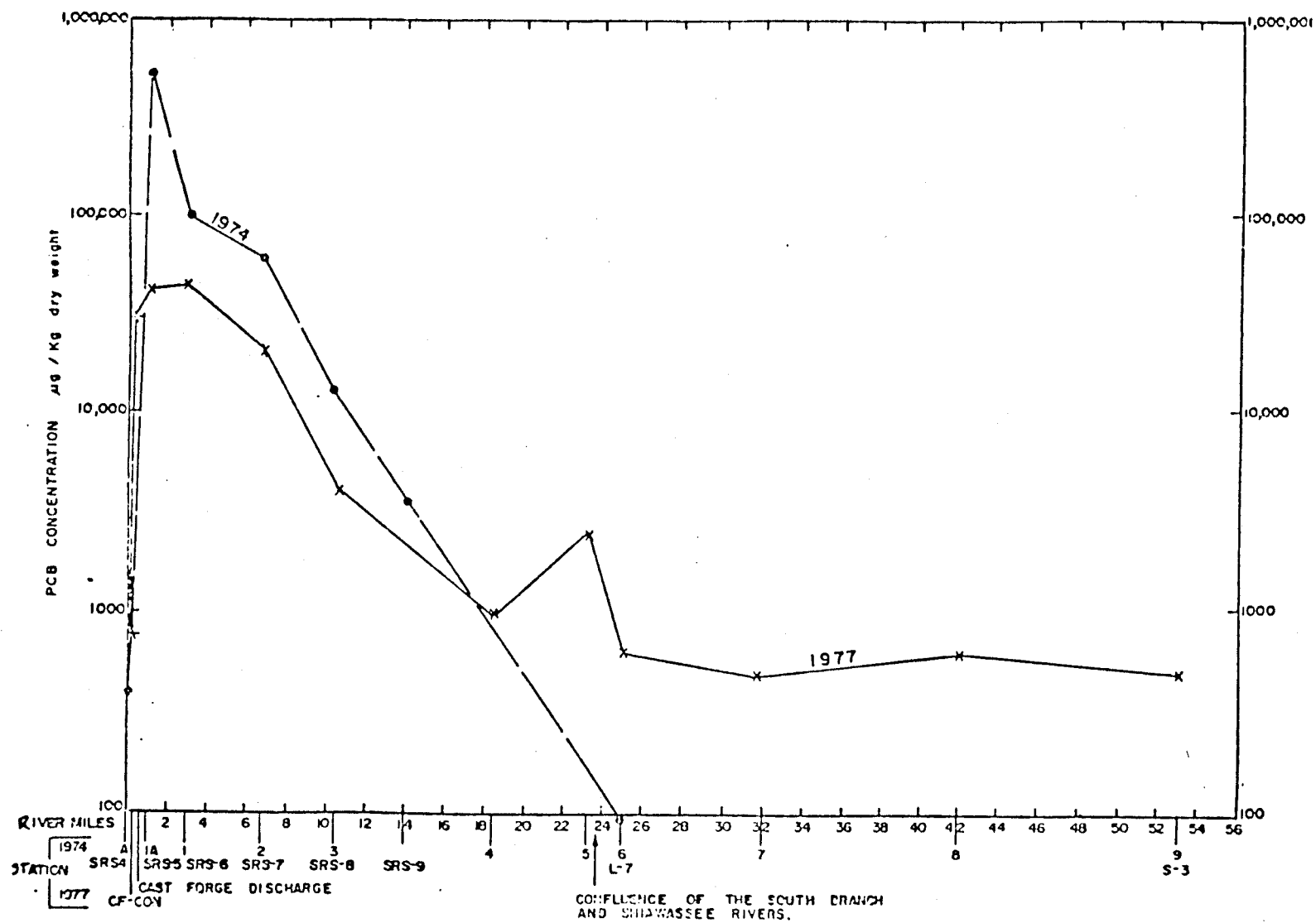
Figure III-44. 1974 and 1977 sediment PCB data for the south branch Shiawassee River below Howell to Corunna (MDNR, 1977).
