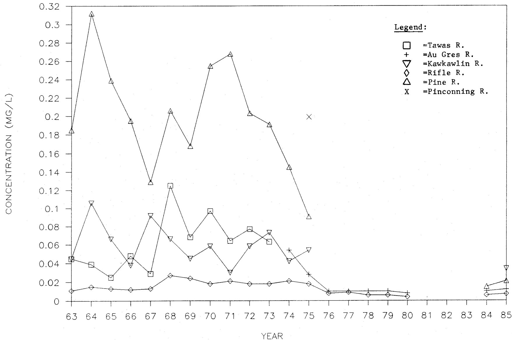
Figure III-26. Annual average orthophosphorus concentrations in Saginaw Bay west coastal basin tributaries, 1963-1985.
