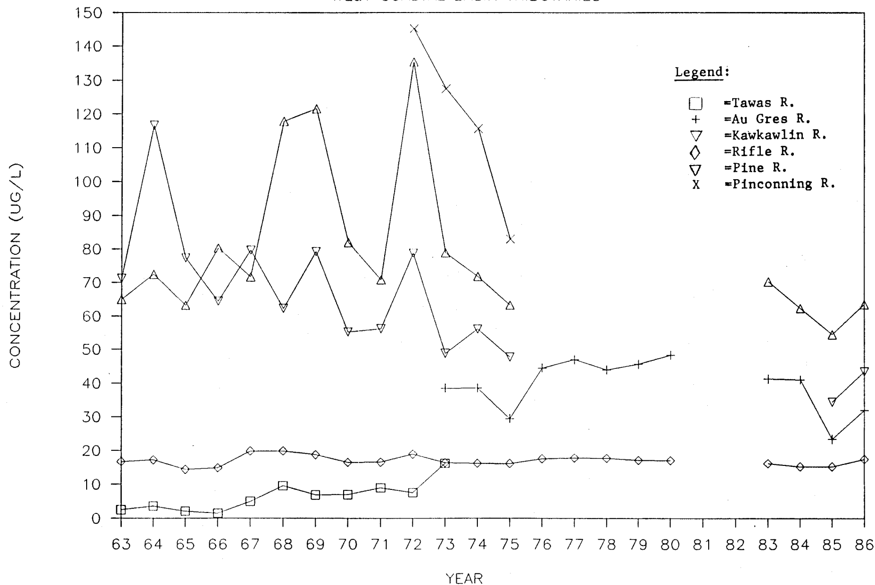
Figure III-38. Annual average chloride concentrations in Saginaw Bay west coastal basin tributaries, 1963-1986.
