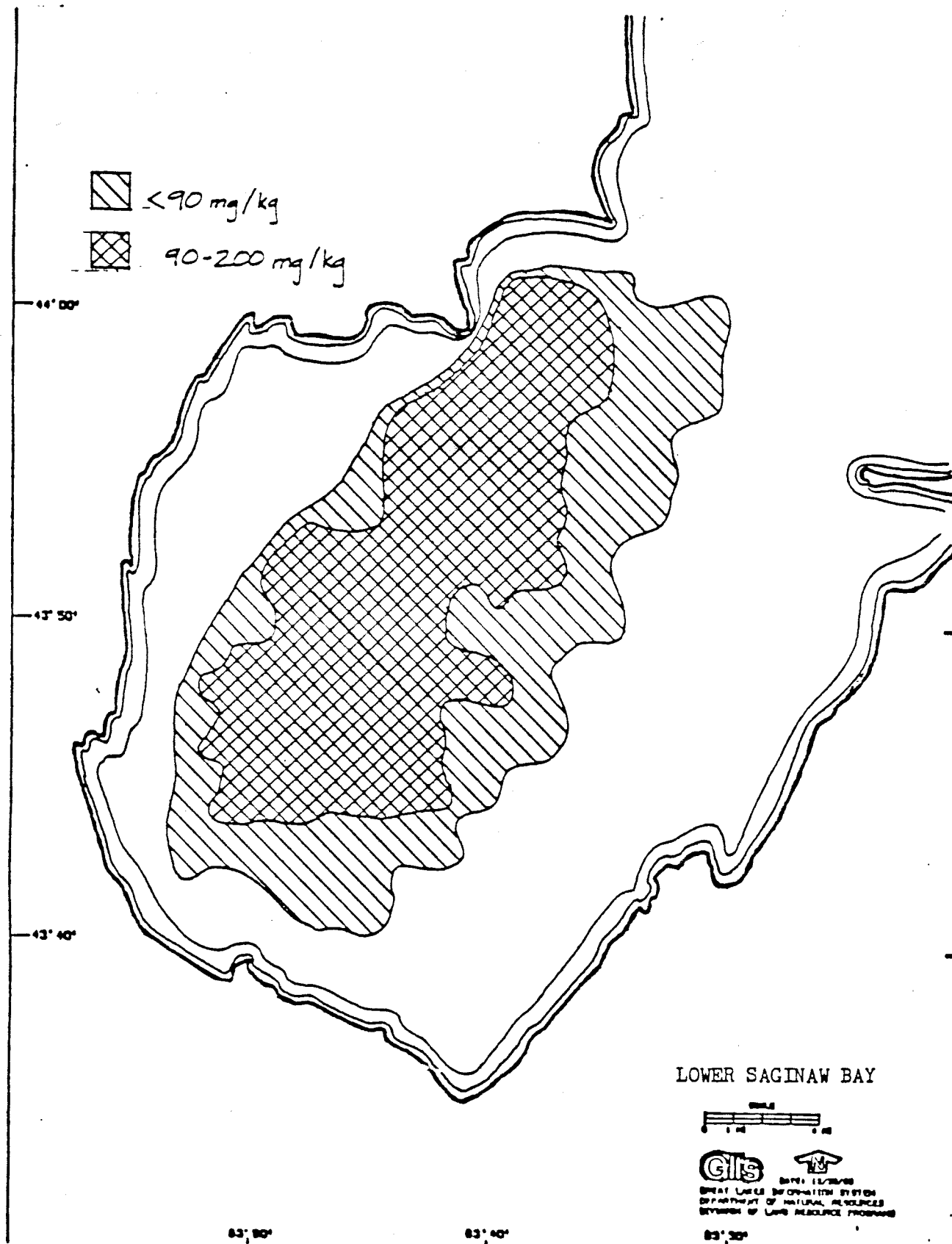
Figure III-84. Spatial distribution of zinc in surface sediments (1-2 cm) of inner Saginaw Bay, 1978 (Robbins, 1986).
