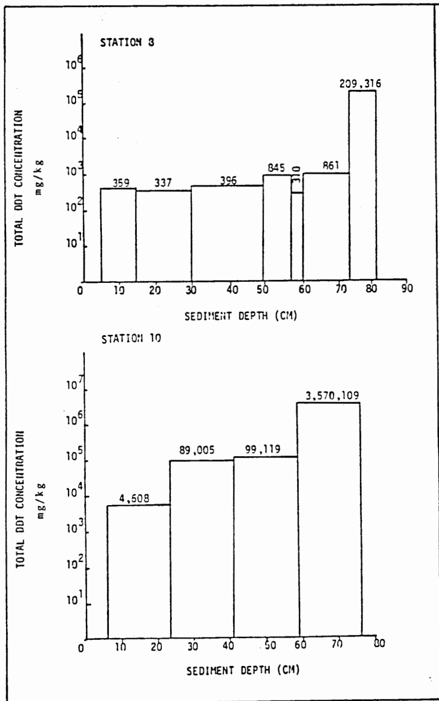
Figure III-58. Vertical DDT distribution, plotted on a log scale, in St. Louis Reservoir sediments offshore of the Michigan Chemical Corporation (ECMPDR, 1983).
