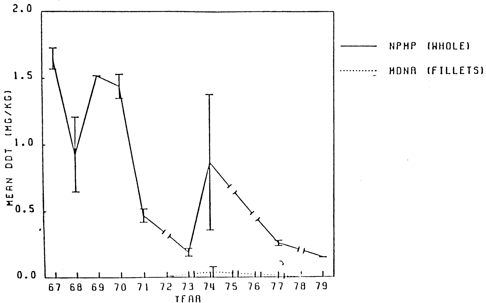
Figure III-103. Yearly mean DDT-R concentrations for yellow perch from Saginaw Bay, 1967-1979 (Kreis and Rice, 1985).
