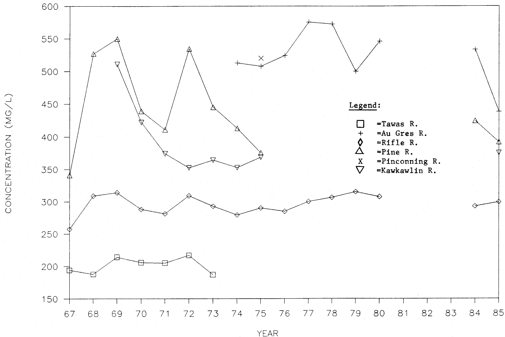
Figure III-19. Annual average total solids concentrations in Saginaw Bay west coastal basin tributaries, 1967-1985.
