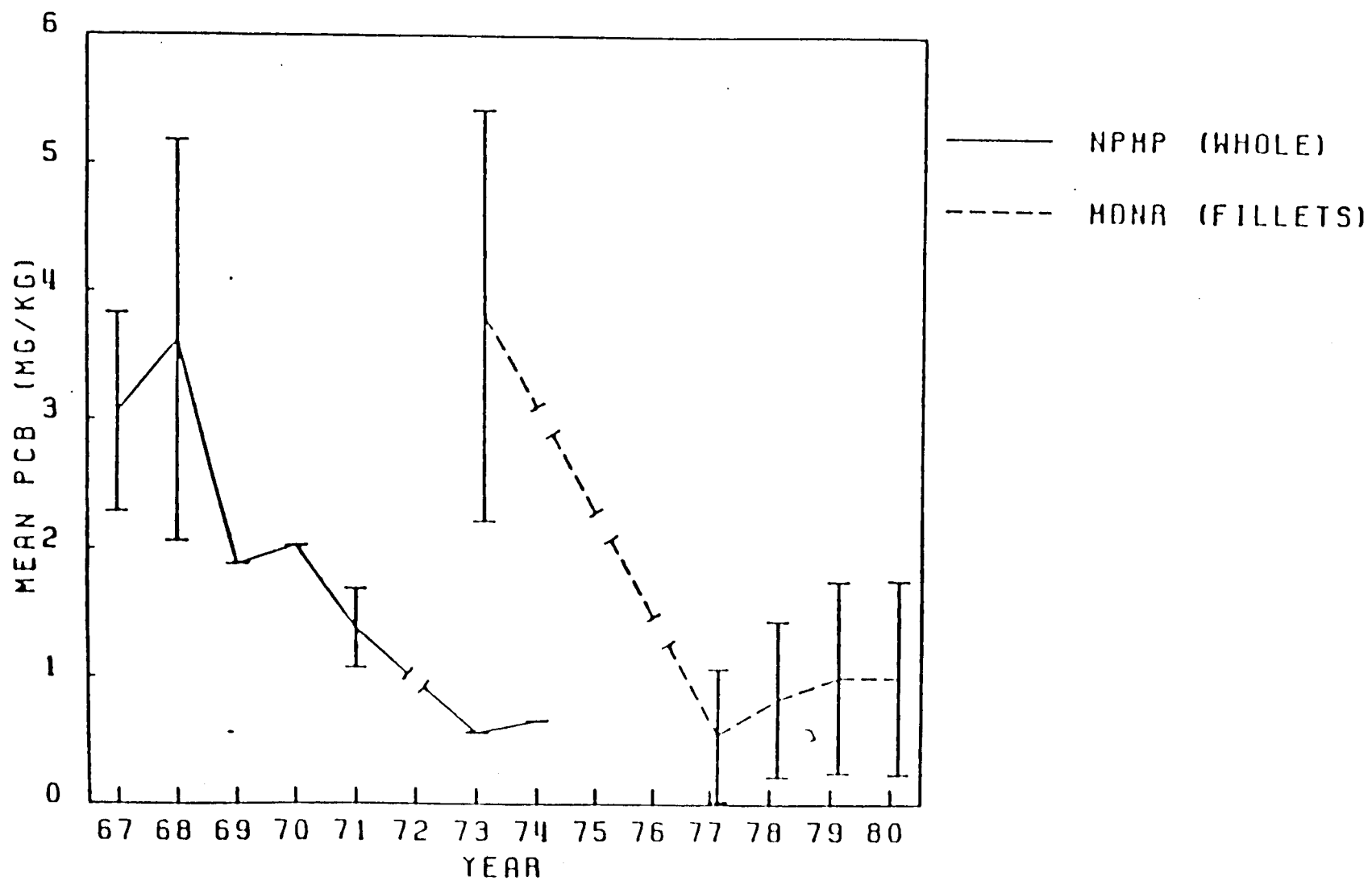
Figure III-102. Yearly mean DDT-R concentrations for channel catfish from Saginaw Bay, 1967-1980 (Kreiss and Rice, 1985).
