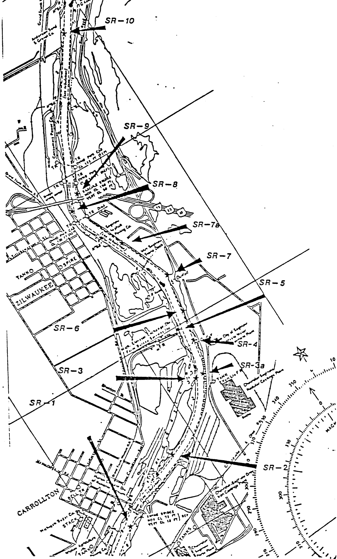
Figure III-65. Saginaw River sediment sampling stations, near the City of Saginaw, 1983 (USACOE, 1983).
