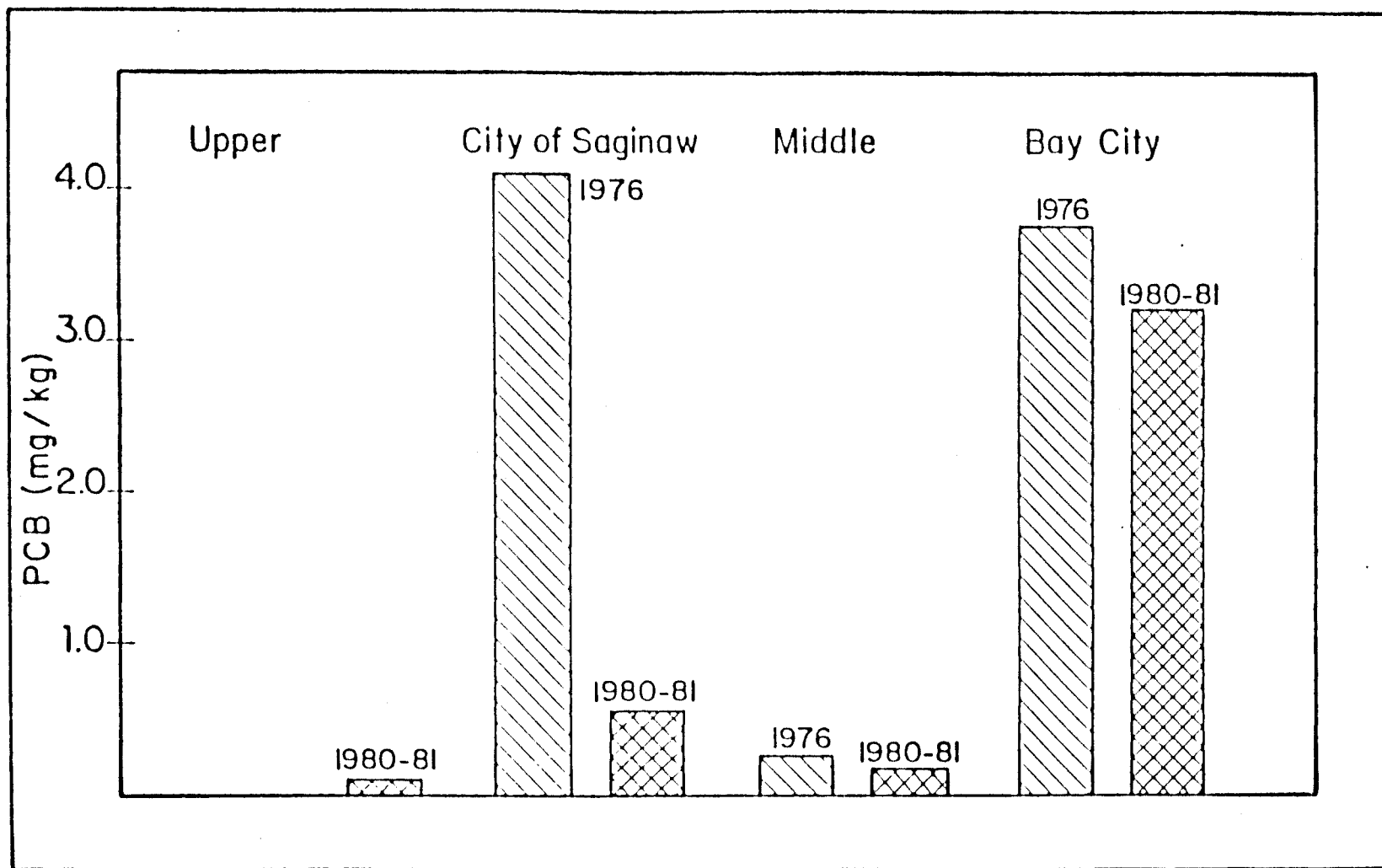
Figure III-64. Comparison of geometric mean PCB concentrations in surficial sediments of the Saginaw River navigation channel, 1976 USACOE survey and 1980-1981 (LTI, 1983).
