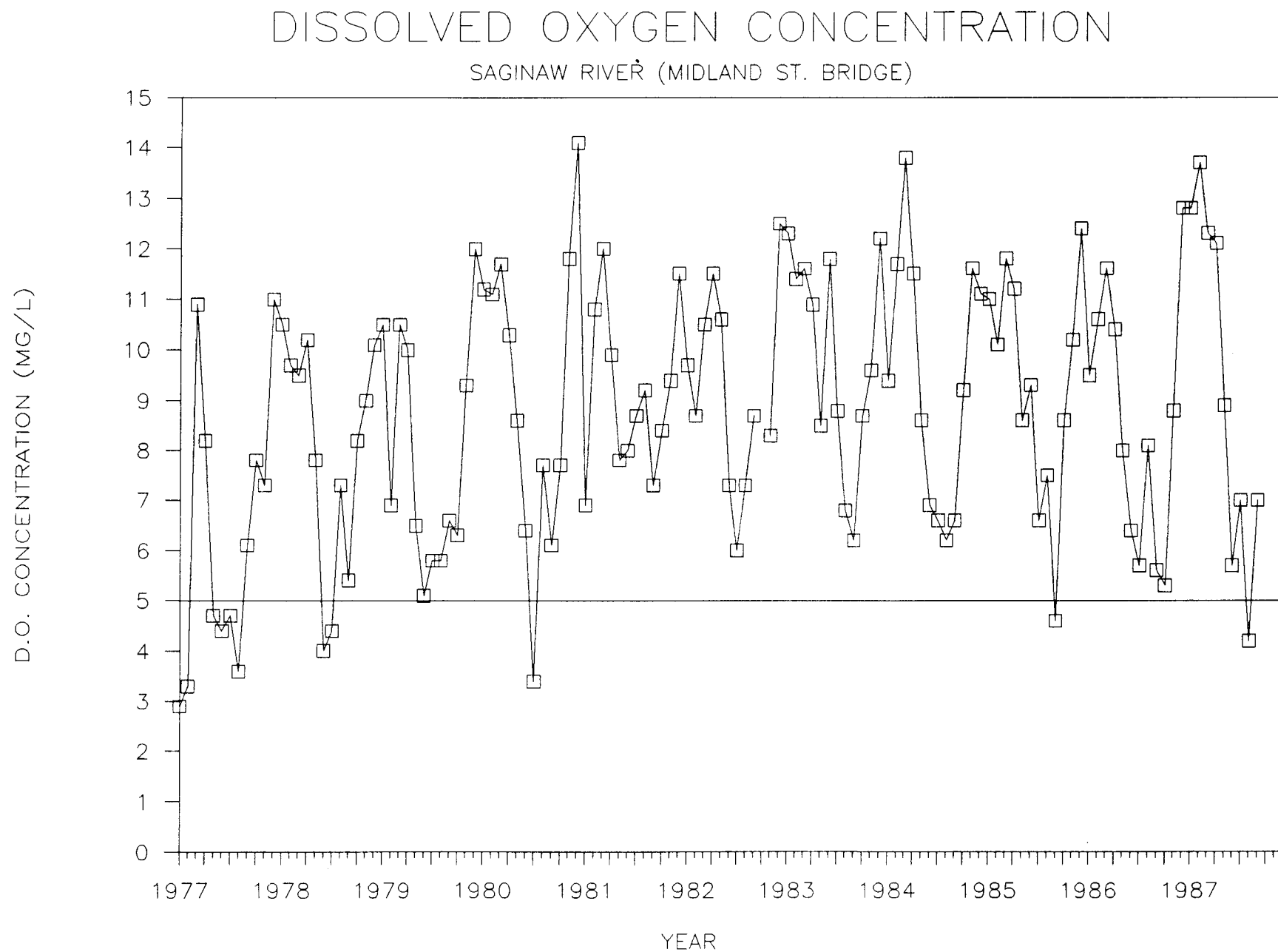
Figure III-4. Monthly dissolved oxygen concentrations in the Saginaw River at the Midland Street bridge, 1977-1987.
