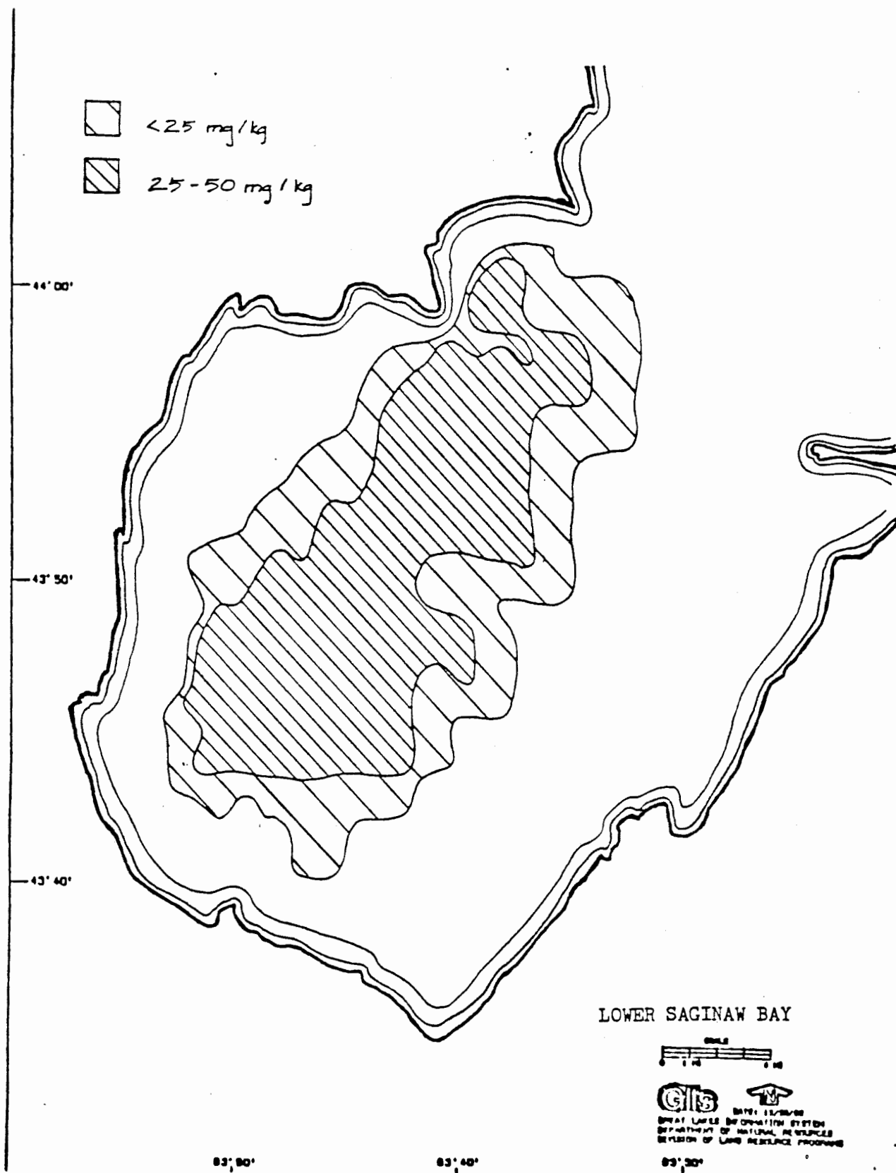
Figure III-81. Spatial distribution of copper in surface sediments (1-2 cm) of inner Saginaw Bay, 1978 (Robbins, 1986).
