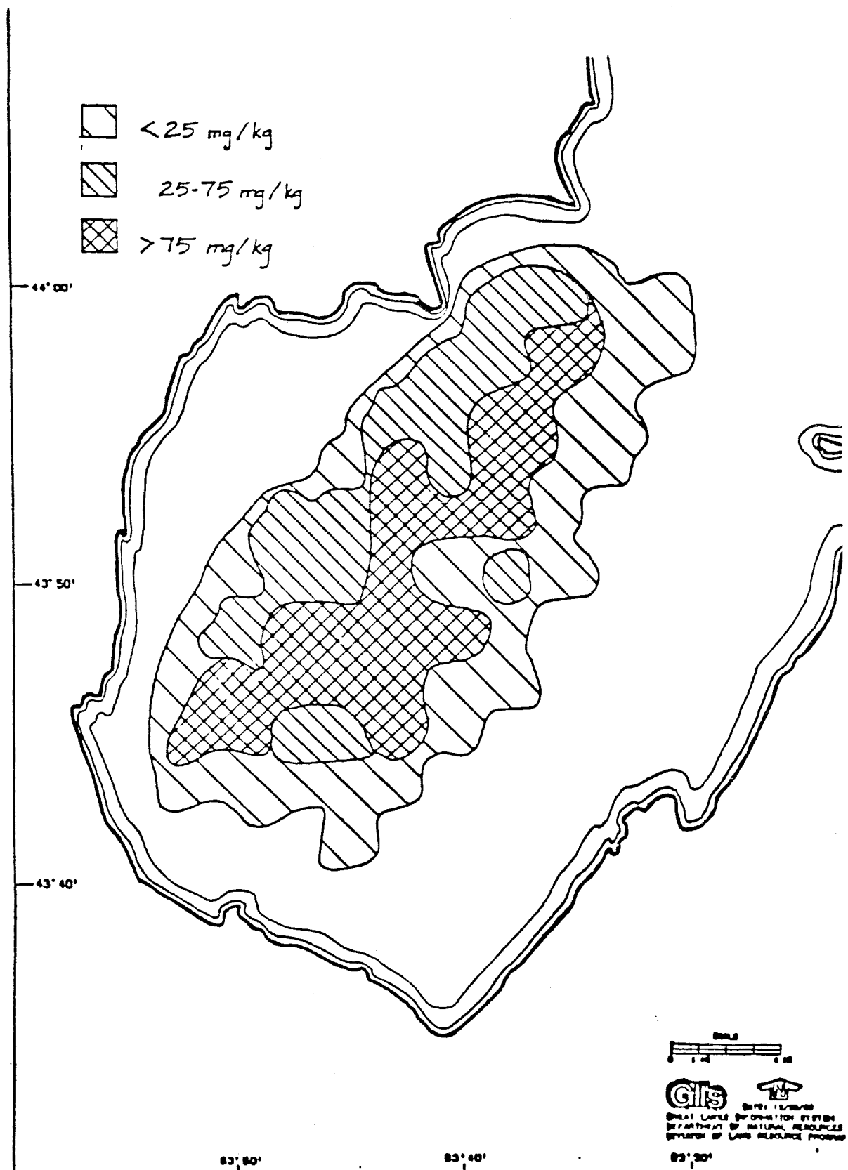
Figure III-80. Spatial distribution of chromium in surface sediments (1-2 cm) of inner Saginaw Bay, 1978 (Robbins, 1986).
