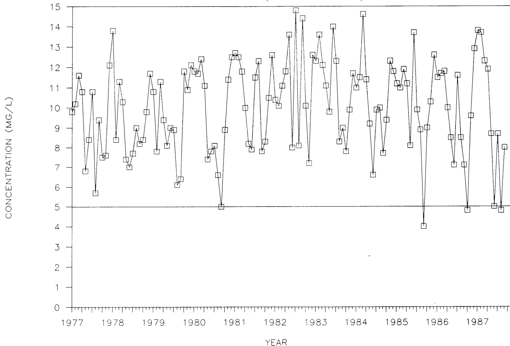
Figure III-5. Monthly dissolved oxygen concentrations in the Saginaw River (at the Center Street bridge, 1977-1987).
