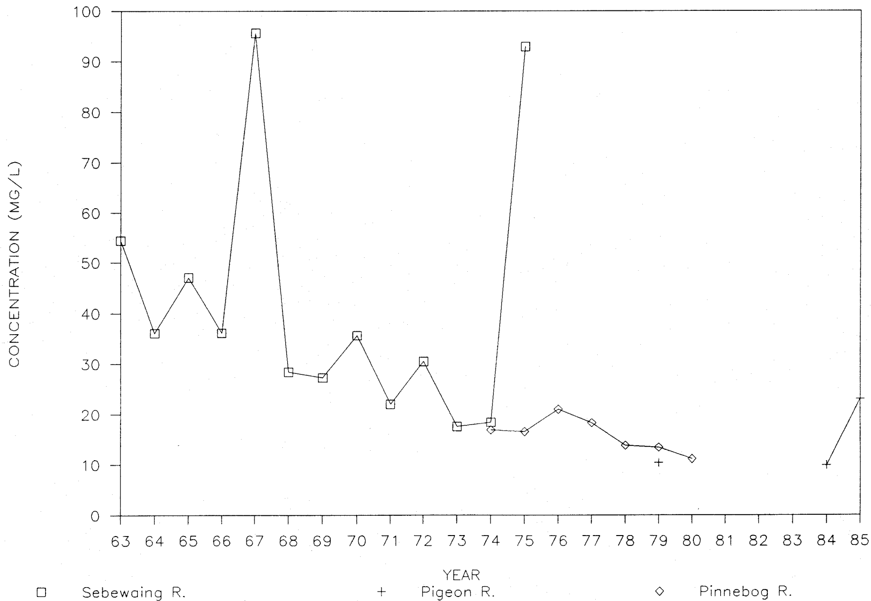
Figure III-16. Annual average suspended solids concentrations in Saginaw Bay east coastal basin tributaries, 1963-1985.
