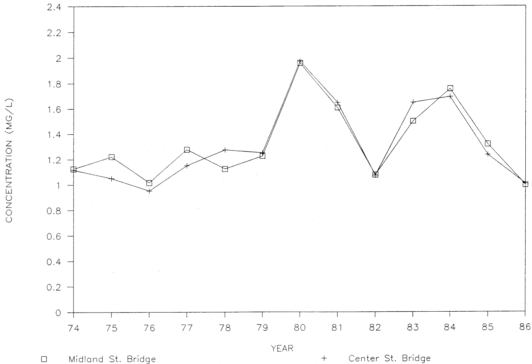
Figure III-31. Annual average nitrate-nitrite concentrations in Saginaw River water samples, 1974-1986.
