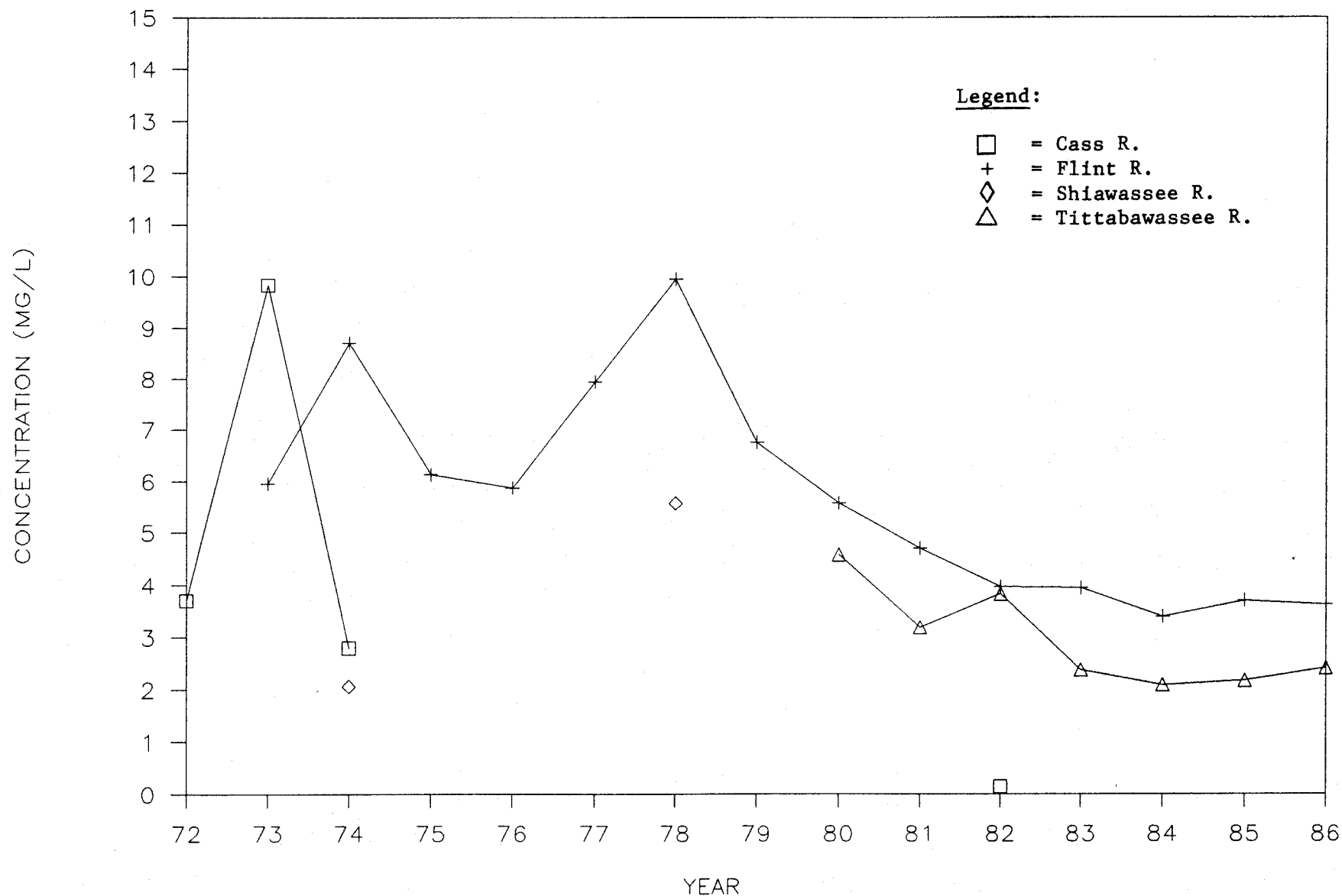
Figure III-7. Annual average biochemical oxygen demand in Saginaw River tributaries, 1972-1986.
