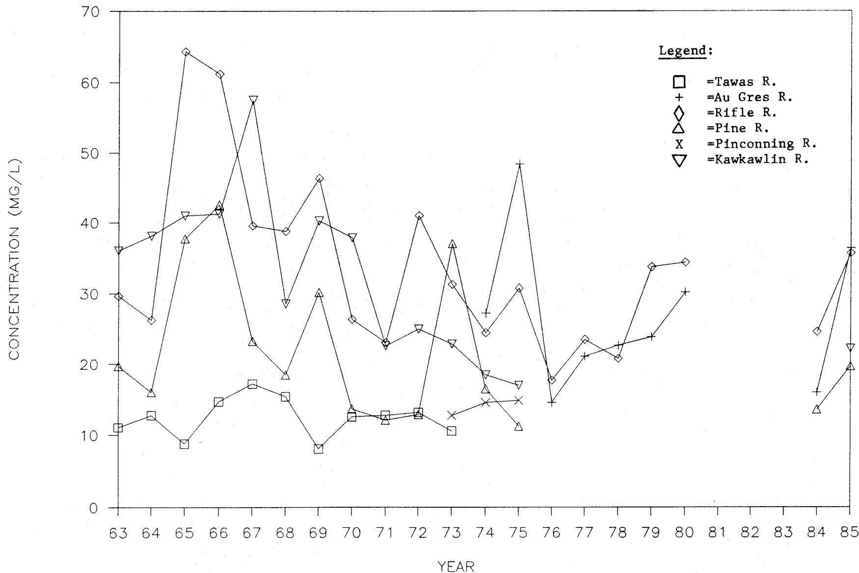
Figure III-15. Annual average suspended solids concentrations in Saginaw Bay west coastal basin tributaries, 1963-1985.
