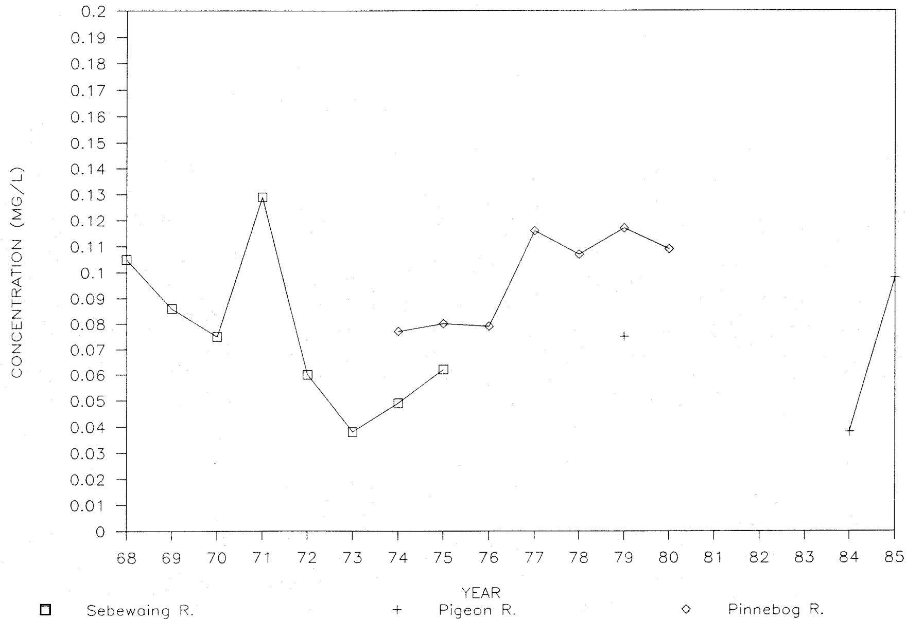
Figure III-28. Annual average orthophosphorus concentrations in Saginaw Bay east coastal basin tributaries, 1968-1985.
