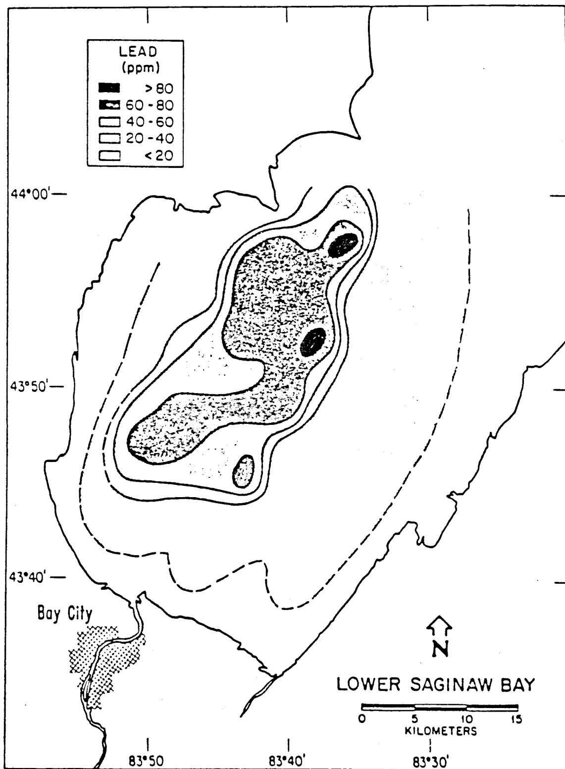
Figure III-83. Spatial distribution of lead in surface sediments (1-2 cm) of inner Saginaw Bay, 1978 (Robbins, 1986).
