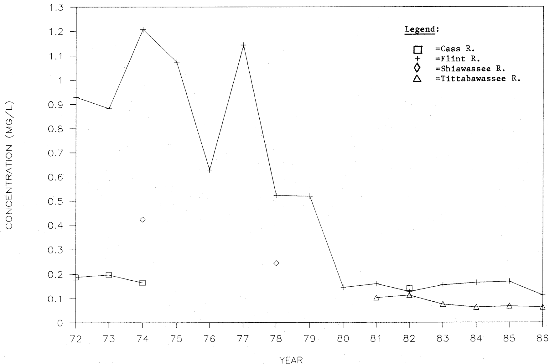
Figure III-23. Annual average total phosphorus concentrations in Saginaw River tributaries, 1972-1986.
