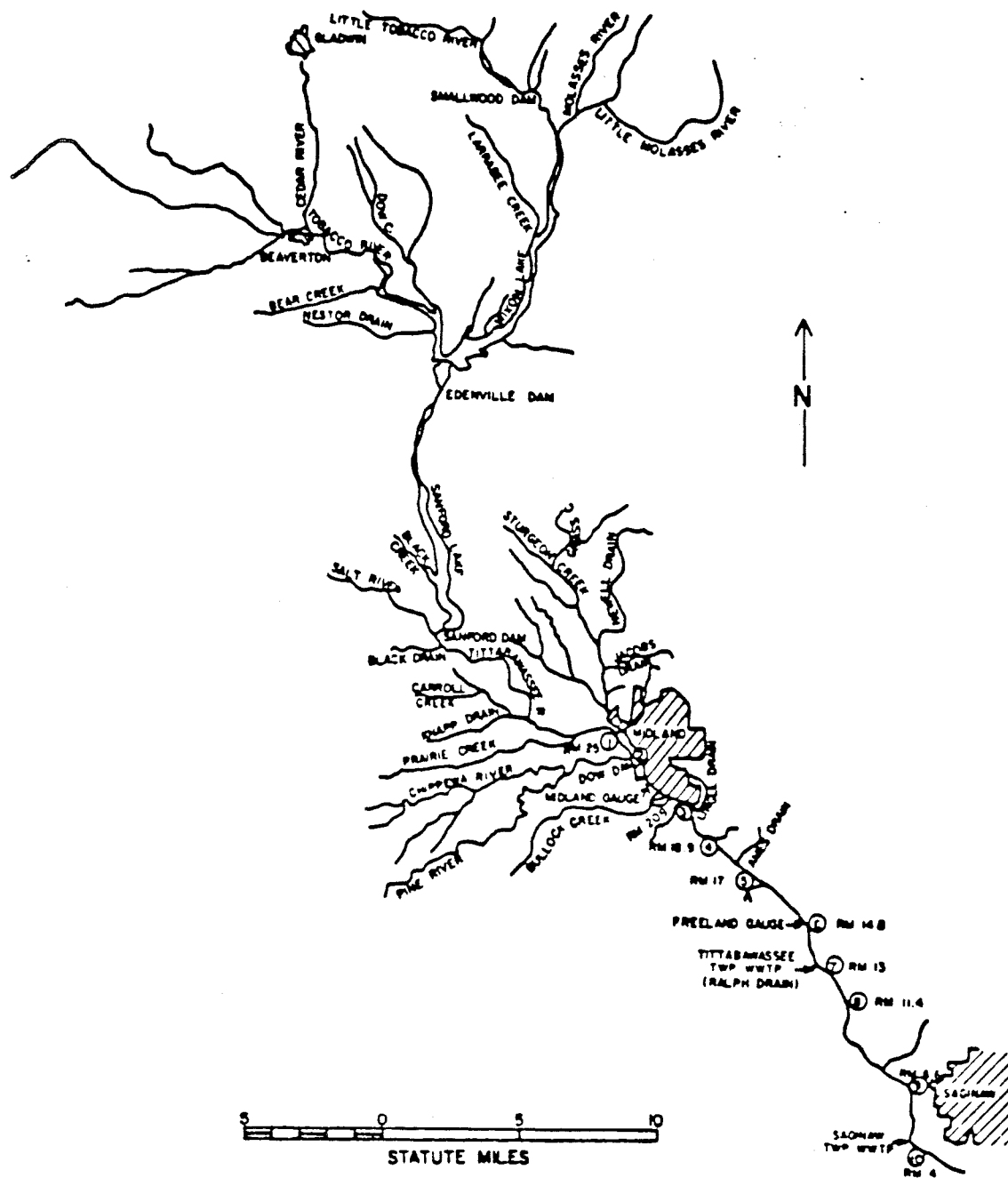
Figure III-49. Tittabawassee River sediment sampling sites for 1981 (Rossman, et al., 1983).
