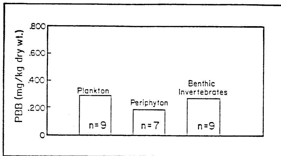
Figure III-97. Average PBB concentrations (mg/kg dry weight) in Pine River plankton, periphyton and benthic invertebrates (LTI, 1983).
