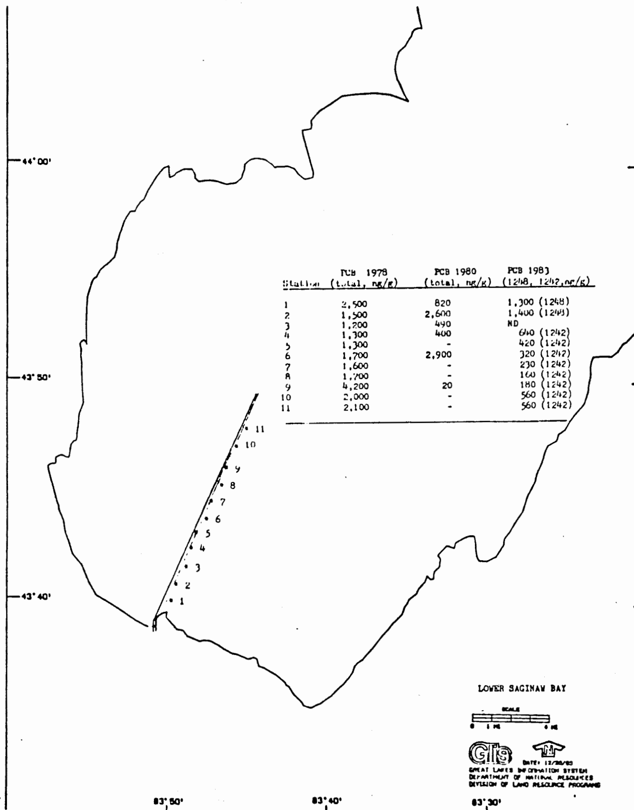
Figure III-78. PCB concentrations in sediments of inner Saginaw Bay collected from the navigation channel at the mouth of the Saginaw River 1978, 1980 and 1983 (USACOE, unpublished).
