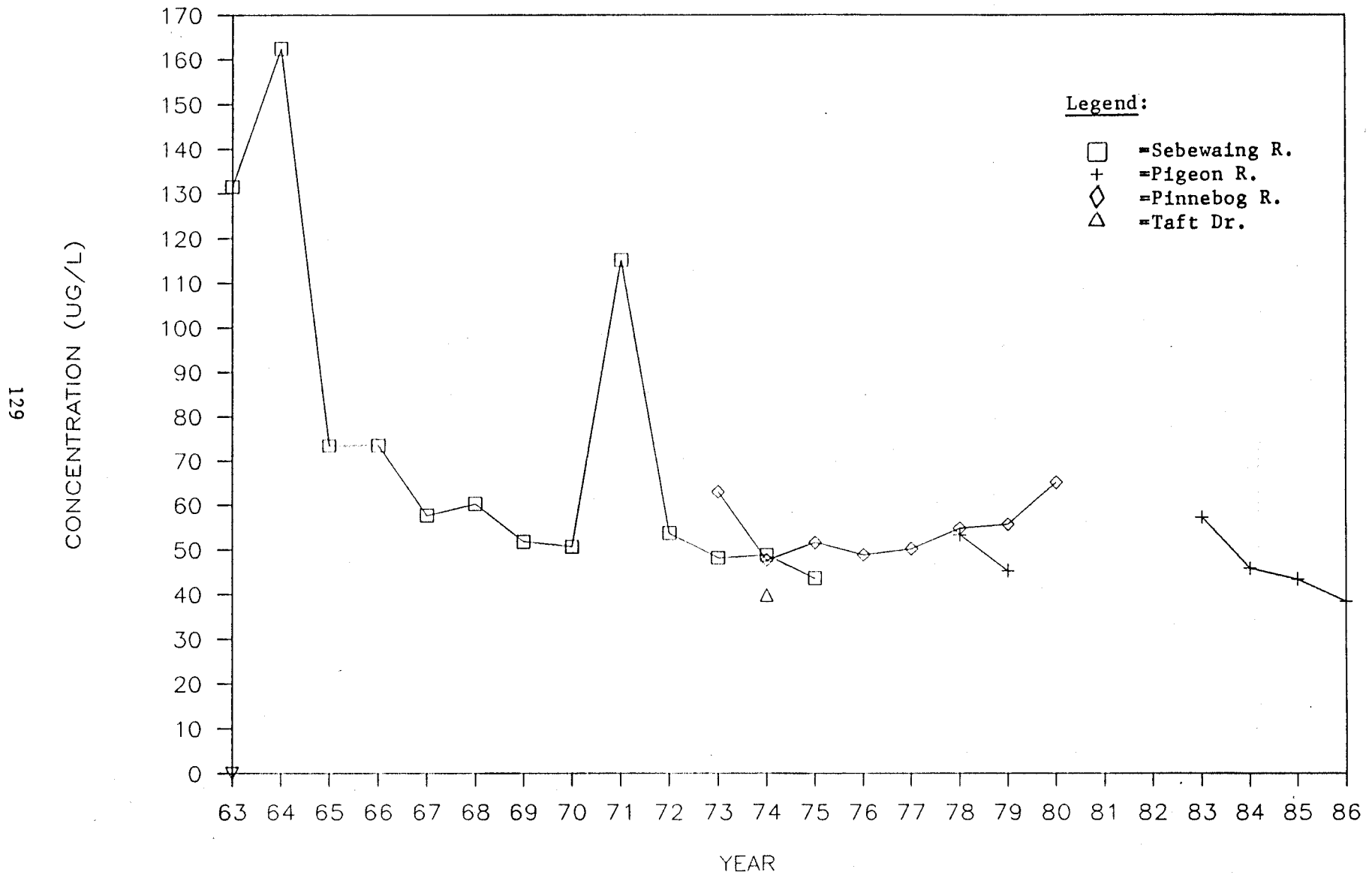
Figure III-39. Annual average chloride concentrations in Saginaw Bay east coastal basin tributaries, 1963-1986.
