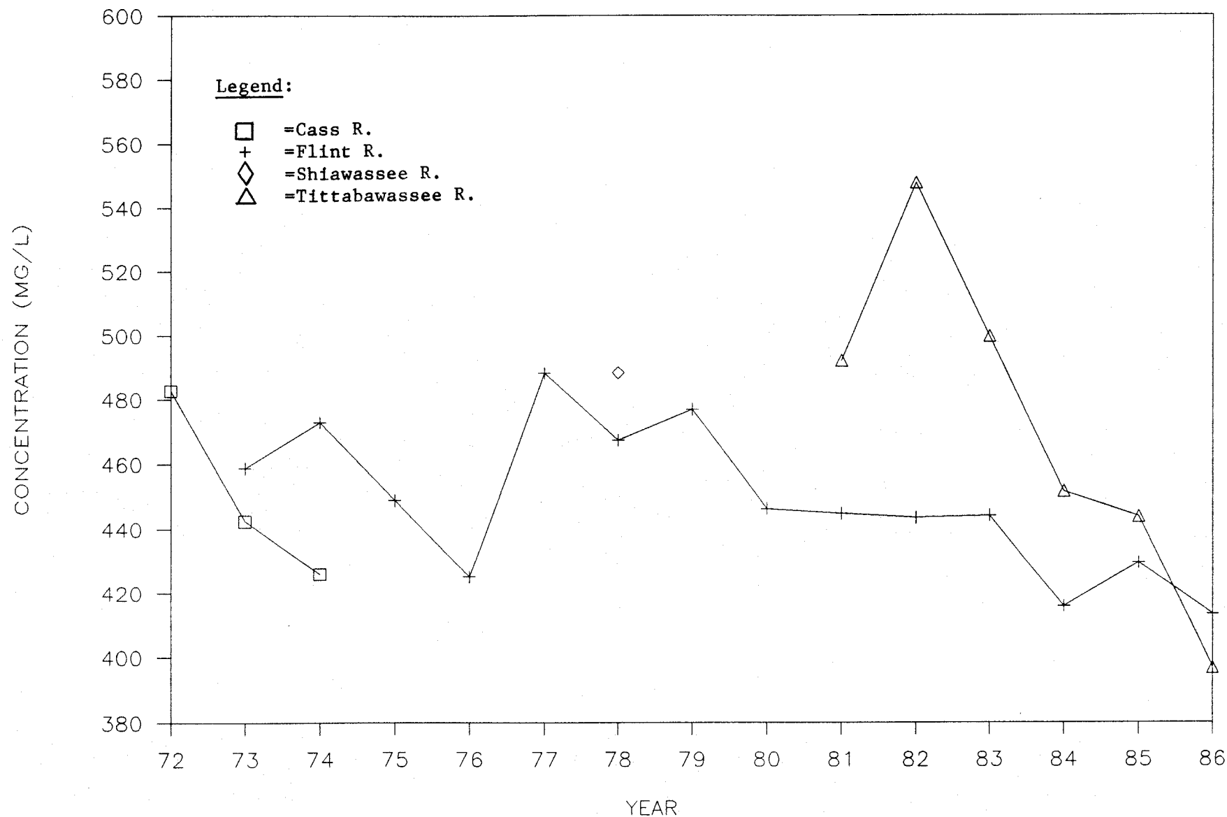
Figure III-18. Annual average total solids concentrations in Saginaw River tributaries, 1972-1986.
