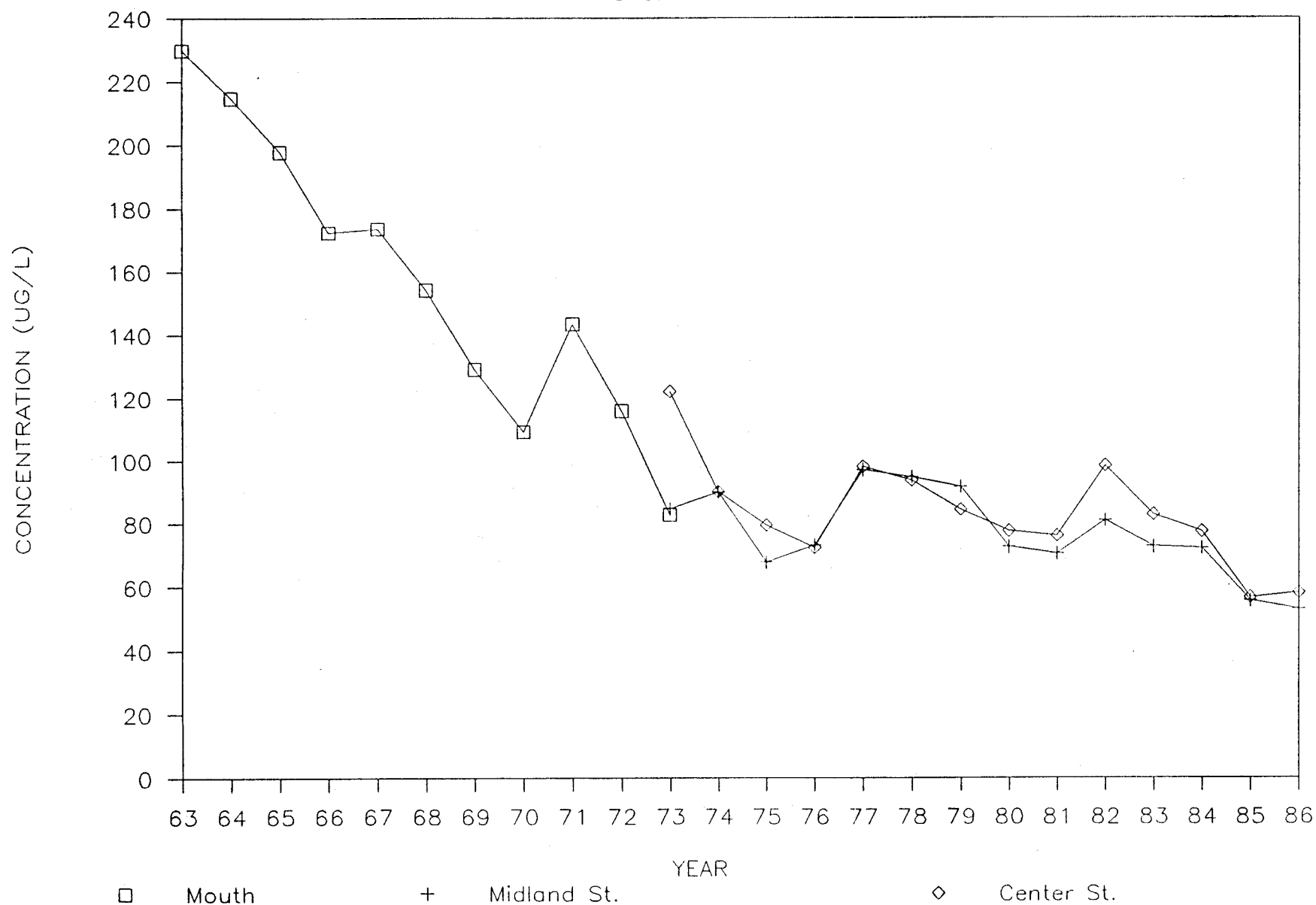
Figure III-36. Annual average chloride concentrations in Saginaw River water samples, 1963-1986.
