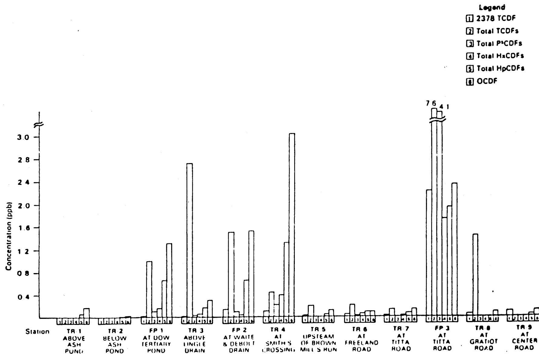
Figure III-52. PCDFs (ug/kg) in Tittabawasee River sediment and flood plain samples, July 1984 (USEPA, 1986).
