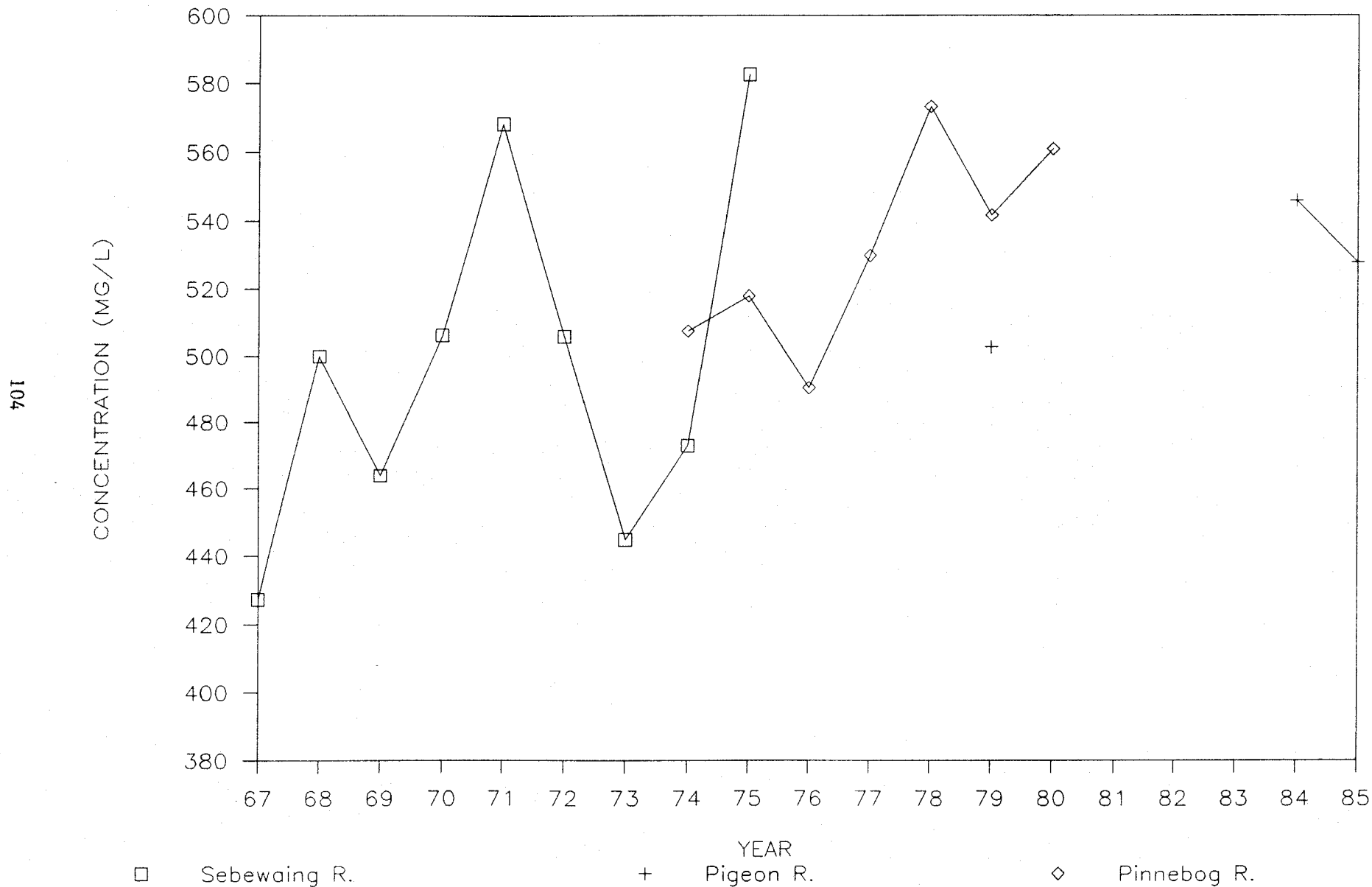
Figure III-20. Annual average total solids concentrations in Saginaw Bay east coastal basin tributaries, 1967-1985.
