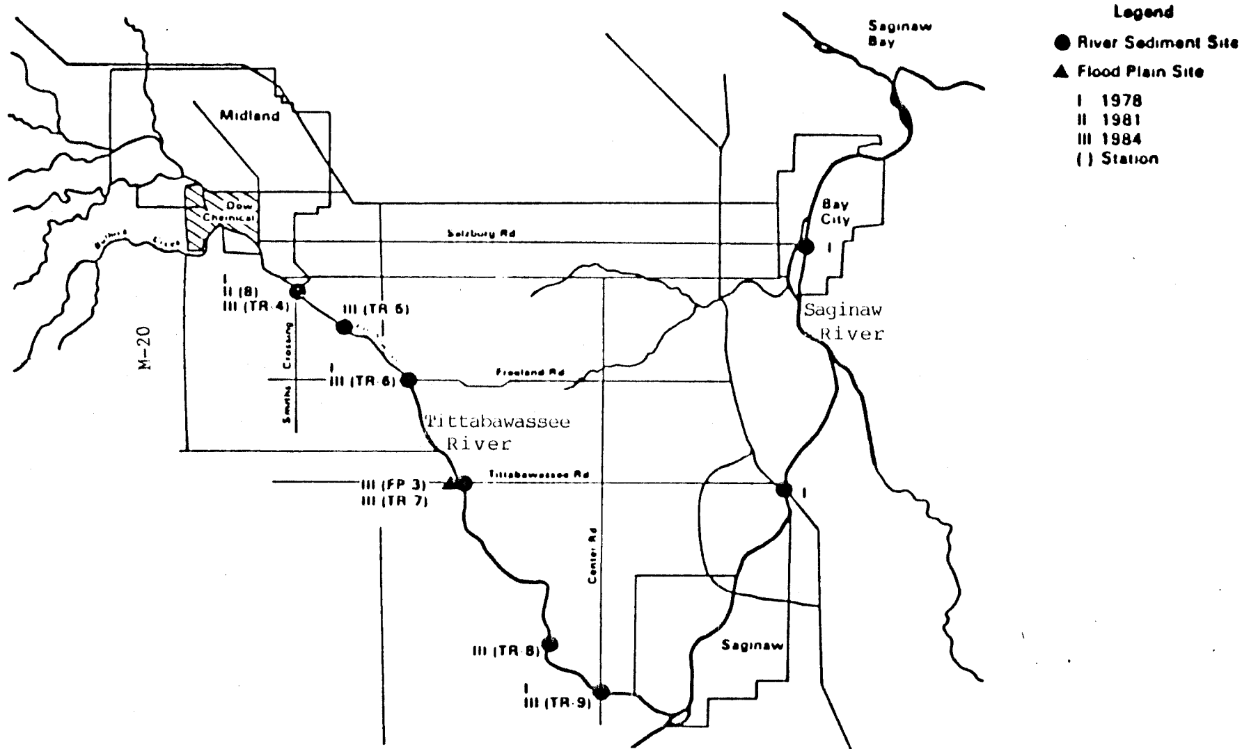
Figure III-48. Tittabawassee River and Saginaw River sediment sampling stations, 1978-1984 (USEPA, 1986).
