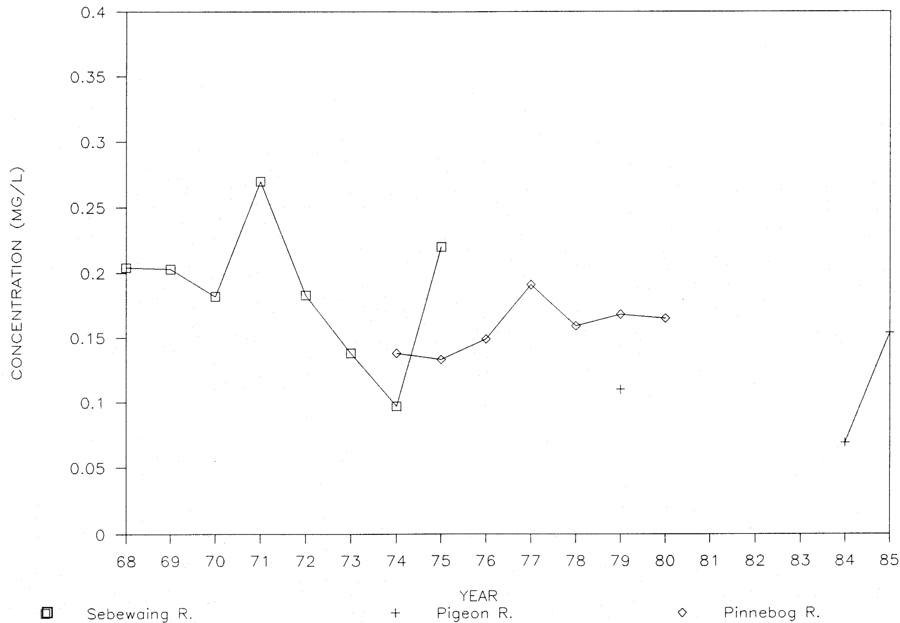
Figure III-27. Annual average total phosphorus concentrations in Saginaw Bay east coastal basin tributaries, 1968-1985.
