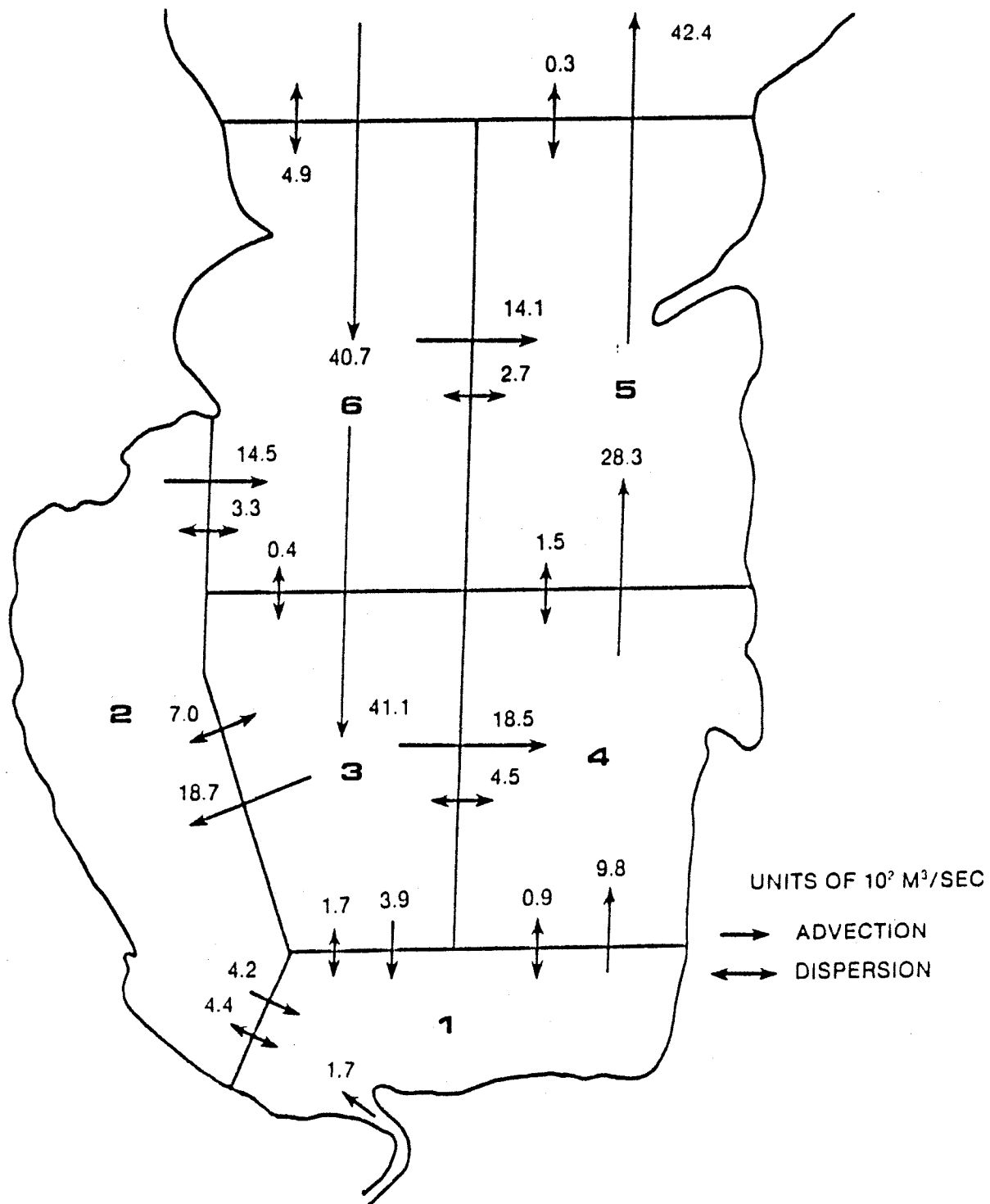
Figure II-11. An advection and dispersion model for Saginaw Bay (Limno-Tech, 1977).
