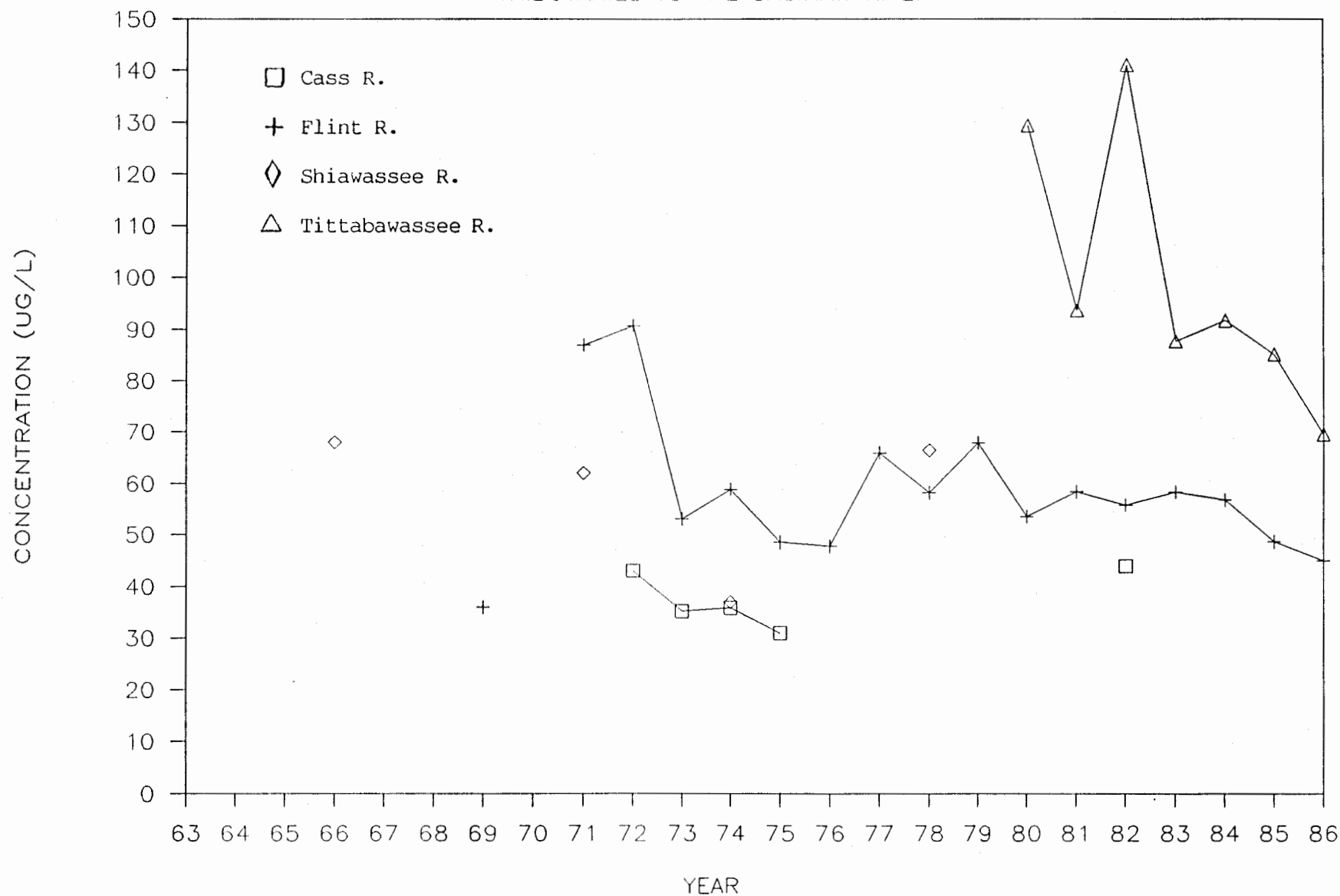
Figure III-37. Annual average chloride concentrations in Saginaw River tributaries, 1963-1986.
