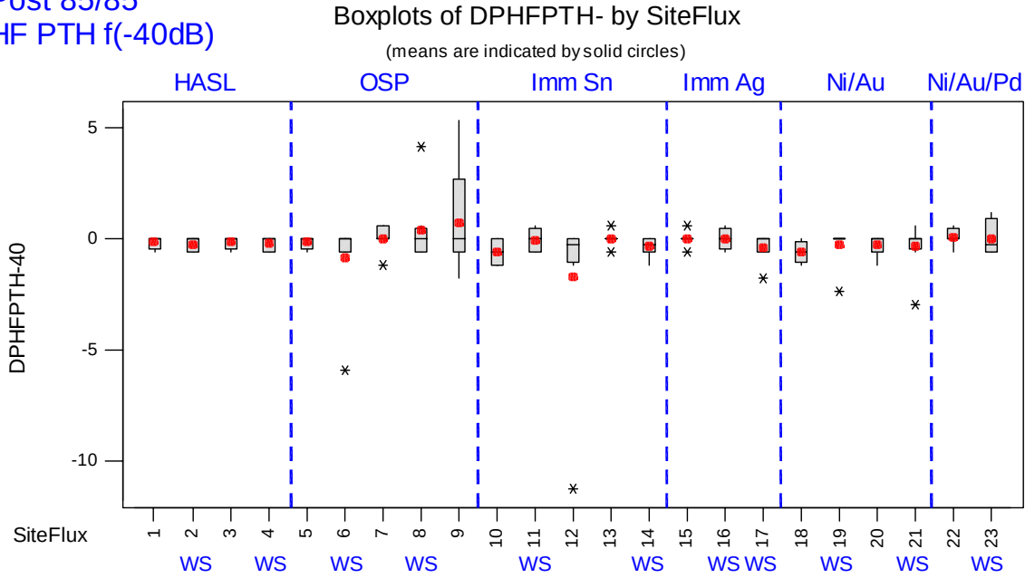
Figure F.17 Boxplot Displays for HF PTH f(-40dB) Post 85/85 - Pre-test Measurements (MHz) by Surf. Fin. (Acceptance Criterion = \pm 50 Mhz of Pre-test)
