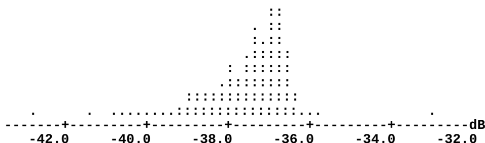
Figure F.66 Dotplot of 479 Measurements of the Response for HF TLC at 50 \text{ MHz} (each dot represents up to 4 points)
