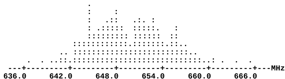
Figure F.69 Dotplot of 479 Measurements of the HF TLC Reverse Null Frequency (each dot represents up to 2 points)
