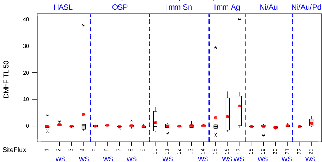
Figure 4-16. Boxplot Displays for HF TLC 50MHz Post MS - Pre-Test Measurements (dB) by Surface Finish
