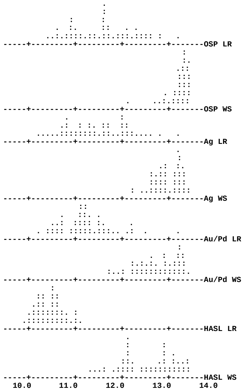
Figure F.73 Dotplots for 480 Measurements of Leakage on PGA A by Surface Finish and Flux
