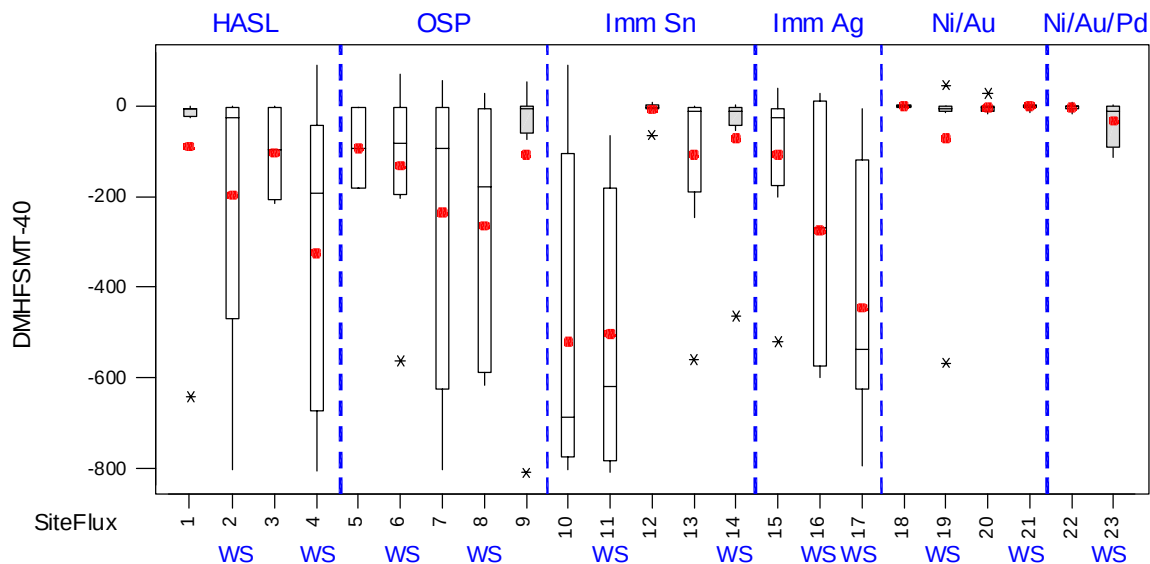
Figure 4-15. Boxplot Displays for HF SMT f(-40dB) Post MS - Pre-Test Measurements (MHz) by Surface Finish
