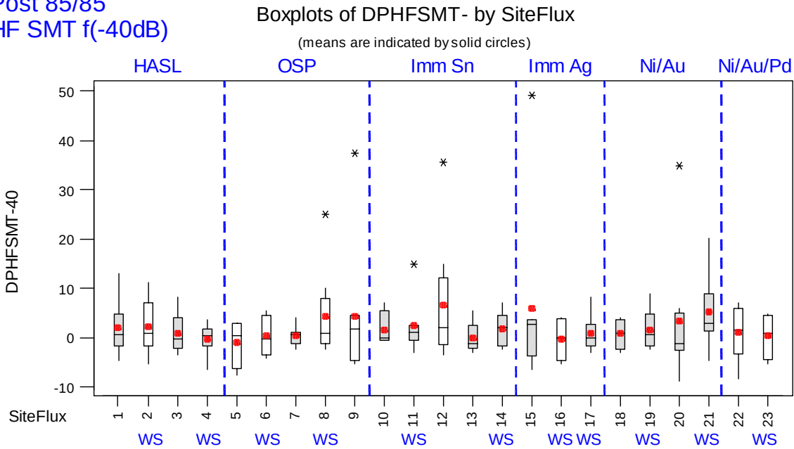
Figure F.26 Boxplot Displays for HF SMT f(-40dB) Post 85/85 - Pre-test Measurements (MHz) by Surf. Fin. (Acceptance Criterion = \pm 50 Mhz of Pre-test)
