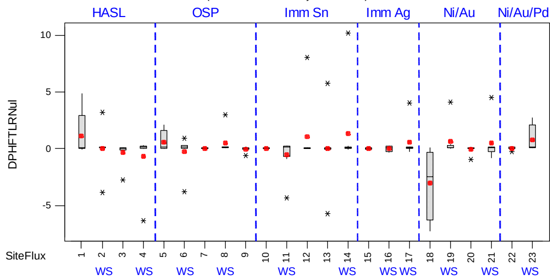
Figure F.35 Boxplot Displays for HF TLC RNR at Post 85/85 - Pre-test Measurements (dB) by Surf. Finish (Acceptance Criterion = <10 dB increase over Pre-test)
