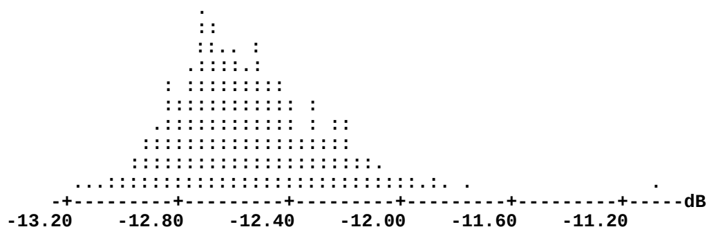
Figure F.68 Dotplot of 478 Measurements of the Response for HF TLC at 1000 MHz (each dot represents up to 2 points)
