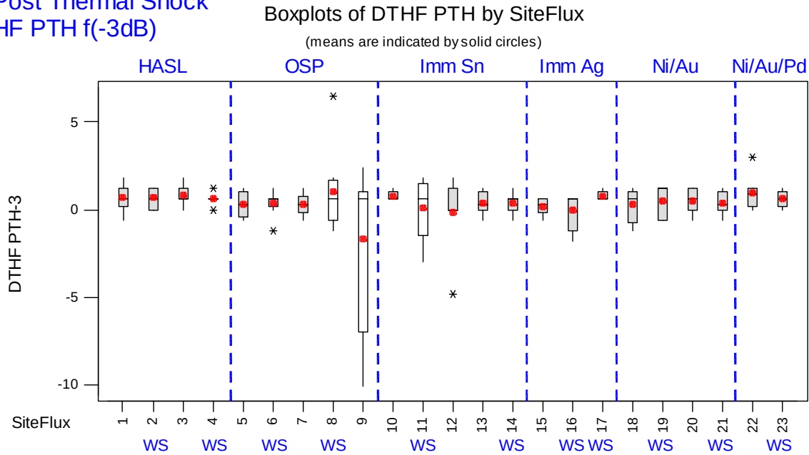
Figure F.15 Boxplot Displays for HF PTH f(-3dB) Post TS - Pre-test Measurements (Mhz) by Surface Finish (Acceptance Criterion = \pm 50 Mhz of Pre-test)
