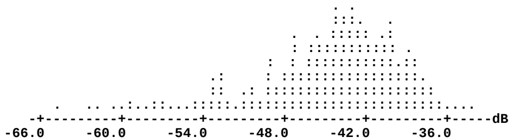
Figure F.70 Dotplot of 479 Measurements of the HF TLC Reverse Null Response (each dot represents up to 2 points)
