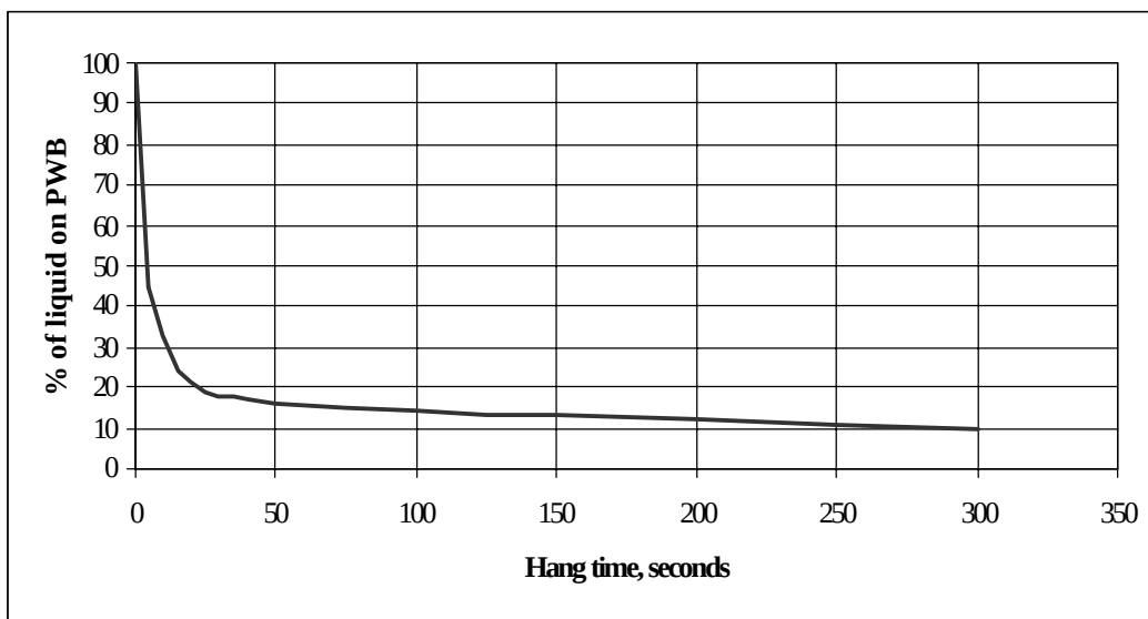
Figure 3. Drainage vs Hang Time (McKesson and Wegener 1998).
