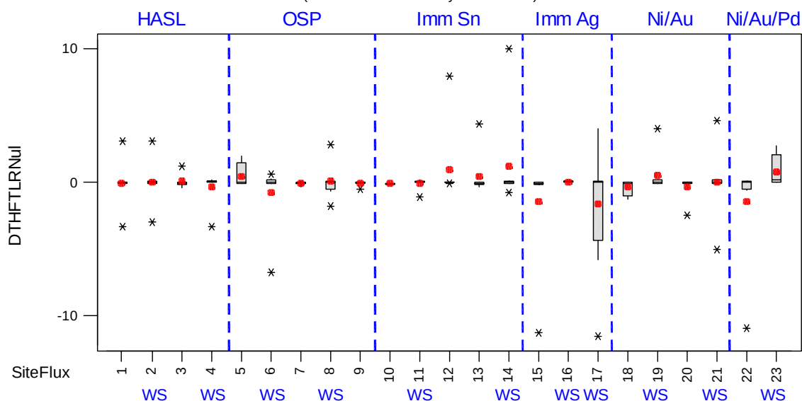
Figure F.36 Boxplot Displays for HF TLC RNR Post TS - Pre-test Measurements (dB) by Surface Finish (Acceptance Criterion = <10 dB increase over Pre-test)
