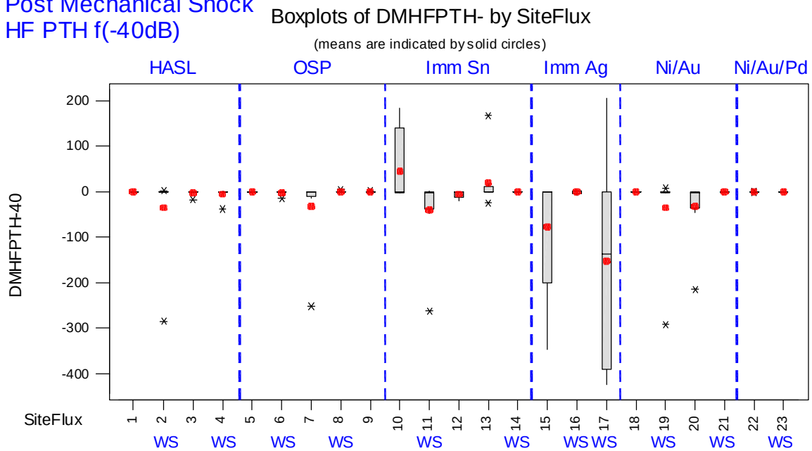
Figure 4-12. Boxplot Displays for HF PTH f(-40dB) Post MS - Pre-Test Measurements (MHz) by Surf. Finish
