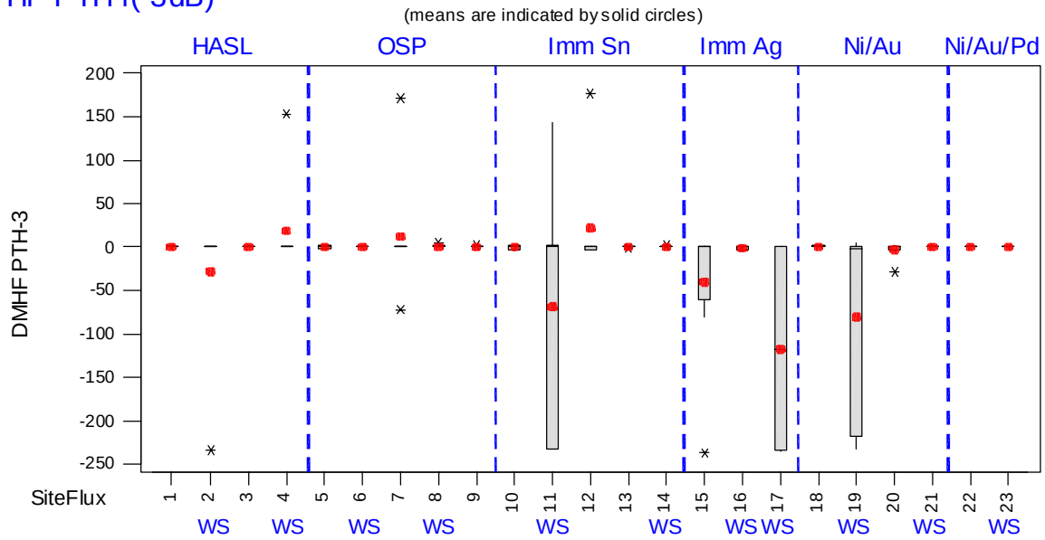
Figure 4-11. Boxplot Displays for HF PTH f(-3dB) Post MS - Pre-Test Measurements (MHz) by Surface Finish
