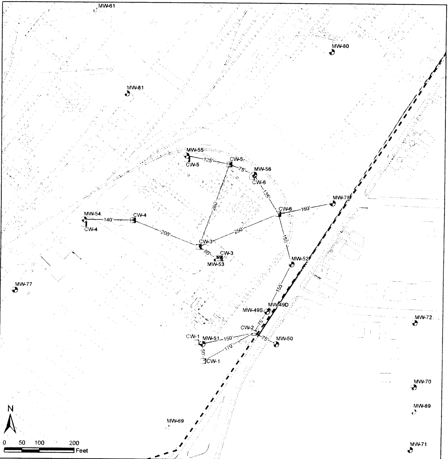
Figure 1 Proposed Containment Well Locations
