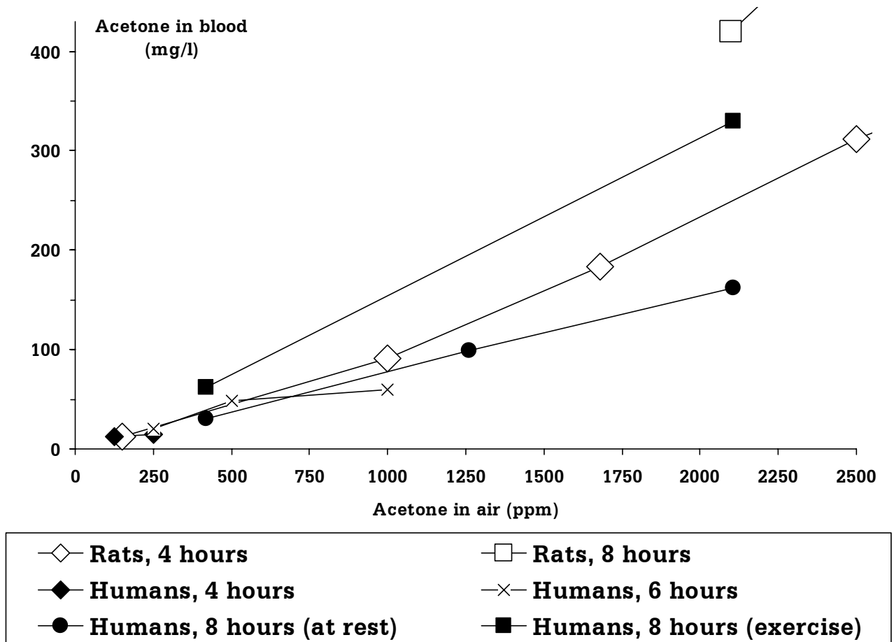
2 FIGURE 2: COMPARISON OF ACETONE CONCENTRATION IN BLOOD OF HUMANS AND 3 RATS FOLLOWING INHALATION (DATA FROM HAGGARD ET AL. 1944).
