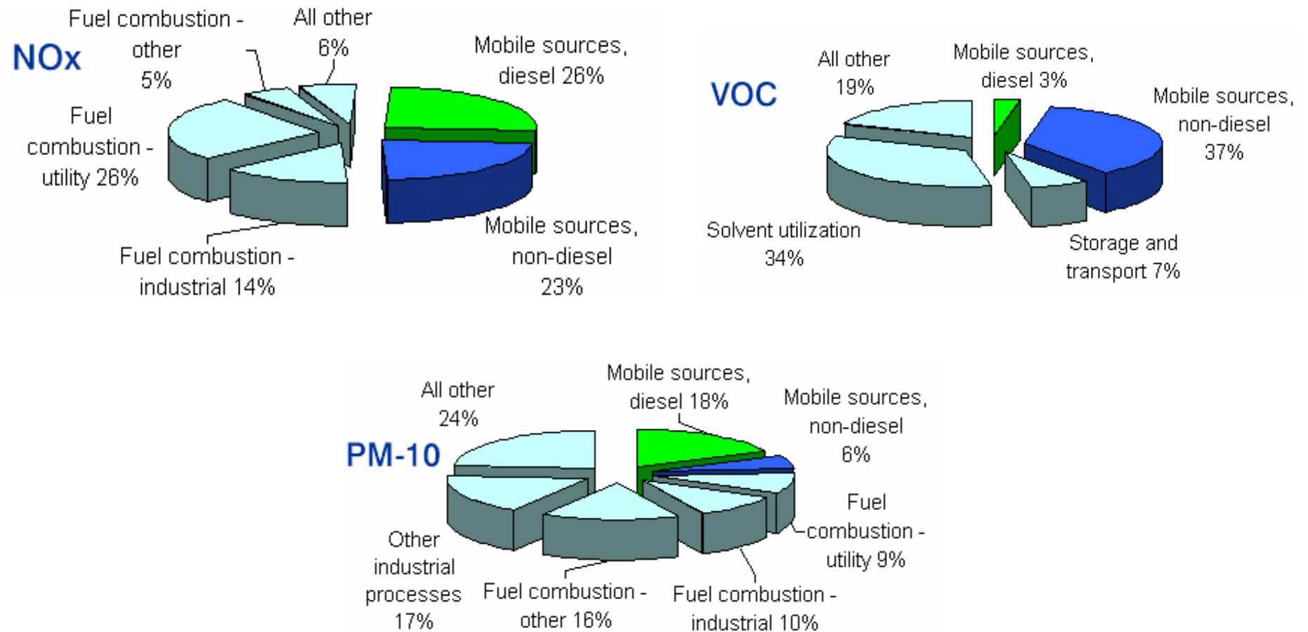
Figure II.1. Contribution of Mobile Sources to NO x , VOC, and PM Emissions
