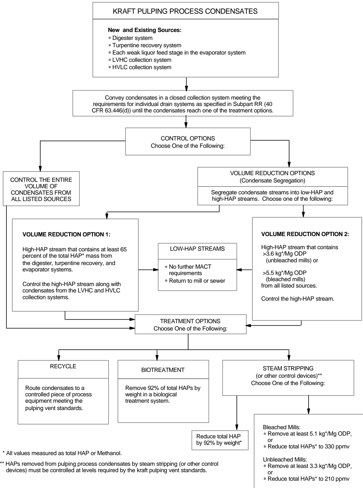
FIGURE 6. KRAFT PULPING PROCESS CONDENSATE STANDARDS (§63.446)
