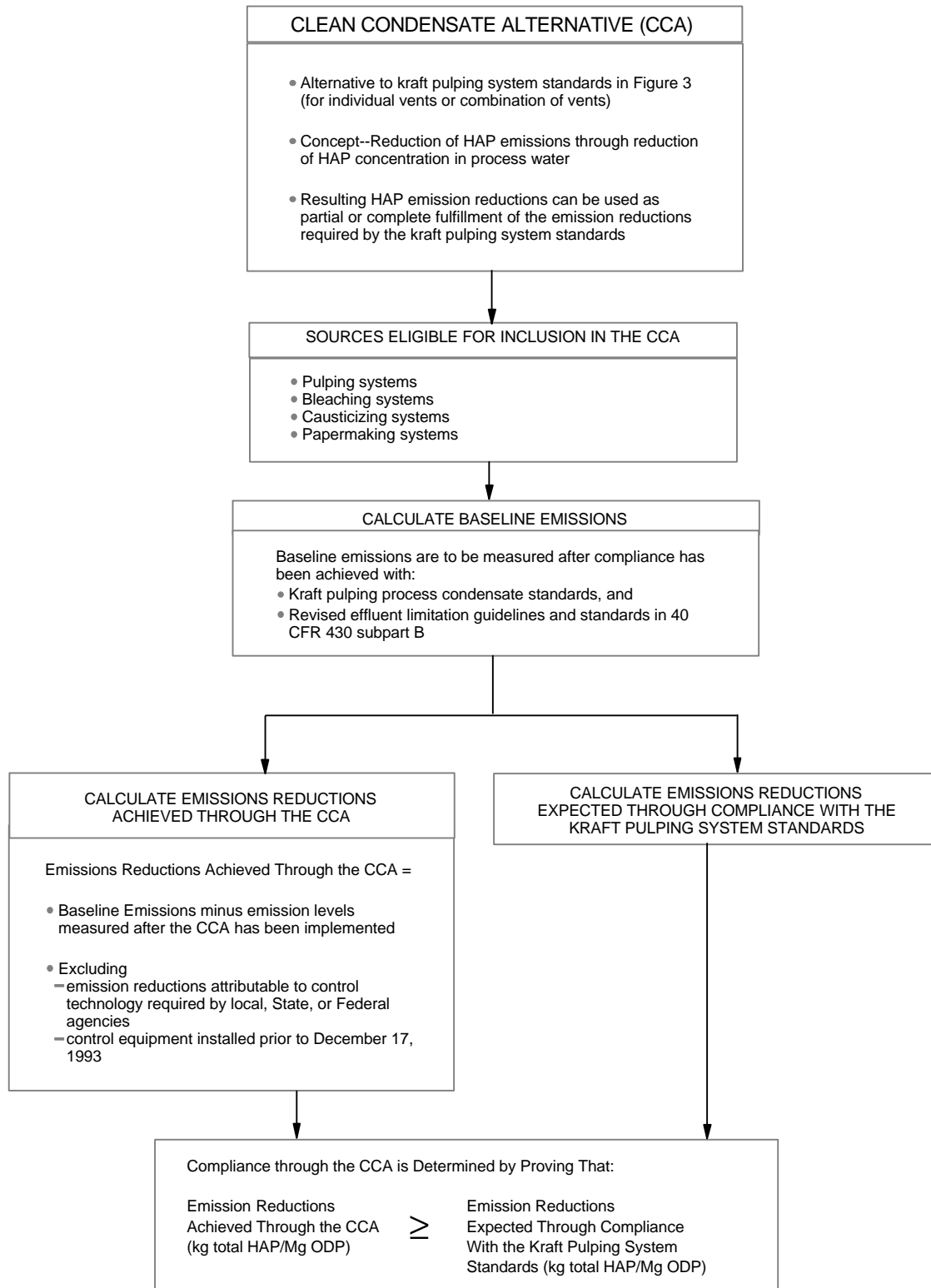
FIGURE 7. CLEAN CONDENSATE ALTERNATIVE (§63.447)
