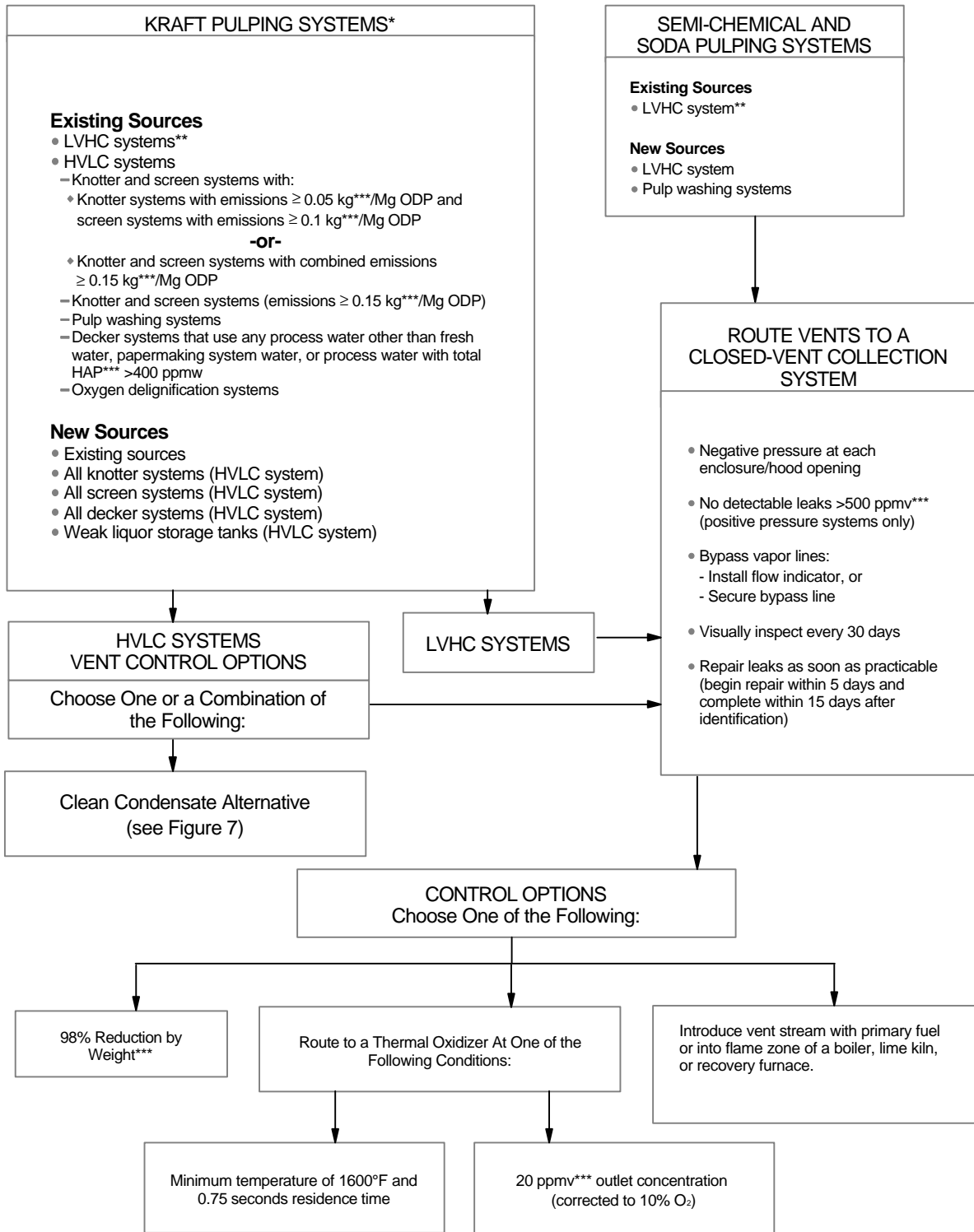
FIGURE 3. PULPING SYSTEM STANDARDS FOR KRAFT, SEMI-CHEMICAL, AND SODA PULPING MILLS (§63.443, §63.450)
