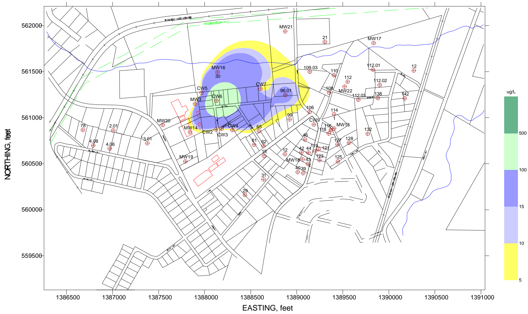
FIGURE 4-13 BEDROCK GROUNDWATER PLUME (BEDROCK MW and POTABLE WELLS) TCE CONTAMINATION, OCTOBER/NOVEMBER 1996 REMEDIAL INVESTIGATION REPORT NORTH BELMONT PCE SUPERFUND SITE NORTH BELMONT, GASTON COUNTY, NC SESD PROJECT No. 96S-058, JUNE 1997
