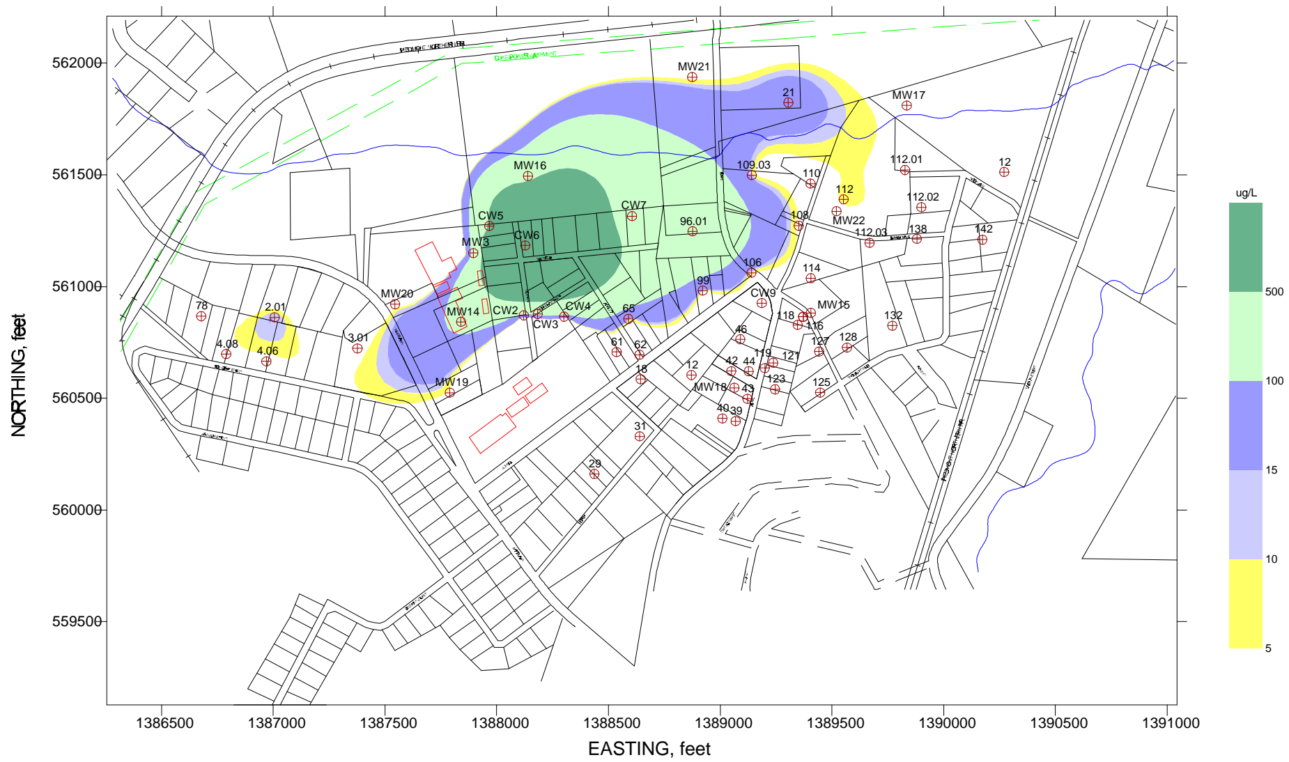
FIGURE 4-12 BEDROCK GROUNDWATER PLUME (BEDROCK MW and POTABLE WELLS) NOT TO SCALE PCE CONTAMINATION, OCTOBER/NOVEMBER 1996 REMEDIAL INVESTIGATION REPORT NORTH BELMONT PCE SUPERFUND SITE NORTH BELMONT, GASTON COUNTY, NC SESD PROJECT No. 96S-058, JUNE 1997
