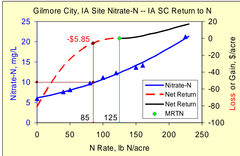
Fig. 6. Tile-flow nitrate-N annual concentration average in a SC rotation from N rates applied in various years from 1990-2004 at the Gilmore City, IA site (Lawlor et al., 2005) and the net economic gain or loss ($0.22/lb N:$2.20/bu corn) across N rates for SC in Iowa (Nafziger et al., 2004). The solid black section of the net return line represents the gain if N rates are reduced to the maximum return to N (MRTN), and the red dashed section represents the loss if N rates are reduced below the MRTN. The indicated economic loss is for reduction of tile-flow nitrate-N from the MRTN rate to the N rate that results in approximately the 10 mg/L MCL drinking water standard.
