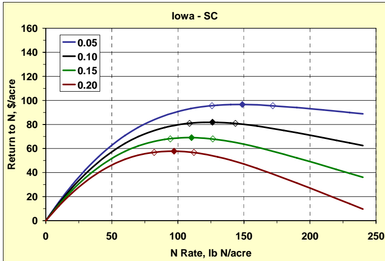
Fig. 4. Effect of fertilizer N:corn grain price ratio on net return to N (SC and CC rotations in Iowa). The closed symbols correspond to the maximum return to N (MRTN) and open symbols the range around the MRTN with similar return.
