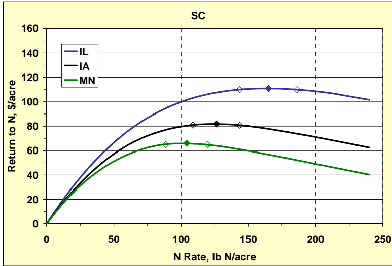
Fig. 5. Differences between net return to N for SC and CC for various states at a 0.10 N:corn price ratio ($0.22/lb N:$2.20/bu corn). The closed symbols correspond to the maximum return to N (MRTN) and open symbols the range around the MRTN with similar return. Response data courtesy of Emerson Nafziger, Univ. of Illinois and Gyles Randall, Univ. of Minnesota.
