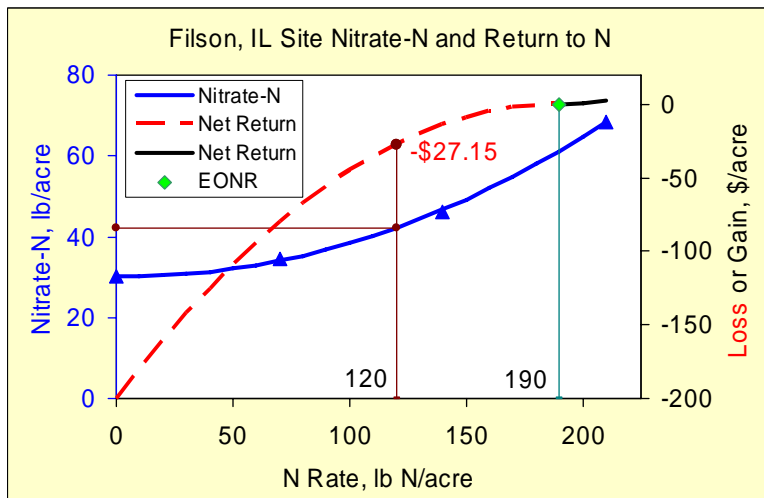
Fig. 7. Rotation total tile-flow nitrate-N mass load and net economic gain or loss ($0.22/lb N:$2.20/bu corn) across spring-applied N rates in a SC rotation, average of 2002-2004 at the Filson, IL site (M. Clover, M.S. Thesis, Univ. of Illinois). The solid black section of the net return line represents the gain if N rates are reduced to the site economic optimum N rate (EONR), and the red dashed section represents the loss if N rates are reduced below the EONR. The indicated economic loss is for reduction of tile-flow nitrate-N load from the EONR rate to the N rate that results in an approximate 30% lower load.
