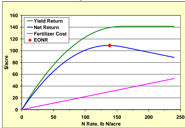
Fig. 1. Example corn grain yield and fertilizer components of calculated economic net return across N rates from a N response trial, with the economic optimum N rate (EONR) at 0.10 N:corn price ratio ($0.22/lb N:$2.20/bu corn) indicated by closed symbol.
