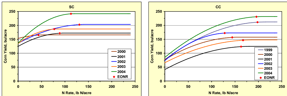
Fig. 2. Variation in EONR (0.10 price ratio) and yield across years for SC and CC at the same site location, Ames, Iowa.
