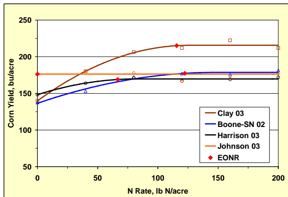
Fig. 3. Example of variation in response to N and EONR (0.10 price ratio) at different locations in Iowa.
