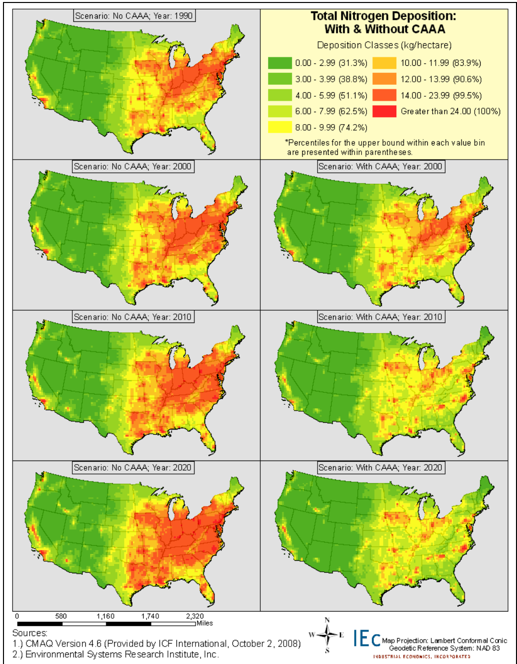
EXHIBIT 3-3 TOTAL NITROGEN DEPOSITION ESTIMATES FOR 1990, 2000, 2010, AND 2020 WITH AND WITHOUT THE CAAA 10, 11
