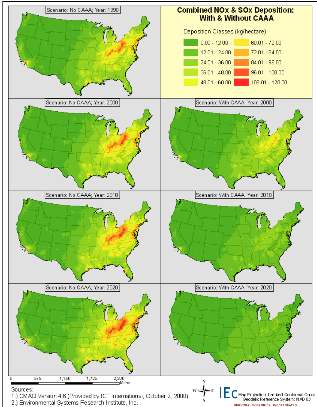
EXHIBIT 3-1 COMBINED NO x AND SO x DEPOSITION ESTIMATES FOR 1990, 2000, 2010, AND 2020 WITH AND WITHOUT THE CAAA
