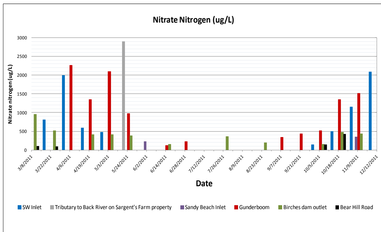
Figure 3-6: Ambient nitrate-nitrogen concentrations from the major inflows and Birch Dam outlet during the survey period.
