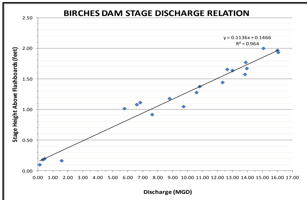
Figure 2-4: Birches Dam rating curve developed in 2011 from velocity and water elevation measurements
