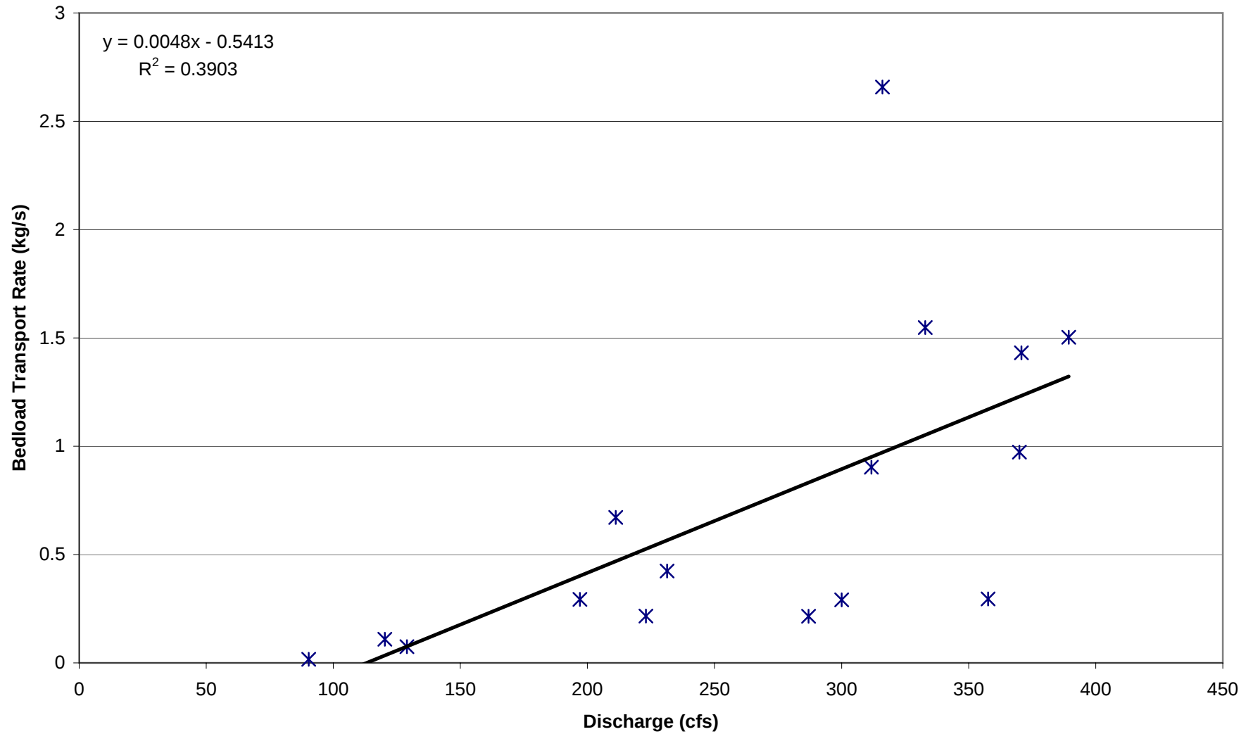
Figure 120. Weminuche Creek Bedload Rating Curve 2001
