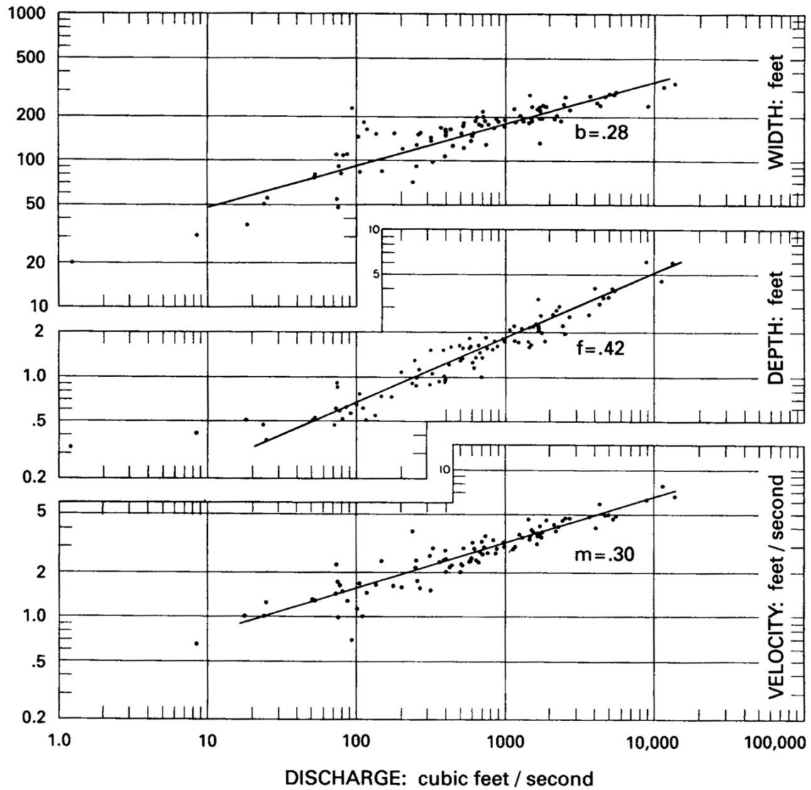
Figure 105. Hydraulic geometry for Powder River, Montana (Leopold, 1994).
