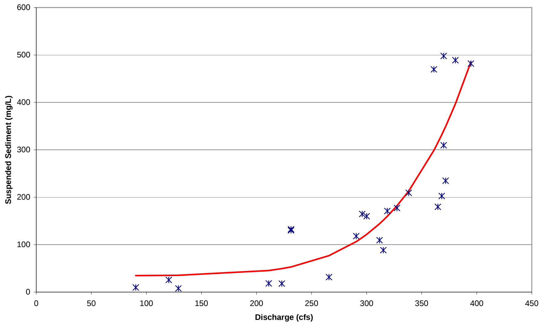
Figure 119. Weminuche Creek 2001 Suspended Sediment Rating Curve
