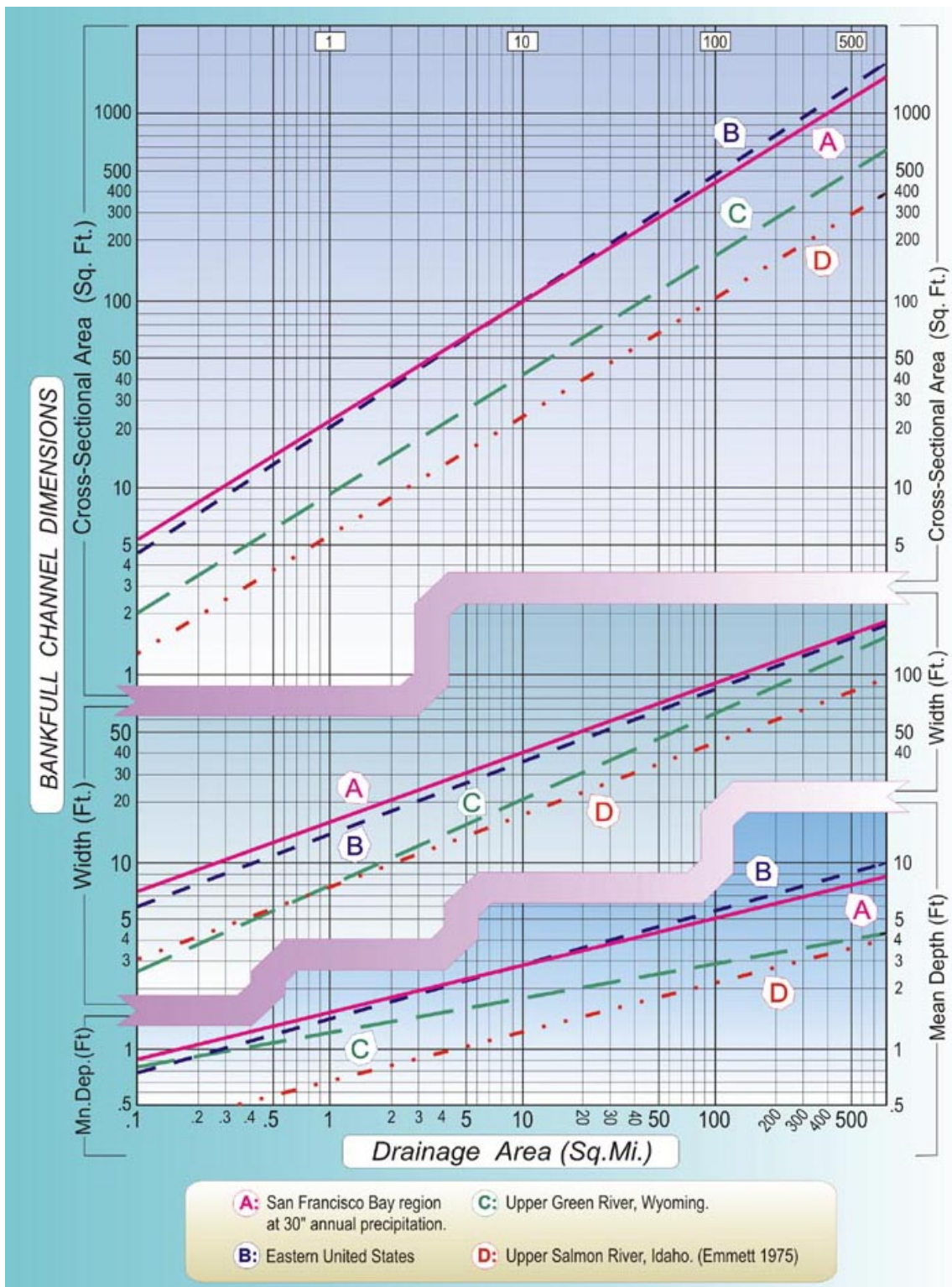
Figure 99. Regional curves showing bankfull dimensions vs drainage areas for various hydro-physiographic provinces (Dunn and Leopold, 1978).
