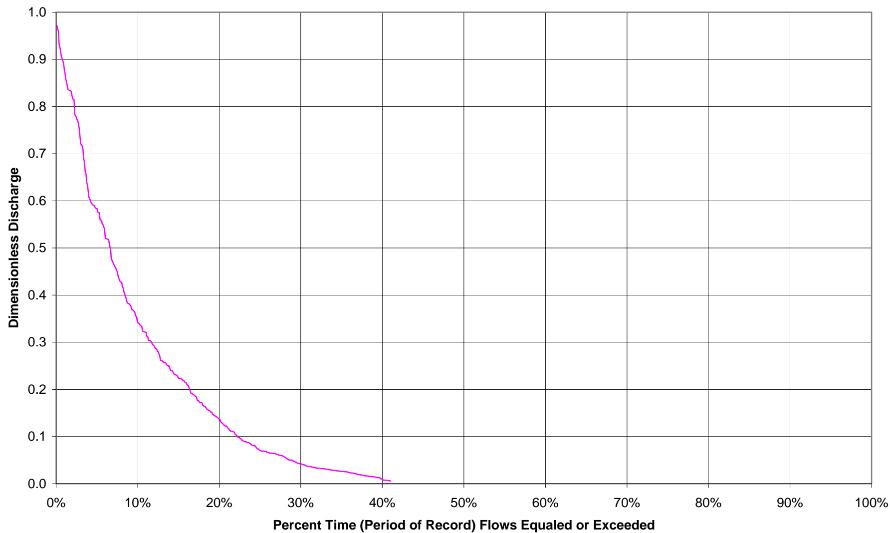
Figure 118. Dimensionless Flow Duration Curve, 1999-2001, Weminuche Creek
