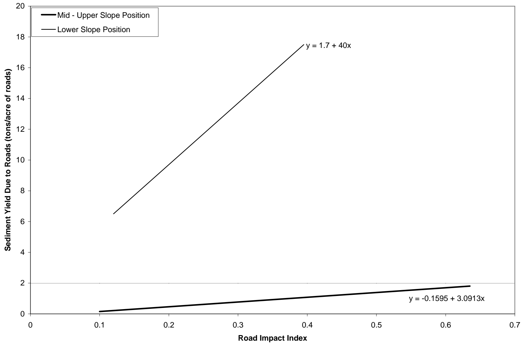
Figure 122. Relationship of sediment yield based on Road Impact Index (basic data from USDA Forest Service, Horse Creek Watershed, Idaho and Fool Creek, Colorado).
