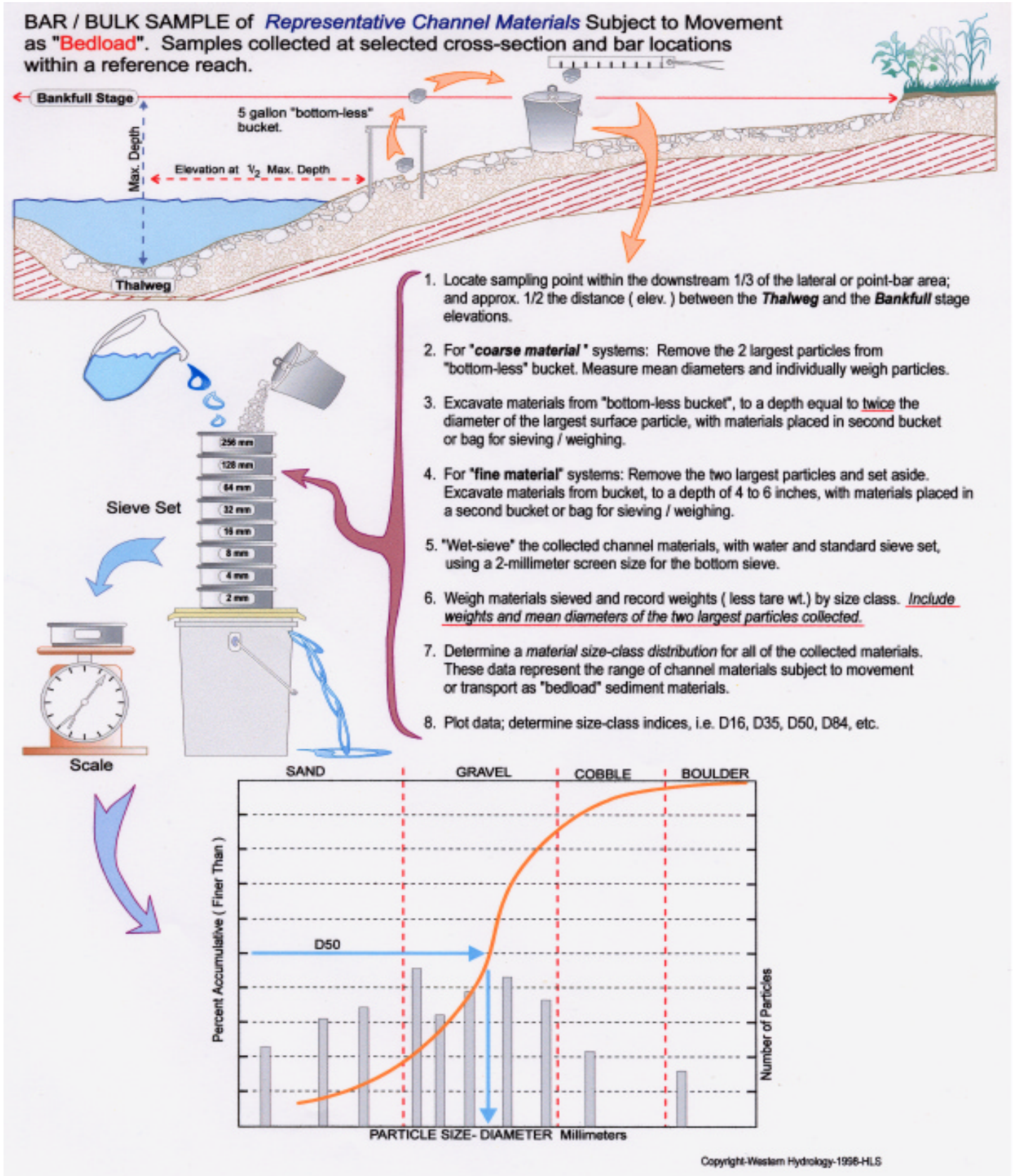
Figure 125. Field sample methods for bar sample
