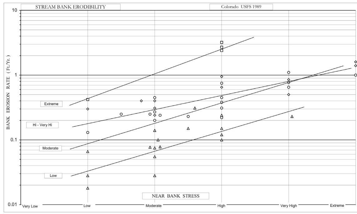
Figure 115. Relationship of BEHI and NBS to predict annual streambank erosion rates, Colorado data, 1989 (Rosgen 1996, 2001a).
