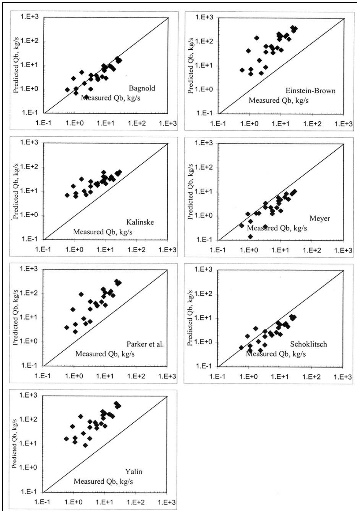
Figure 11. Comparisons of predicted and measured bedload rates for Chippewa River at Durand, WI. (Lopes et al. 2001a).
