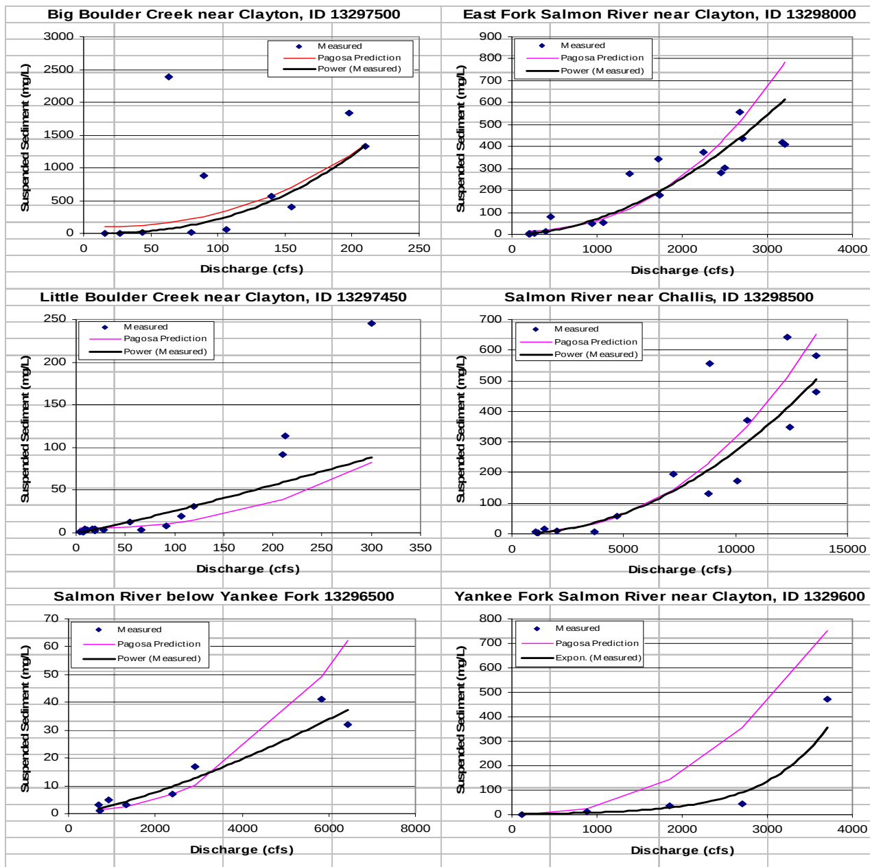
Figure 58. Examples of predicted versus measured suspended sediment data using reference dimensionless rating curve.
