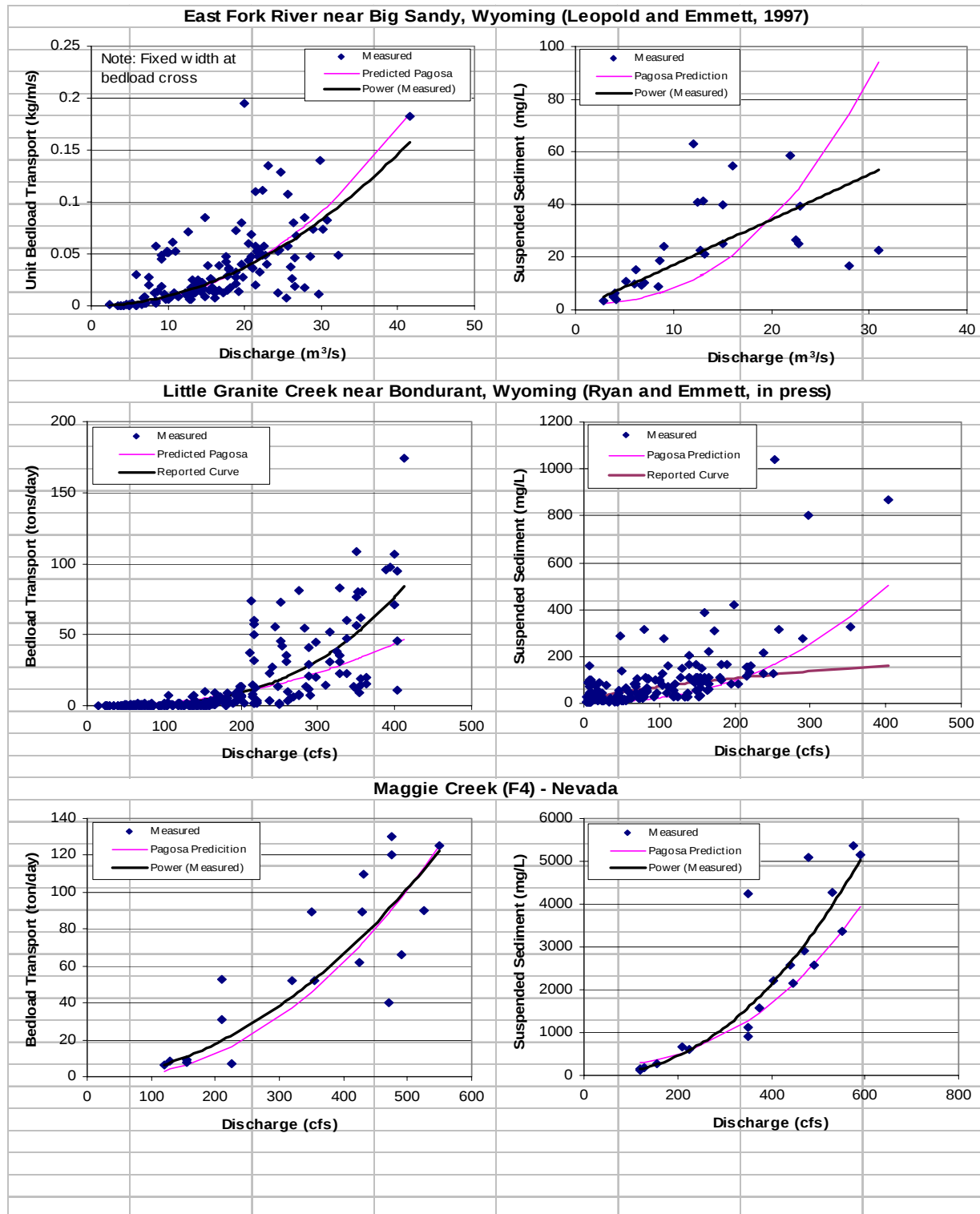
Figure 59. Examples of predicted versus measured bedload and suspended sediment data using reference dimensionless rating curve.
