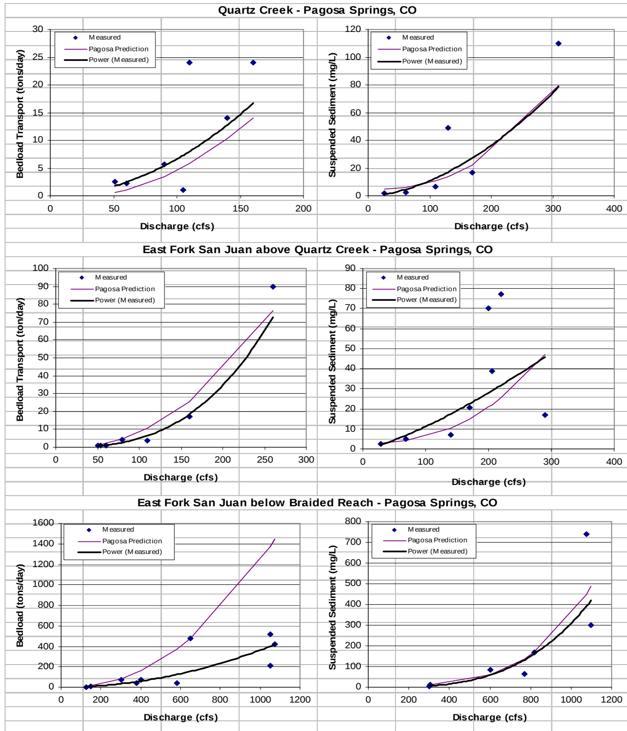
Figure 60. Example of predicted versus measured bedload and suspended sediment data using dimensionless reference curve (Data from Emmett, 1975)
