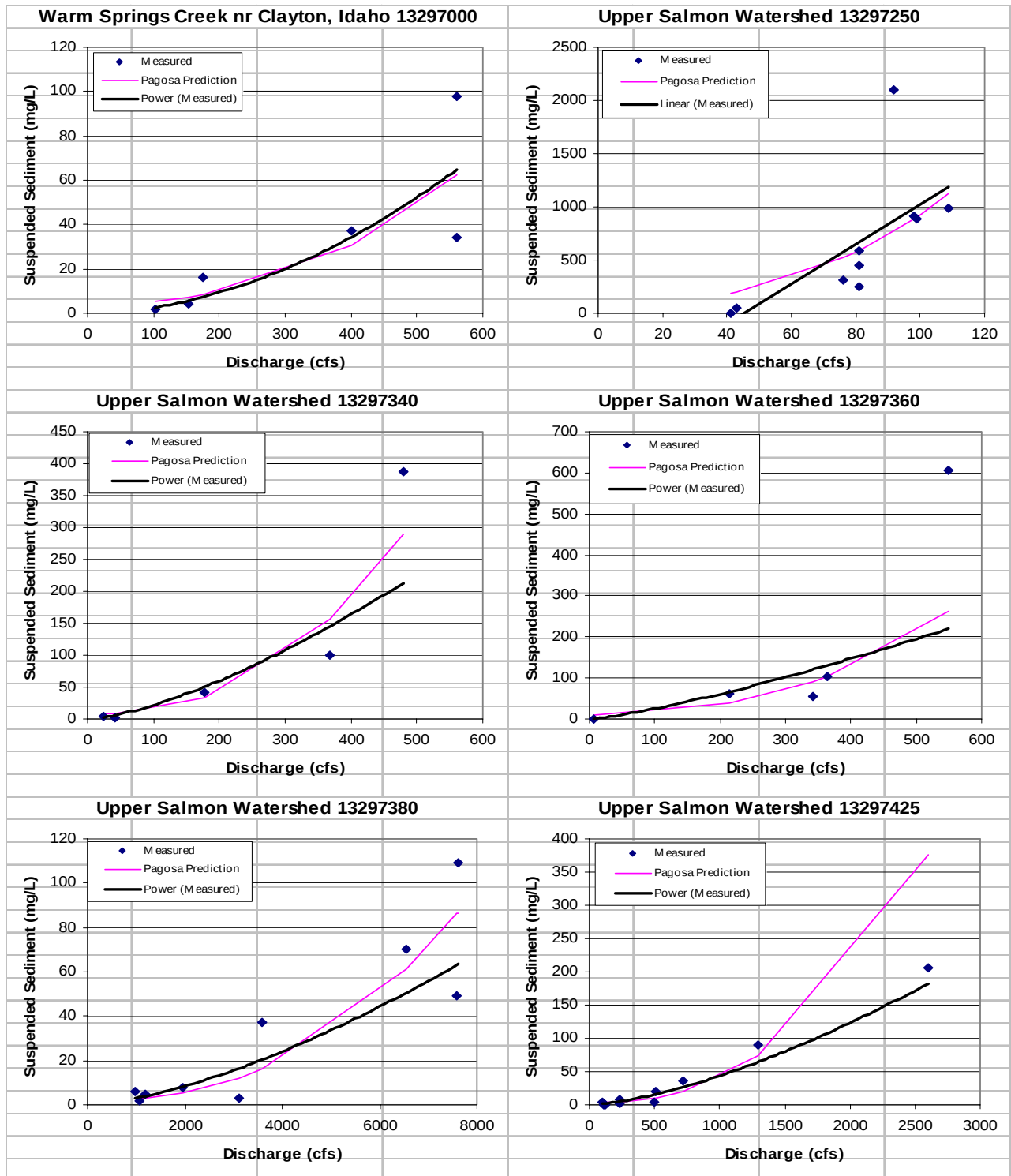
Figure 61. Example of predicted versus measured suspended sediment data using dimensionless reference curve (Data from Emmett, 1975)
