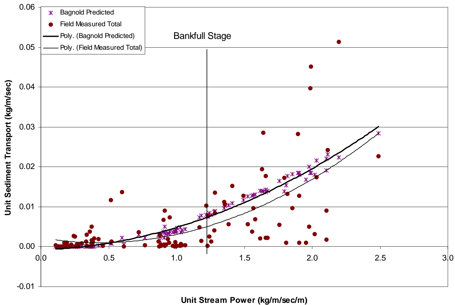
Figure 66. Comparison of predicted bedload using the Bagnold formula versus measured values for Upper Wolf Creek, Colorado.
