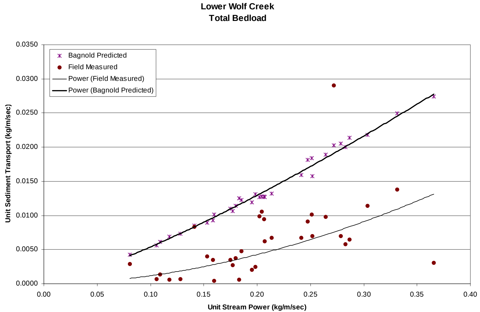
Figure 67. Predicted bedload transport using the Bagnold equation versus measured values on Lower Wolf Creek (D4 stream type).
