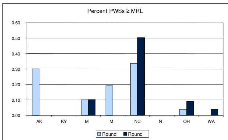
Exhibit 11-11: Distribution of 1,1,2,2-Tetrachloroethane Detections (above) and HRL Exceedances (below) Among Select Cross-Section States
