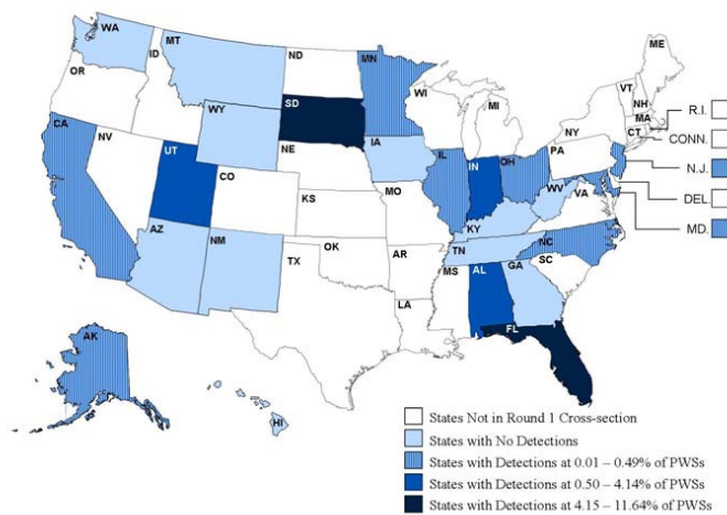
Exhibit 11-8: Geographic Distribution of 1,1,2,2-Tetrachloroethane Detection Frequencies in Cross-Section States (Above: UCM Round 1; Below: UCM Round 2)
