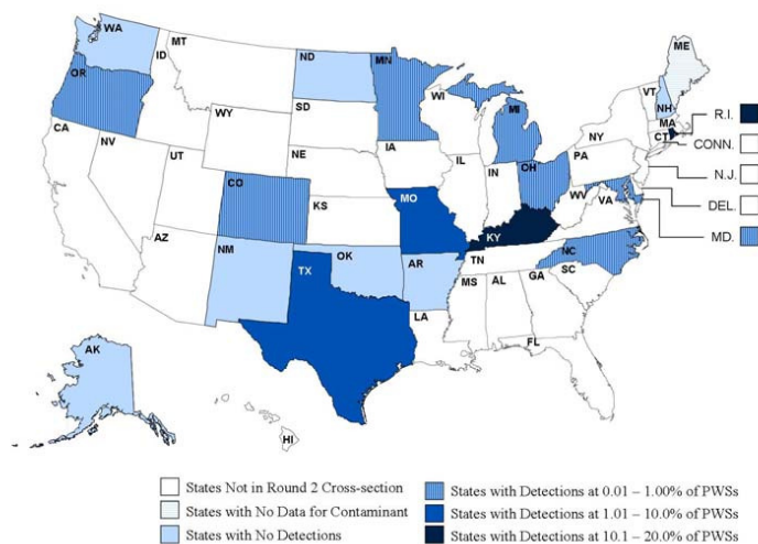
Exhibit 12-8: Geographic Distribution of Metolachlor Detection Frequencies in Cross-Section States (UCM Round 2)
