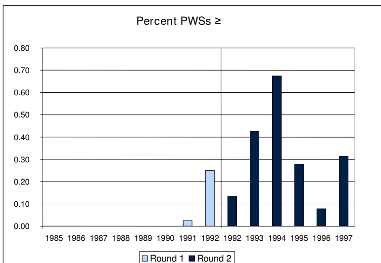
Exhibit 6-10: Annual Frequency of 1,3-Dichloropropene Detections (above) and HRL Exceedances (below), 1985 - 1997, in Select Cross-Section States
