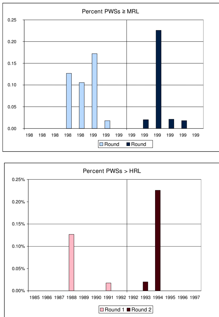
Exhibit 11-10: Annual Frequency of 1,1,2,2-Tetrachloroethane Detections (above) and HRL Exceedances (below), 1985 - 1997, in Select Cross-Section States
