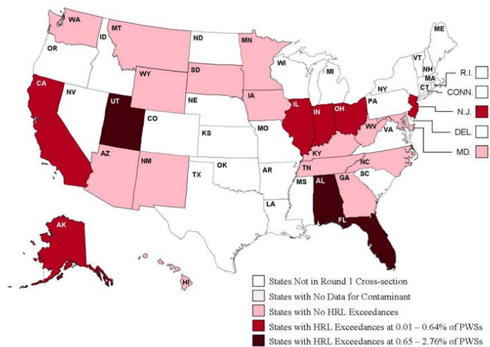
Exhibit 11-9: Geographic Distribution of 1,1,2,2-Tetrachloroethane HRL Exceedance Frequencies in Cross-Section States (Above: UCM Round 1; Below: UCM Round 2)
