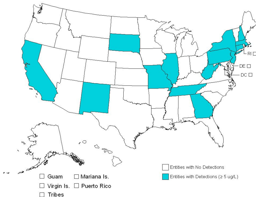
Exhibit 13-11: Geographic Distribution of MTBE in UCMR 1 Monitoring BStates With At Least One Detection At or Above the MRL ( \geq 5 \mu\text{g/L} )
