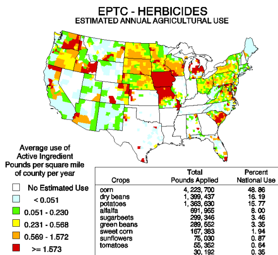
Exhibit 8-2: Estimated Annual Agricultural Use of EPTC, c. 1997
