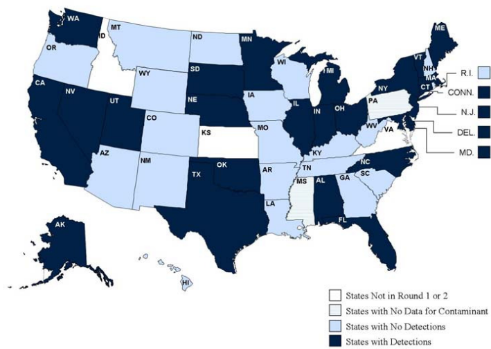
Exhibit 11-6: Geographic Distribution of 1,1,2,2-Tetrachloroethane Detections in Both Cross-Section and Non-Cross-Section States (Combined UCM Rounds 1 and 2)
