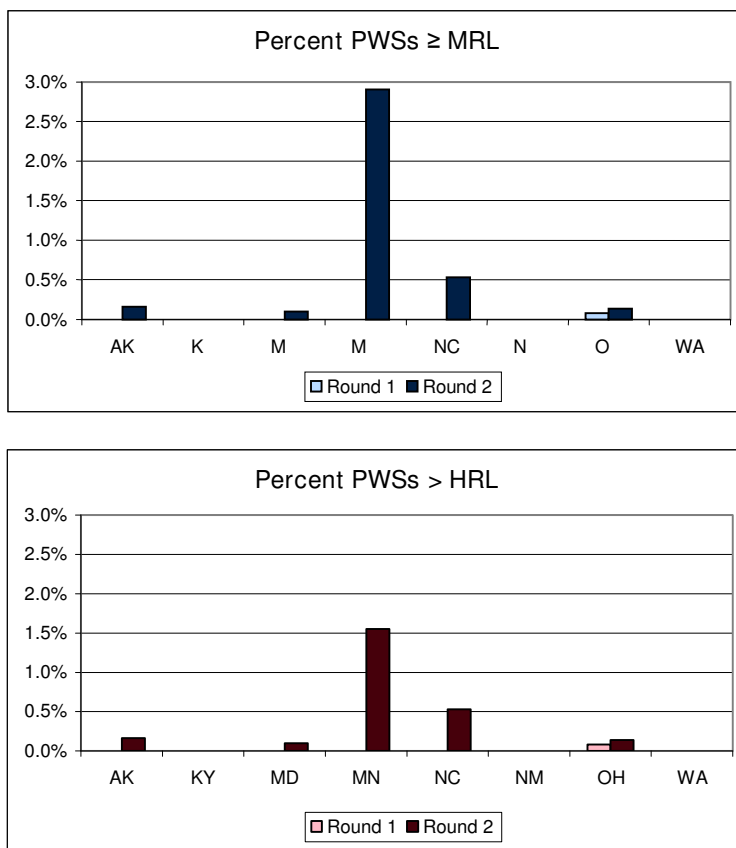
Exhibit 6-11: Distribution of 1,3-Dichloropropene Detections (above) and HRL Exceedances (below) Among Select Cross-Section States
