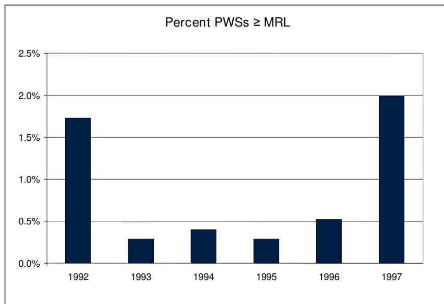
Exhibit 12-9: Annual Frequency of Metolachlor Detections, 1992-1997, in Cross-Section States
