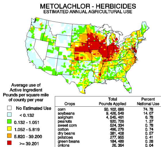
Exhibit 12-2: Estimated Annual Agricultural Use of Metolachlor, c. 1997
