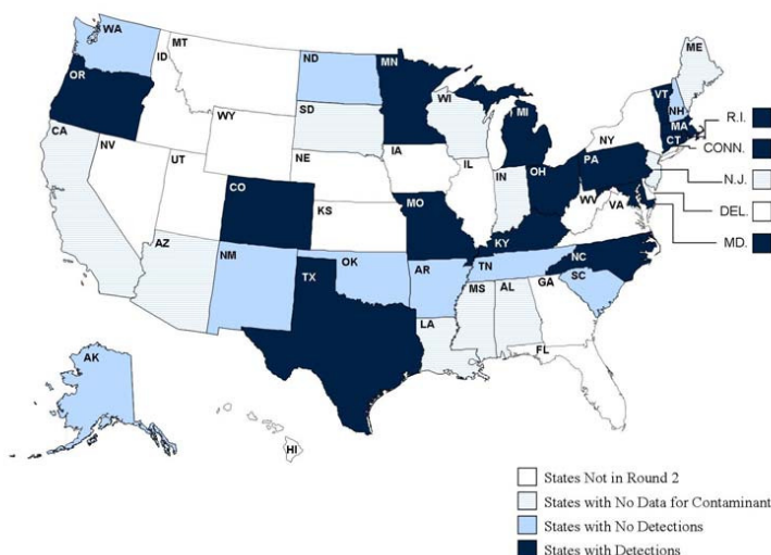
Exhibit 12-7: Geographic Distribution of Metolachlor Detections in Both Cross-Section and Non-Cross-Section States (UCM Round 2)
