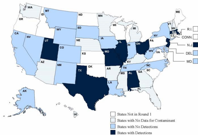
Exhibit 6-7: Geographic Distribution of 1,3-Dichloropropene Detections in Both Cross-Section and Non-Cross-Section States (Above: UCM Round 1; Below: UCM Round 2)
