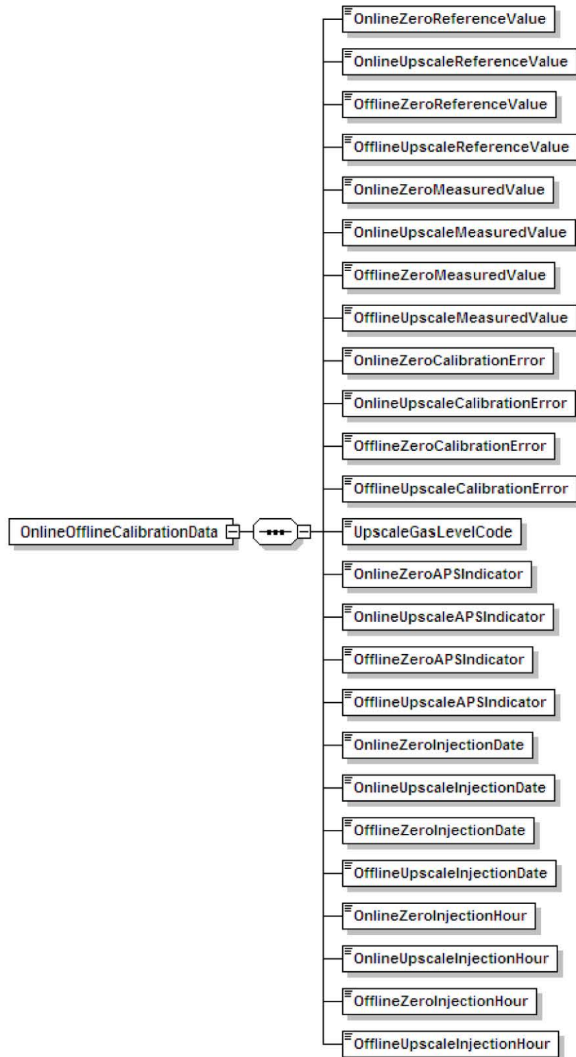
Figure 30: Online Offline Calibration Data XML Elements
