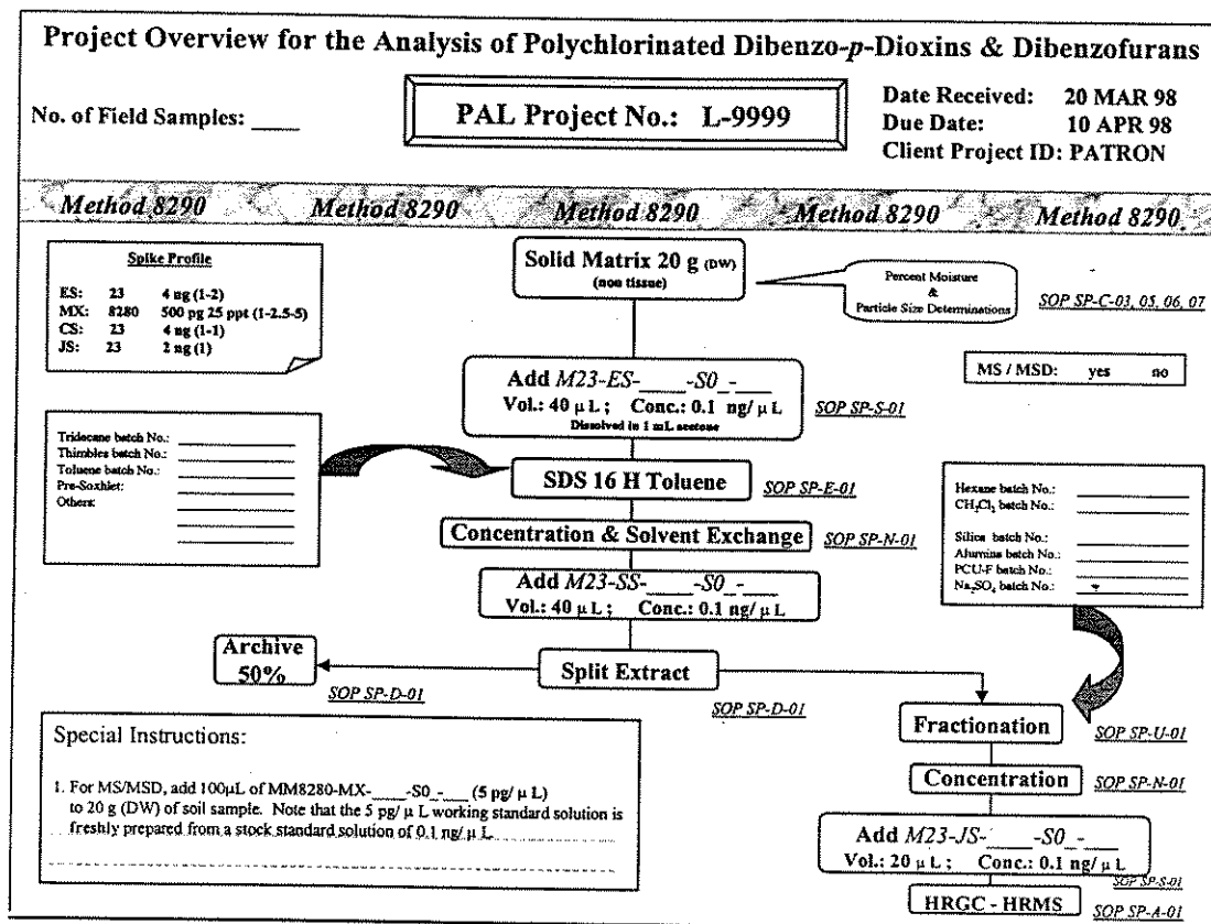
Figure 1: Schematic representation of Method 8290 for solids using the SDS extraction technique.
