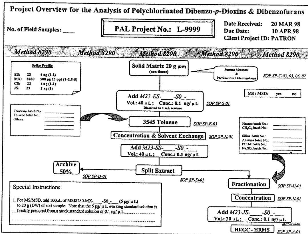
Figure 2: Schematic representation of Method 8290 for solids using Method 3545 extraction technique.
