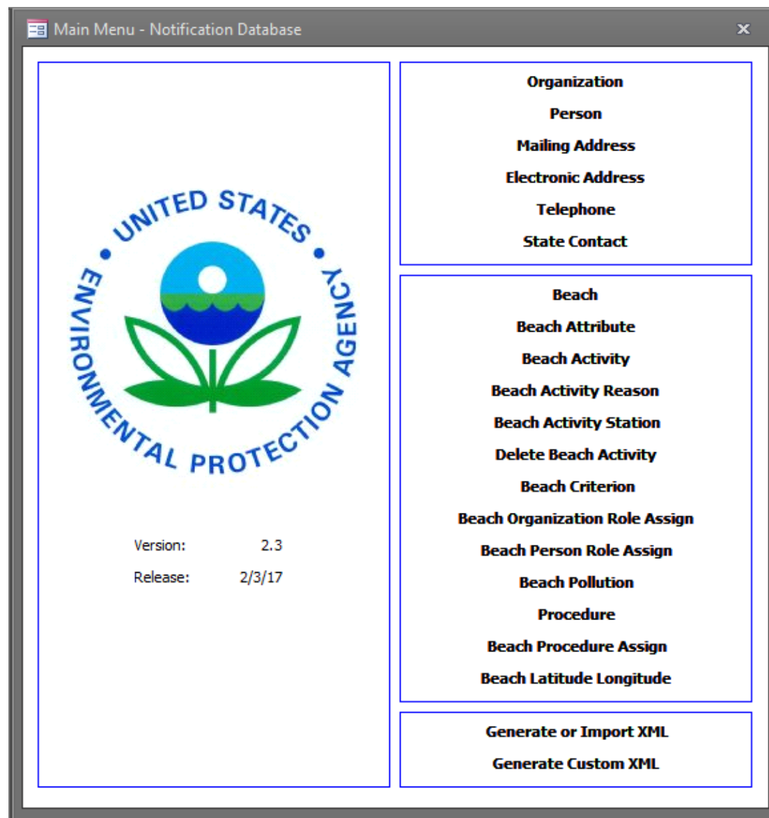
Exhibit 13-2 Main Menu
