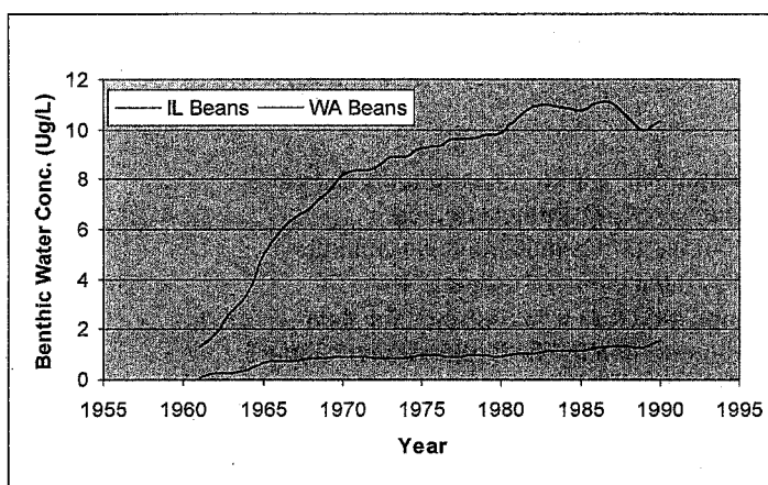
Figure 4. Accumulation of flubendiamide in benthic pore water of the PRZM/EXAMS standard pond under a low exposure scenario with Washington Beans and a high exposure scenario with Illinois Beans based on annual peak concentrations.
