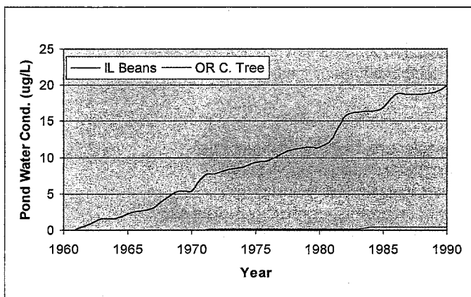
Figure 5. Accumulation of the flubendiamide des-iodo degradate in water column of the PRZM/EXAMS standard pond under a low exposure scenario of Oregon Christmas Tree and a high exposure scenario of Illinois Beans.
