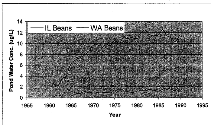
Figure 3. Accumulation of flubendiamide in water column of the PRZM/EXAMS standard pond under a low exposure scenario with Washington Beans and a high exposure scenario with Illinois Beans based on annual peak concentrations.
