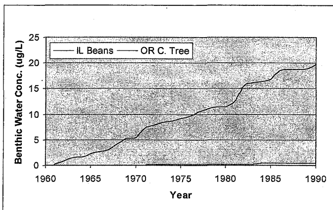
Figure 6. Accumulation of the flubendiamide des-iodo degradate in benthic pore water of the PRZM/EXAMS standard pond under a low exposure scenario of Oregon Christmas Tree and a high exposure scenario of Illinois Beans.
