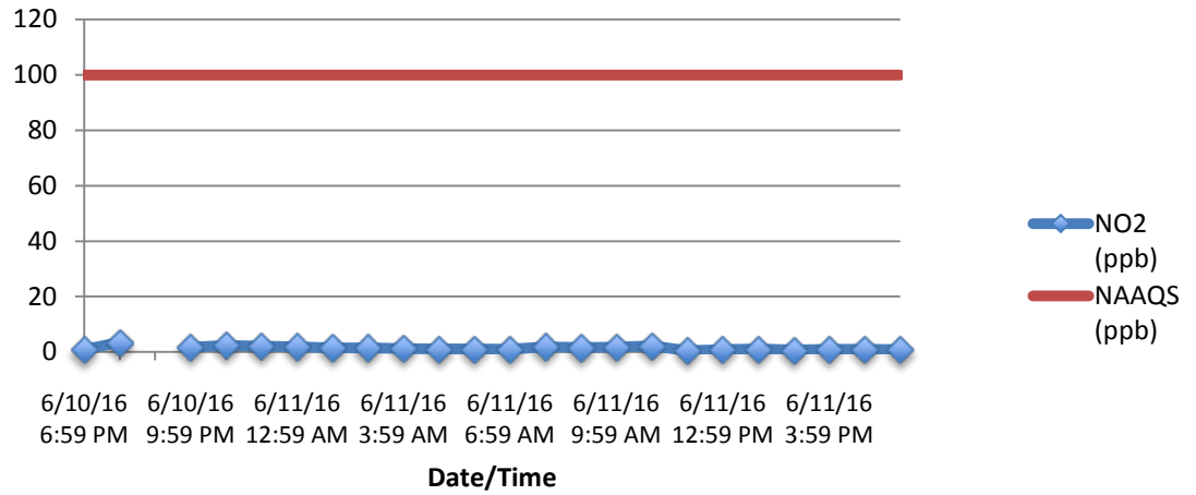
Hourly Averages NO2 (ppb)
