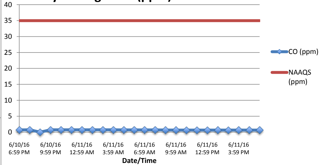
Hourly Averages CO (ppm)
