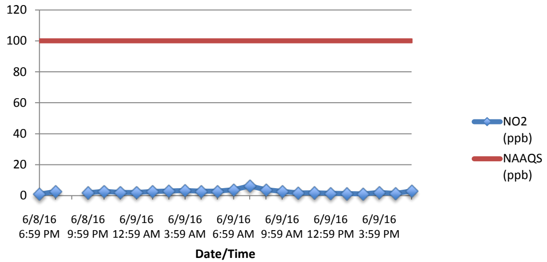
Hourly Averages NO2 (ppb)
