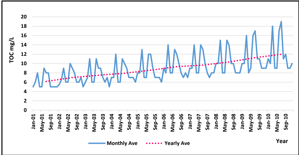
Figure 6-5. Example Plots of Monthly Average and Yearly Average for Source Water TOC
