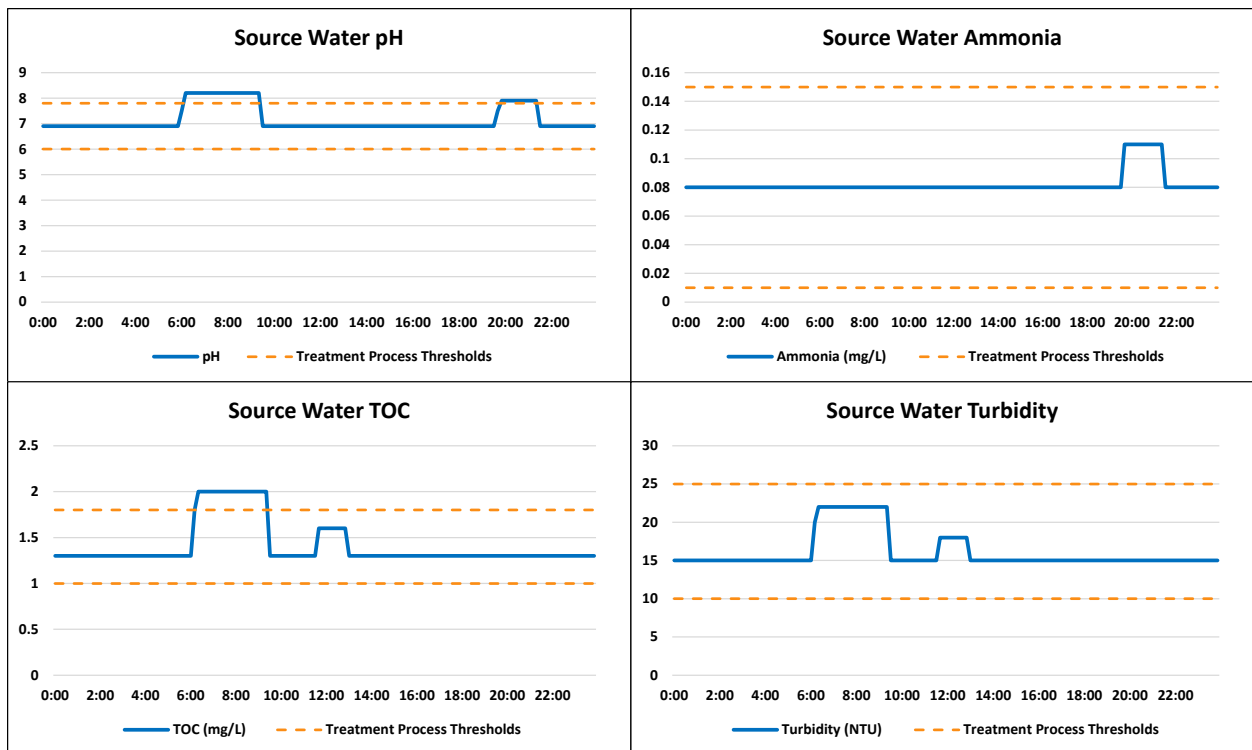
Figure 6-1. Time-Series Plots and Thresholds for Treatment Process Optimization
