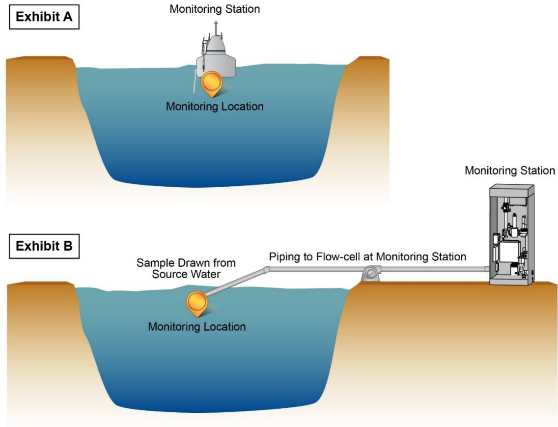
Figure 1-3. Monitoring Location vs. Monitoring Station
