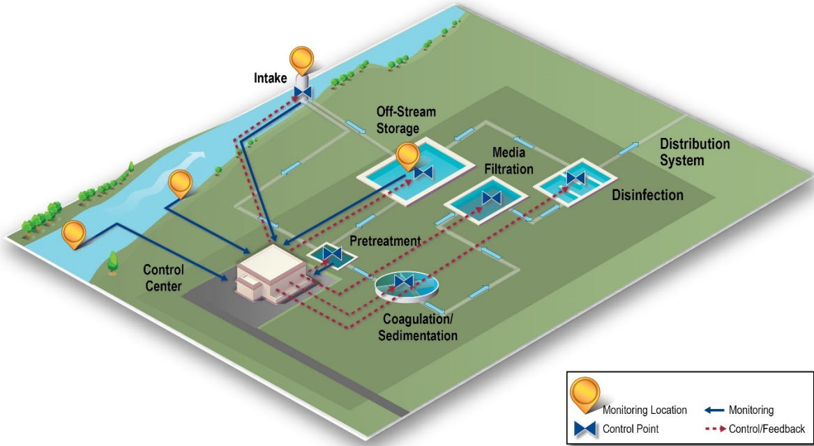
Figure 1-2. Example Schematic of OWQM-SW
