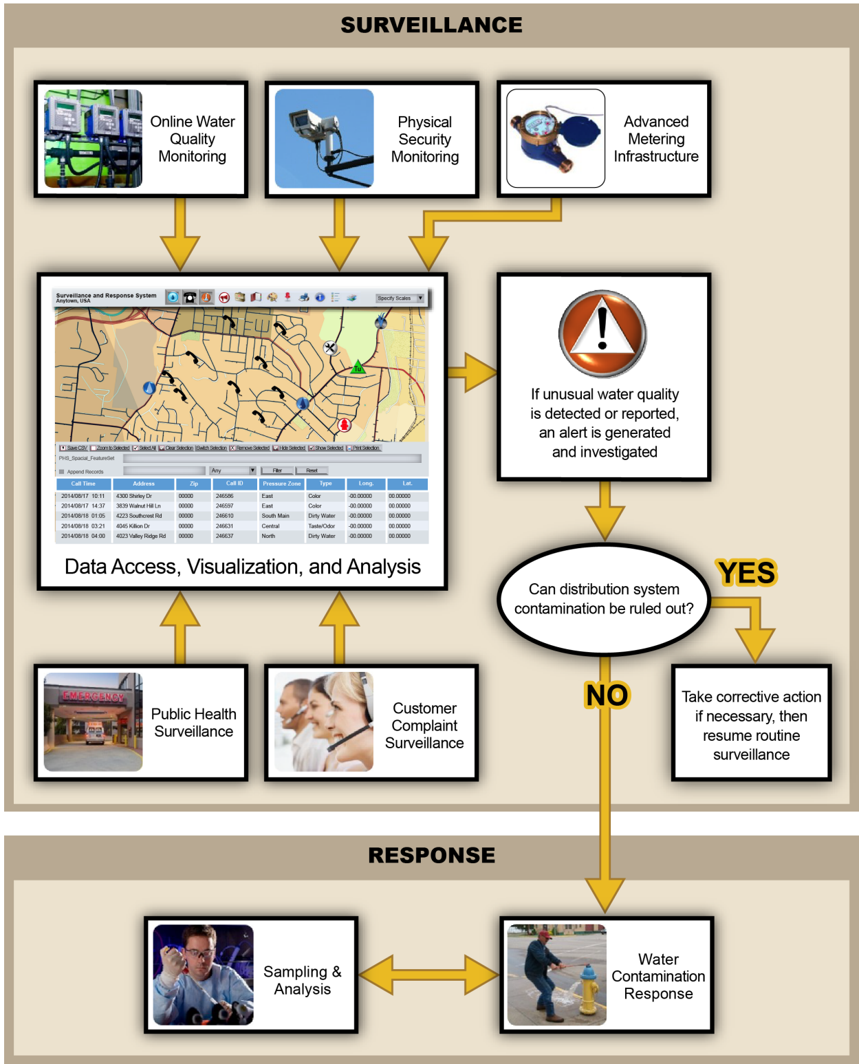
Figure 1-1. Incorporation of OWQM-SW into an SRS
