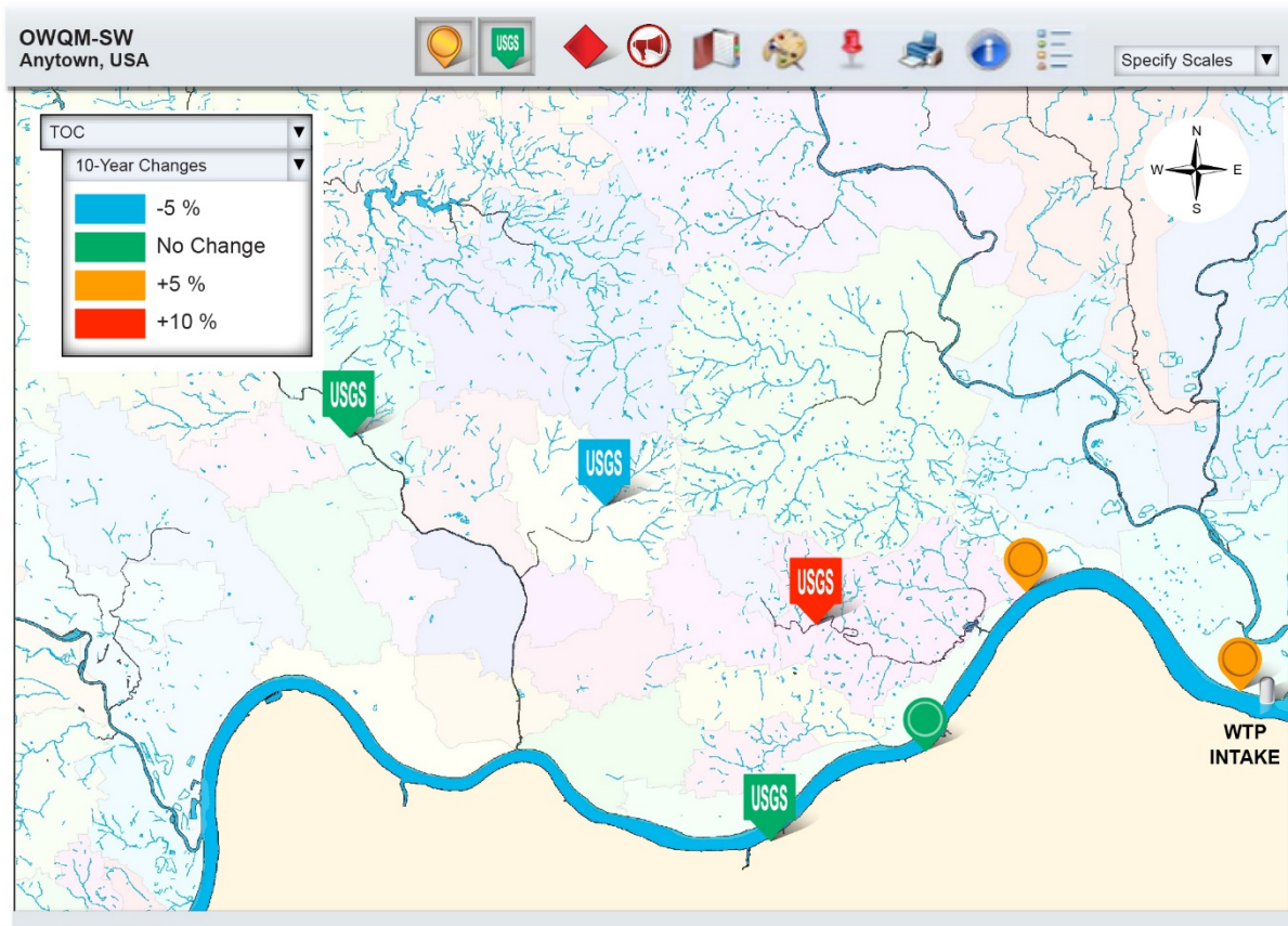
Figure 6-6. Geospatial Presentation Showing the Change in TOC over a 10-Year Period
