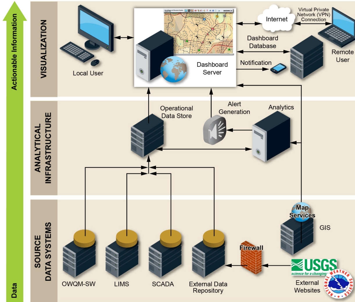
Figure 6-8. Example of a Dedicated OWQM-SW Information Management System
