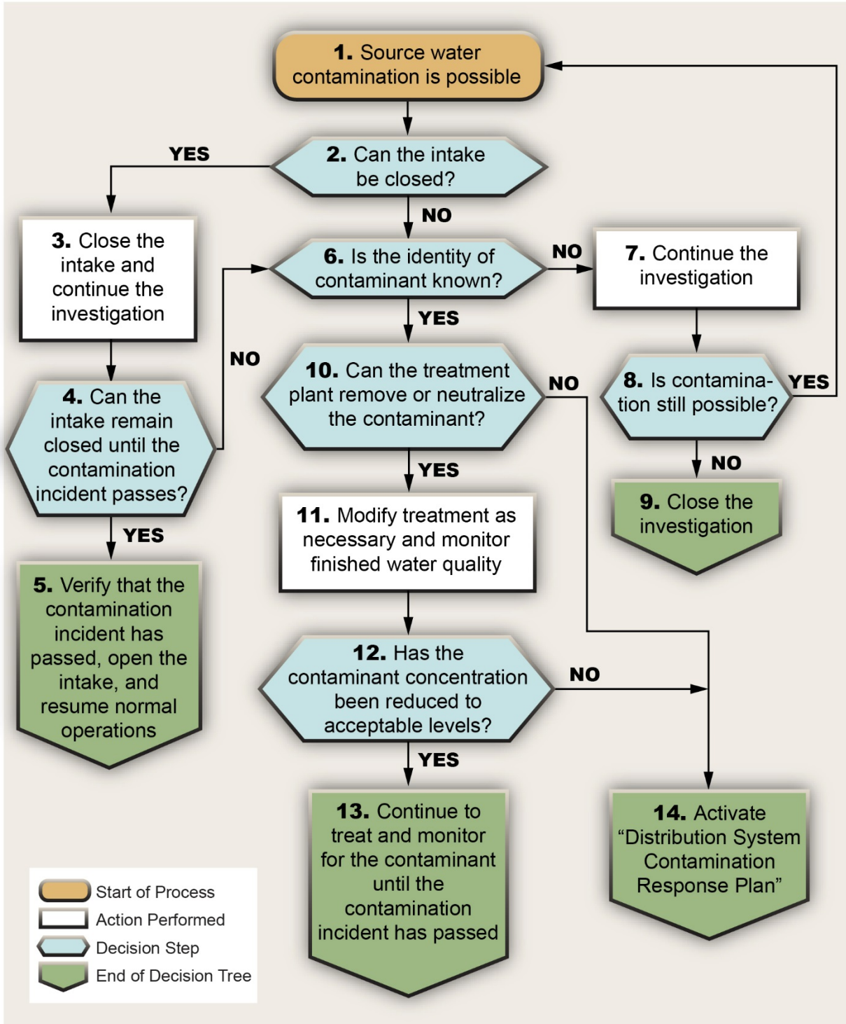
Figure 7-3. Example Source Water Contamination Incident Response Decision Tree
