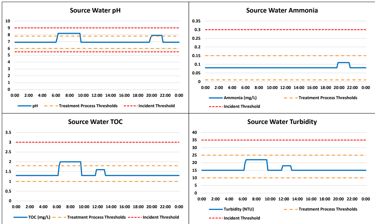
Figure 6-2. Time-Series Plots and Thresholds for Detection of Contamination Incidents
