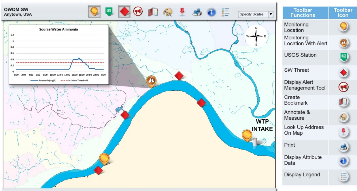
Figure 6-3. OWQM-SW Display showing Alert Status and Time-Series Data for an OWQM-SW Location
