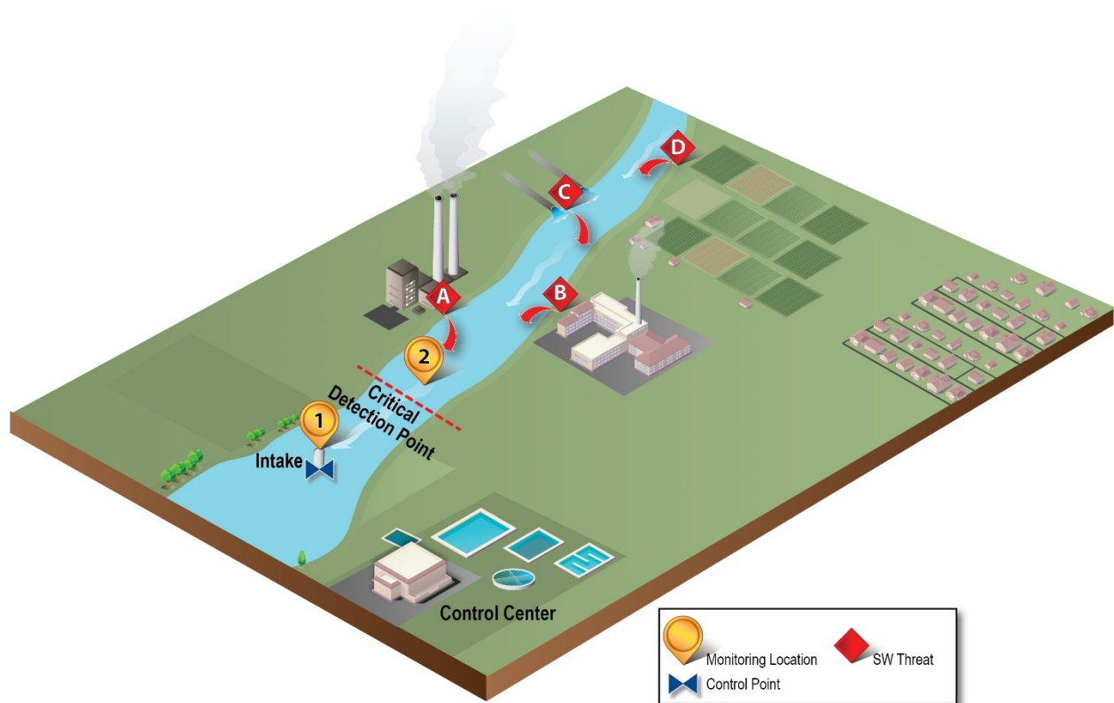
Figure 3-2. A Single Upstream Monitoring Location to Monitor Multiple SW Threats
