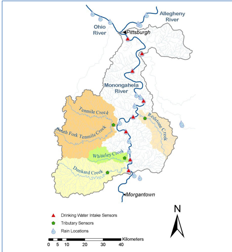
Figure 9-10. Overview of RAIN Monitoring Locations
