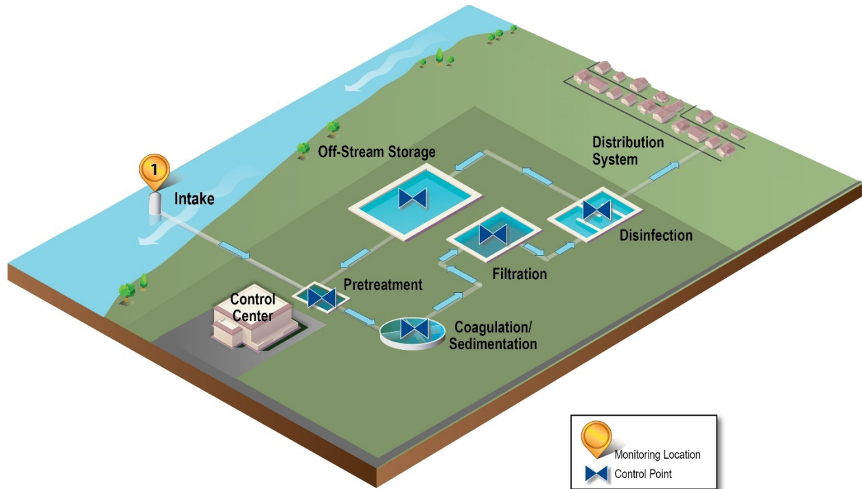
Figure 3-1. Monitoring Location Selected to Support Treatment Process Optimization
