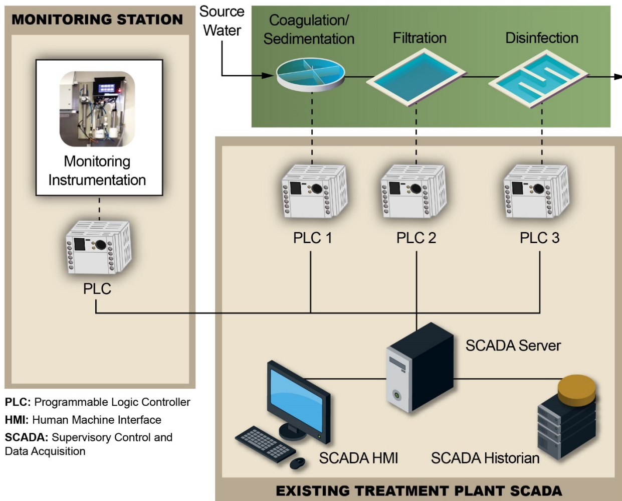
Figure 6-7. OWQM-SW Information Management as an Extension of an Existing SCADA Architecture
