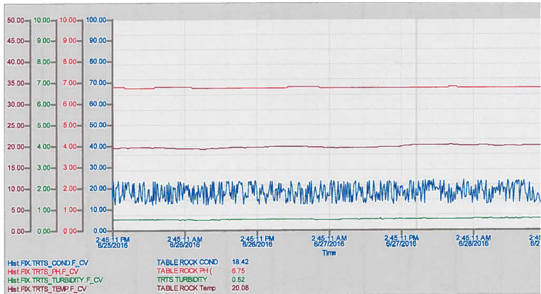
Figure 9-2. Example of Greenville Water SCADA System Screen for OWQM-SW Data
