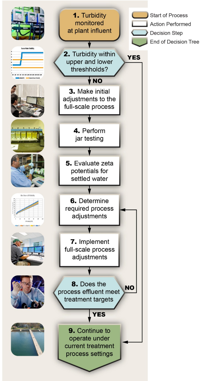
Figure 7-2. Example Treatment Optimization Procedure Flow Diagram
