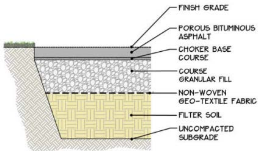
Exhibit 14-6. Example Porous Asphalt Cross-section (Source: EPA, 2009)
