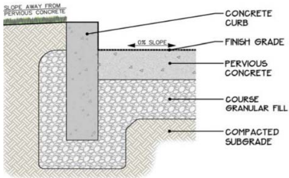
Exhibit 14-5. Example Pervious Concrete Cross-section (Source: EPA, 2009)
