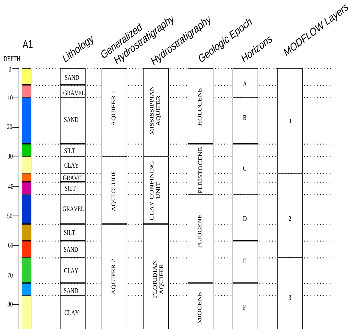
Figure A-2 Example of Geologic Units
