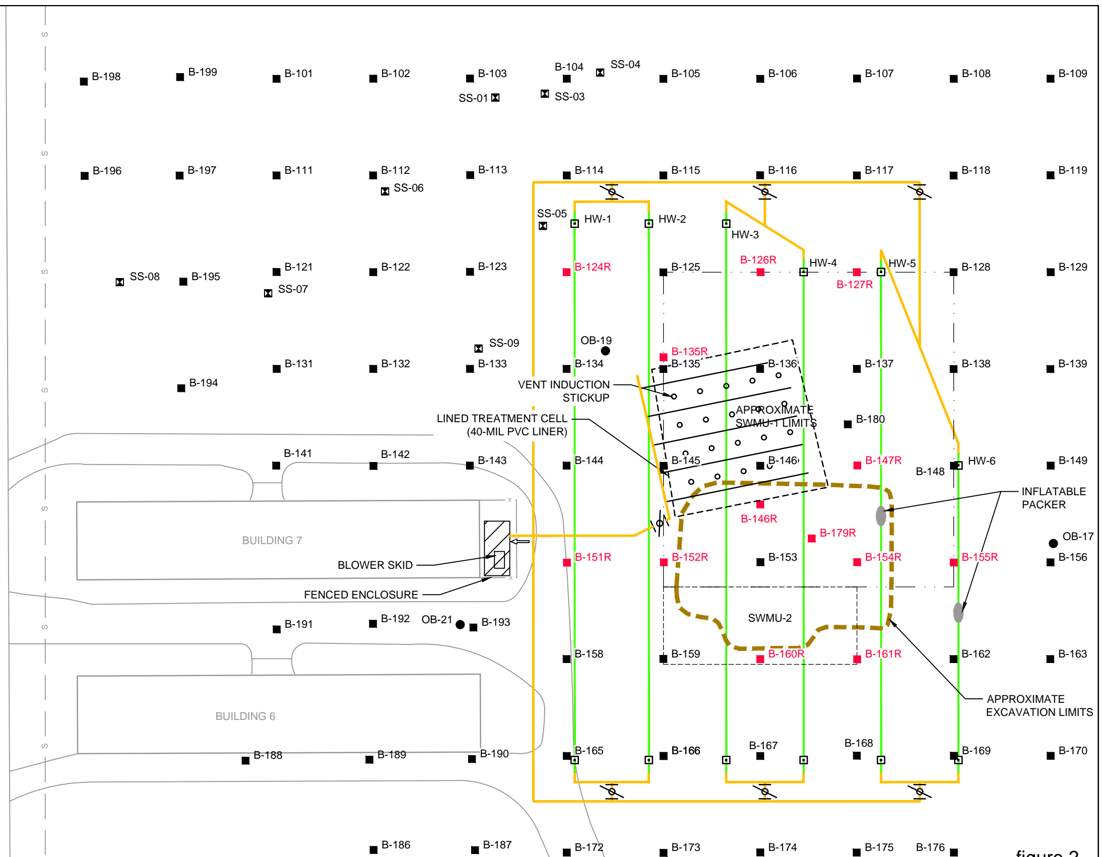
figure 2 SWMU 1 & 2 SVE CONFIGURATION AND SOIL SAMPLE LOCATIONS RADIO MATERIALS CORPORATION Attica, Indiana
