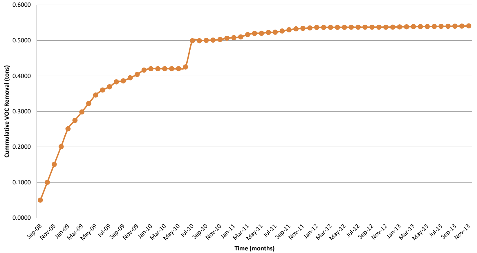
SWMU 1 and 2 - Primary VOC Removal vs. Time
