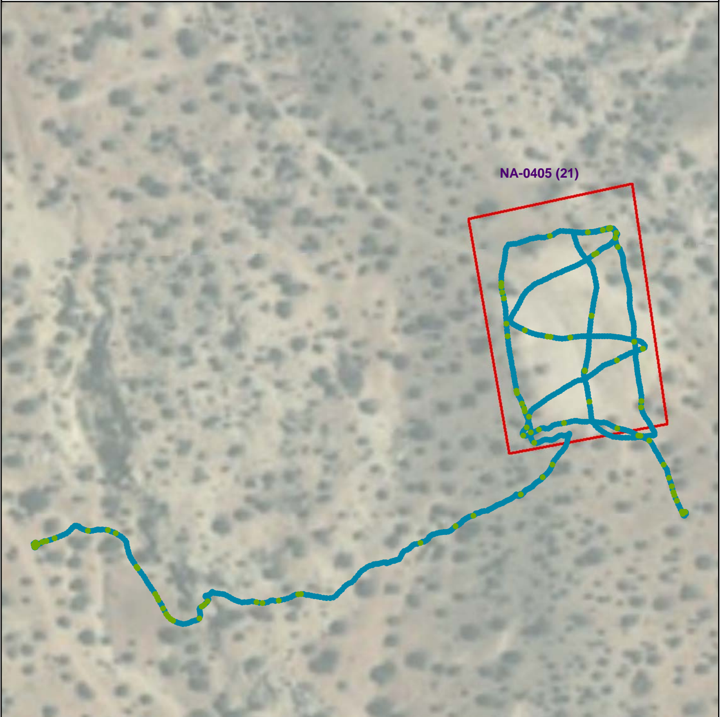
Figure 2 - Gamma Radiation Measurements NA-0405 (21) Red Valley Chapter, Navajo Nation, Arizona
