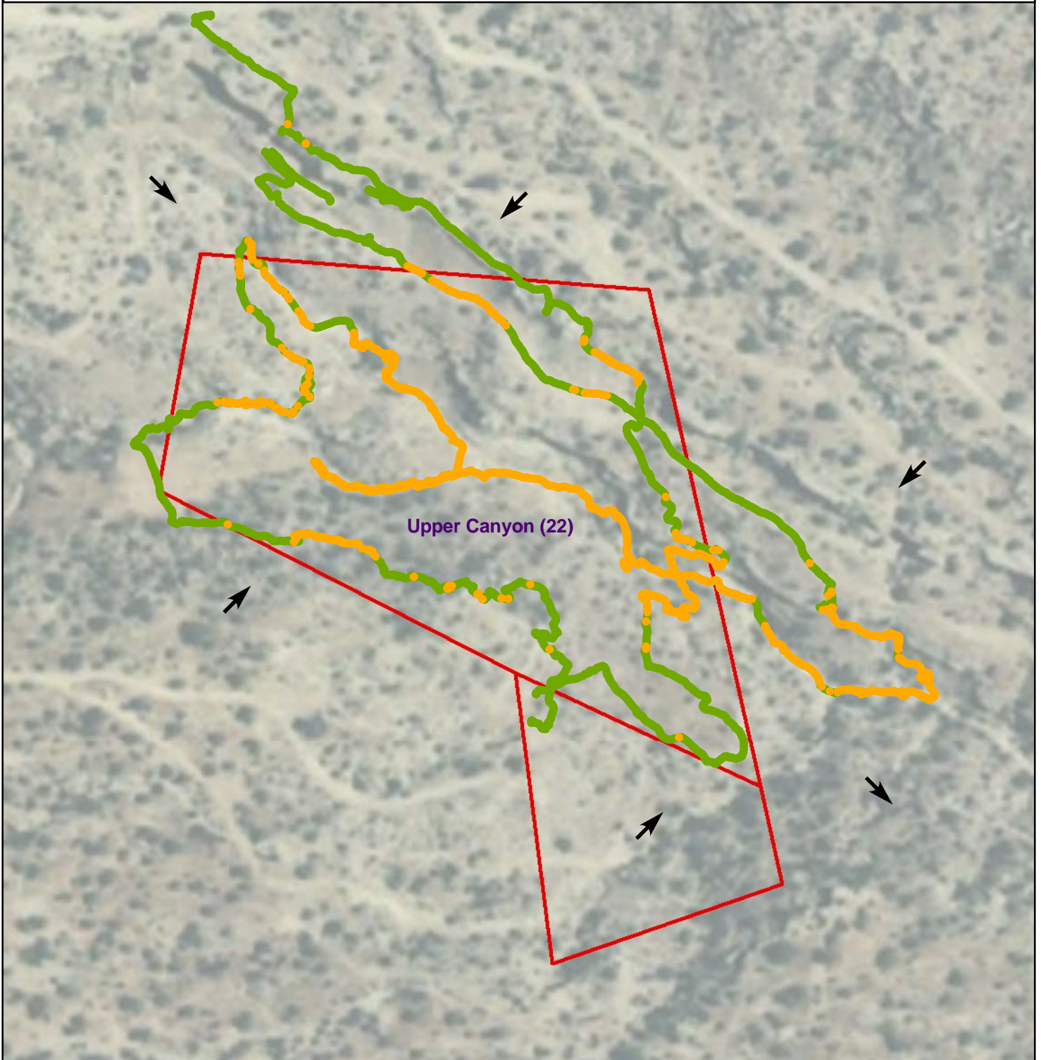
Figure 1 - Gamma Radiation Measurements, Above Two Times Background Upper Canyon (22) Red Valley Chapter, Navajo Nation, Arizona
