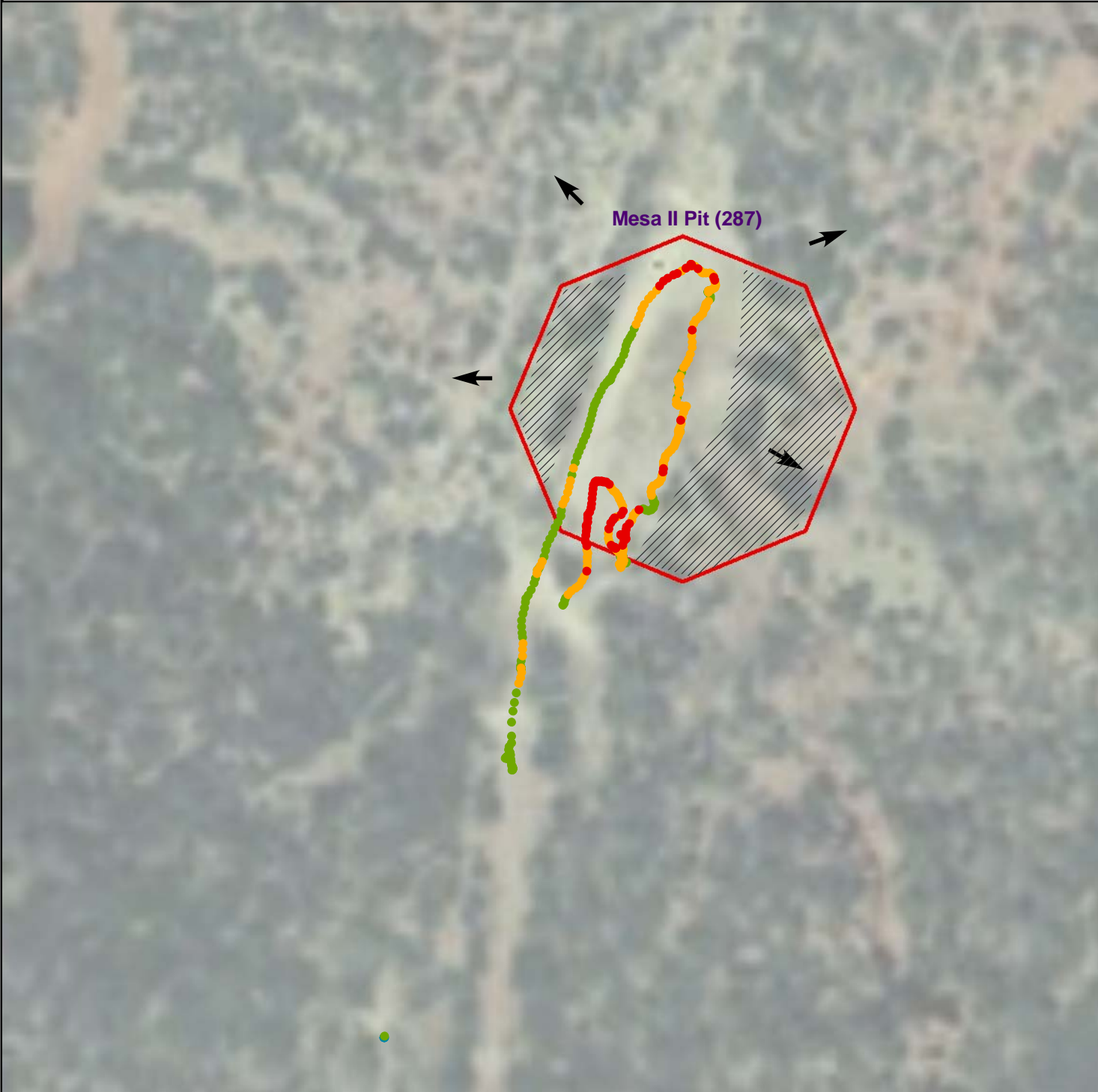
Figure 2 - Gamma Radiation Measurements Mesa II Pit (287) Cove Chapter, Navajo Nation, Arizona
