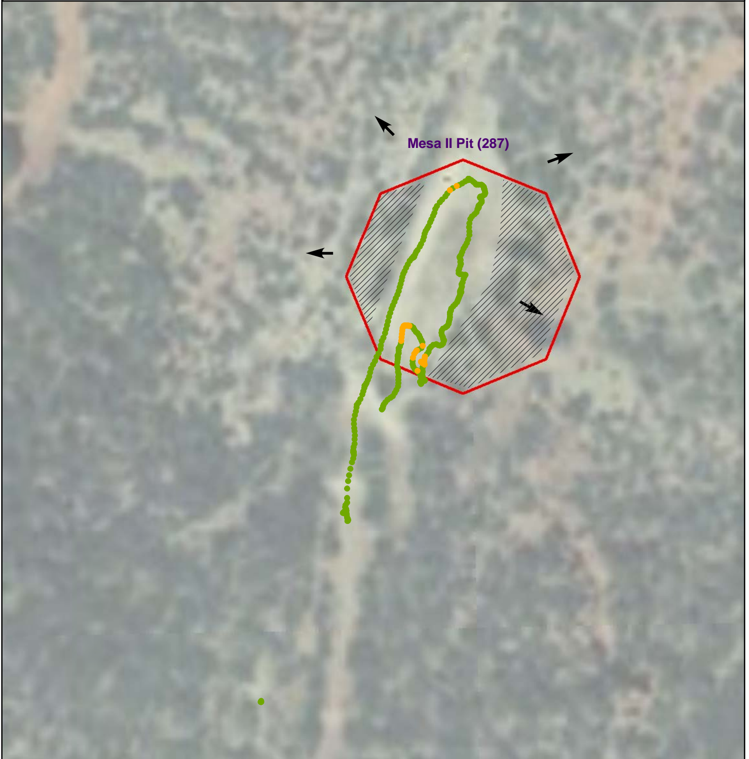
Figure 1 - Gamma Radiation Measurements, Above Two Times Background Mesa II Pit (287) Cove Chapter, Navajo Nation, Arizona
