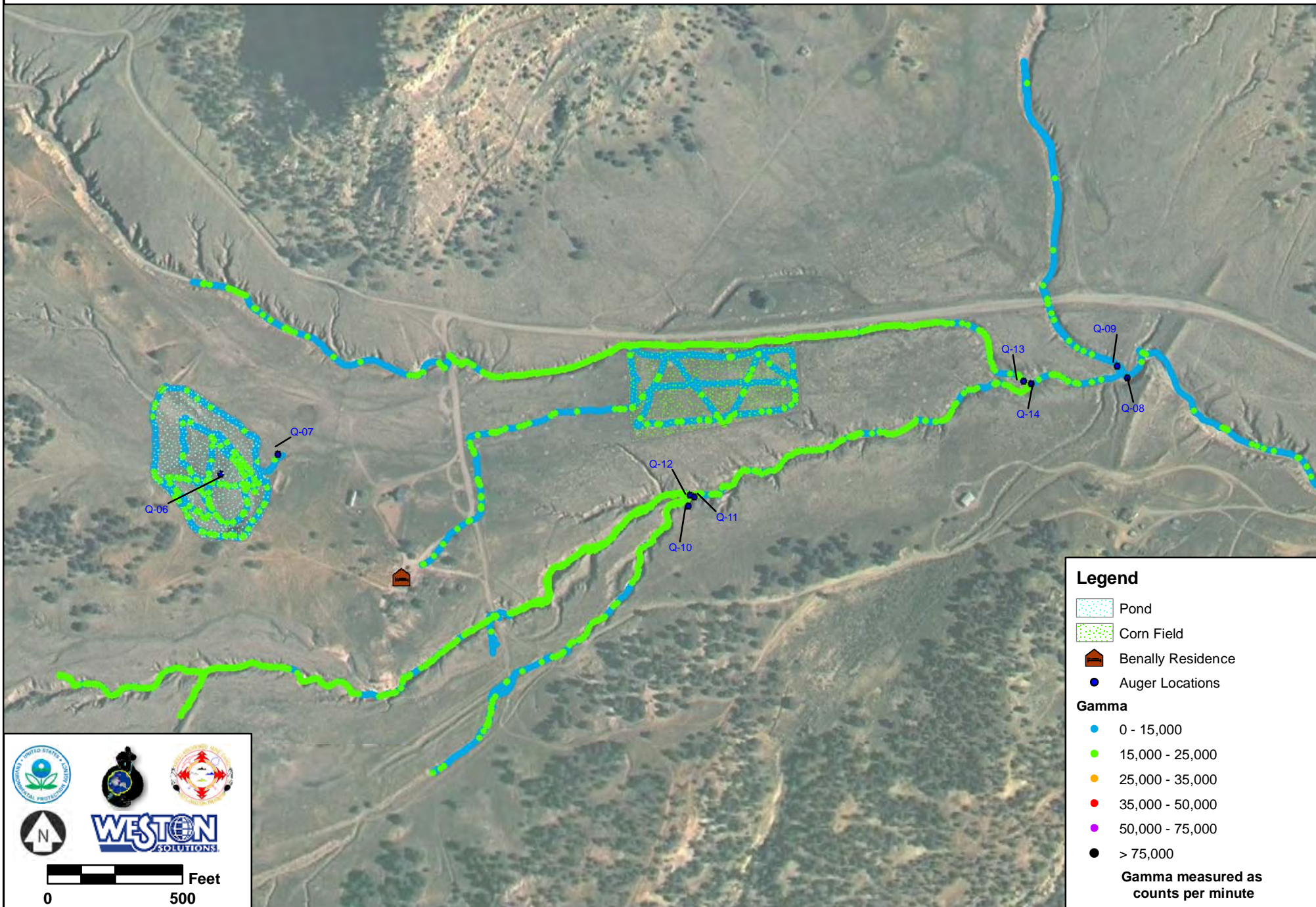
Figure 7 Western Area Gamma Radiation Measurements Northeast Church Rock - Quivira Mines Navajo Nation, New Mexico
