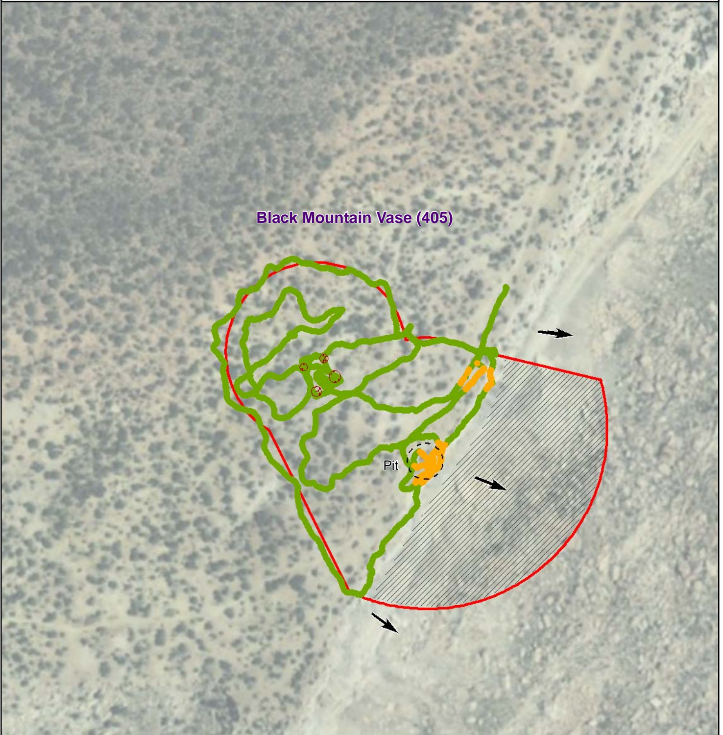
Figure 1 - Gamma Radiation Measurements, Above Two Times Background Black Mountain Vase (405) Tselani Chapter, Navajo Nation
