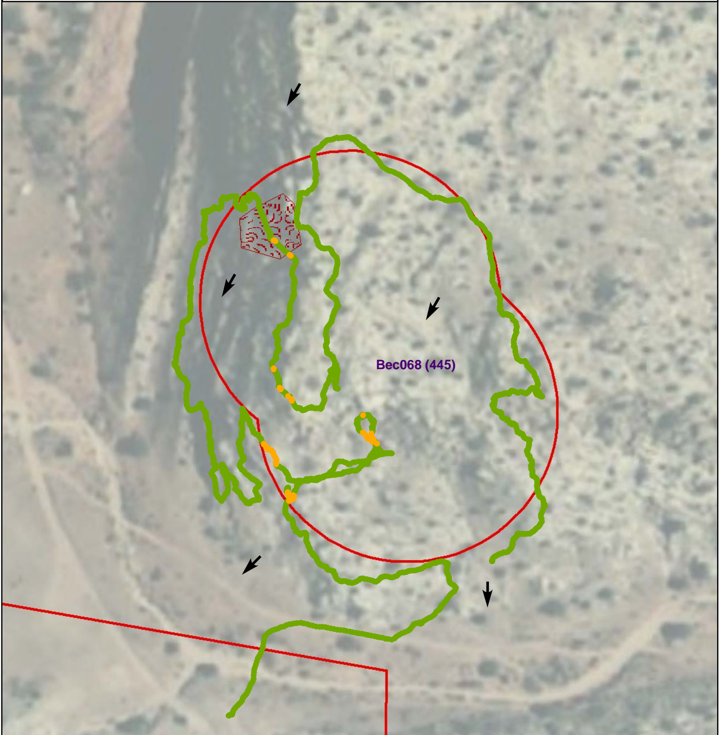
Figure 1 - Gamma Radiation Measurements, Above Two Times Background Bec068 (445) Beclabito Chapter, Navajo Nation, Arizona
