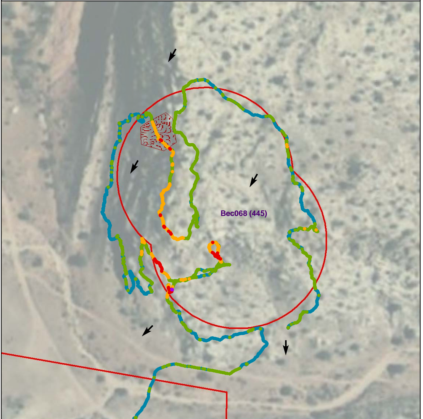
Figure 2 - Gamma Radiation Measurements Bec068 (445) Beclabito Chapter, Navajo Nation, Arizona
