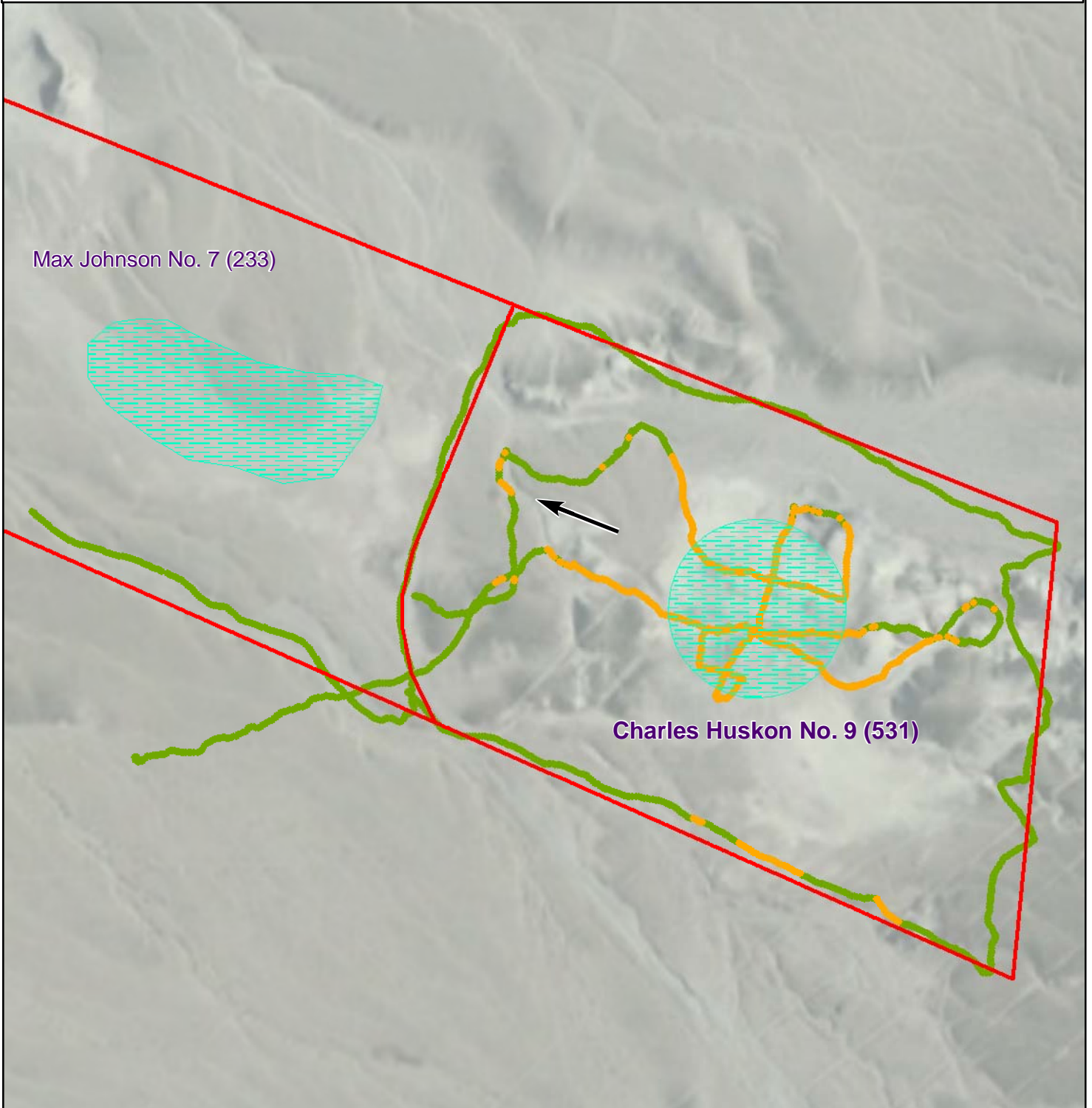
Figure 1 - Gamma Radiation Measurements, Above Two Times Background Charles Huskon No. 9 (531) Coalmine Mesa Chapter, Navajo Nation
