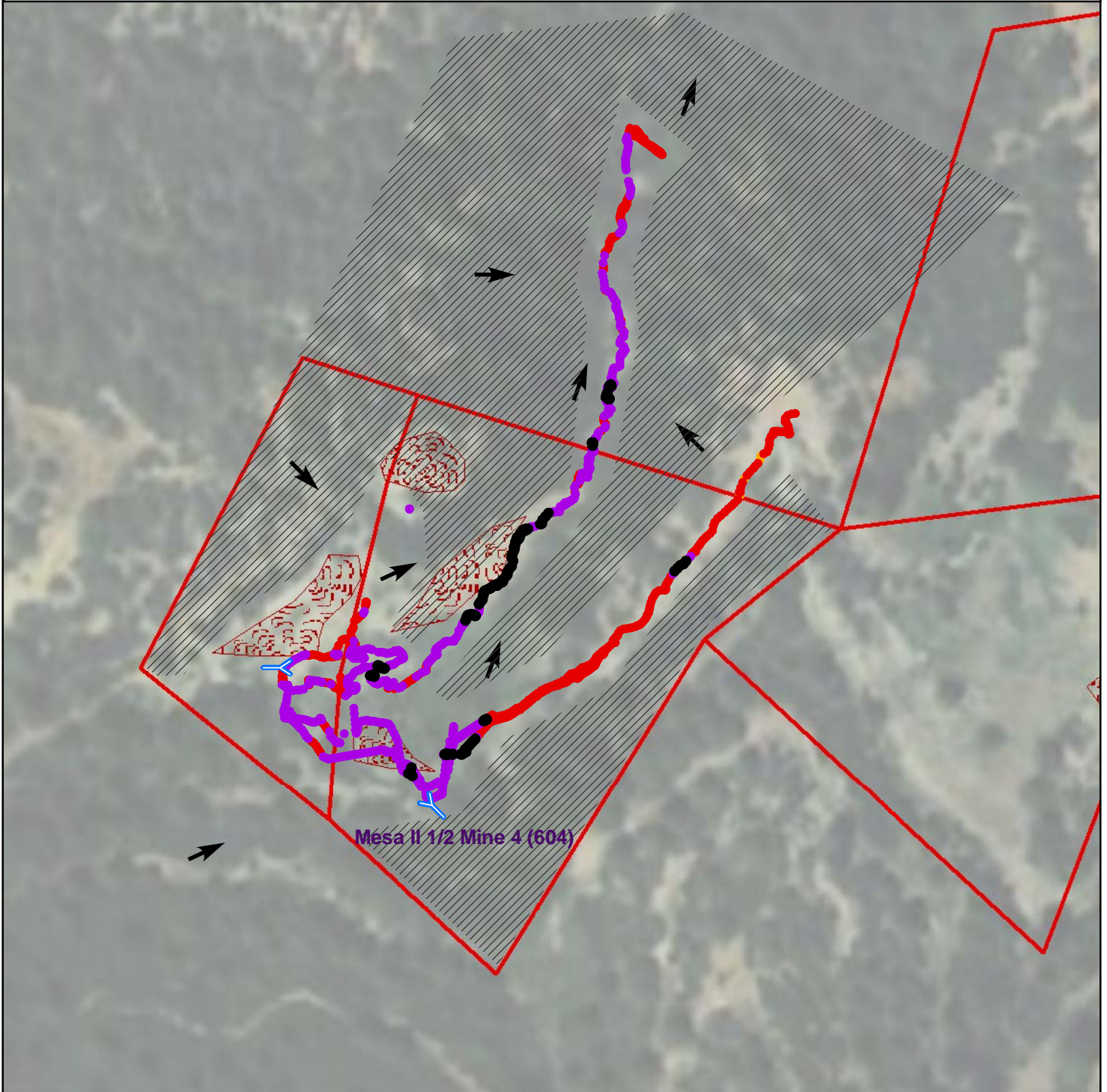
Figure 2 - Gamma Radiation Measurements Mesa II 1/2 Mine 4 (604) Cove Chapter, Navajo Nation, Arizona
