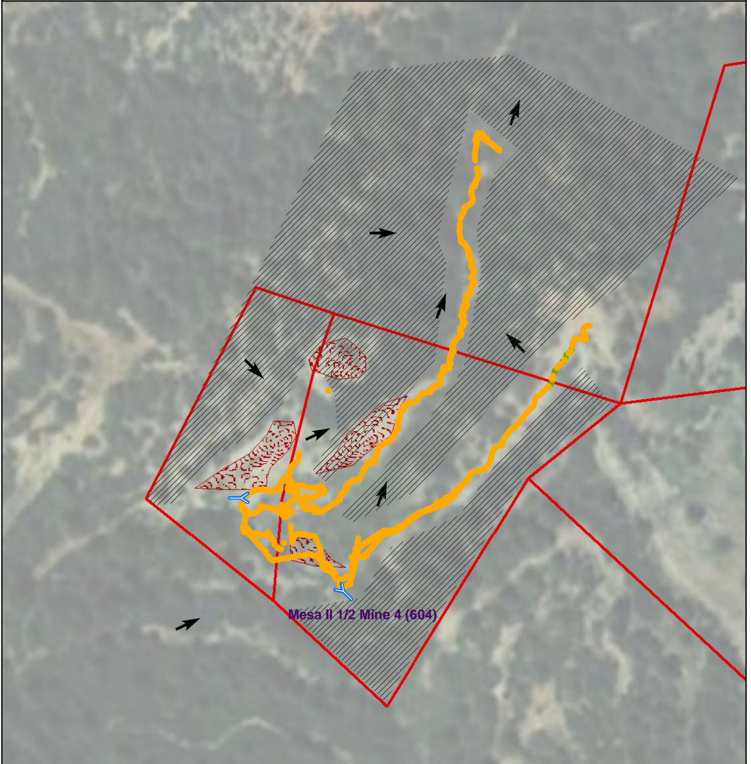
Figure 1 - Gamma Radiation Measurements, Above Two Times Background Mesa II 1/2 Mine 4 (604) Cove Chapter, Navajo Nation, Arizona
