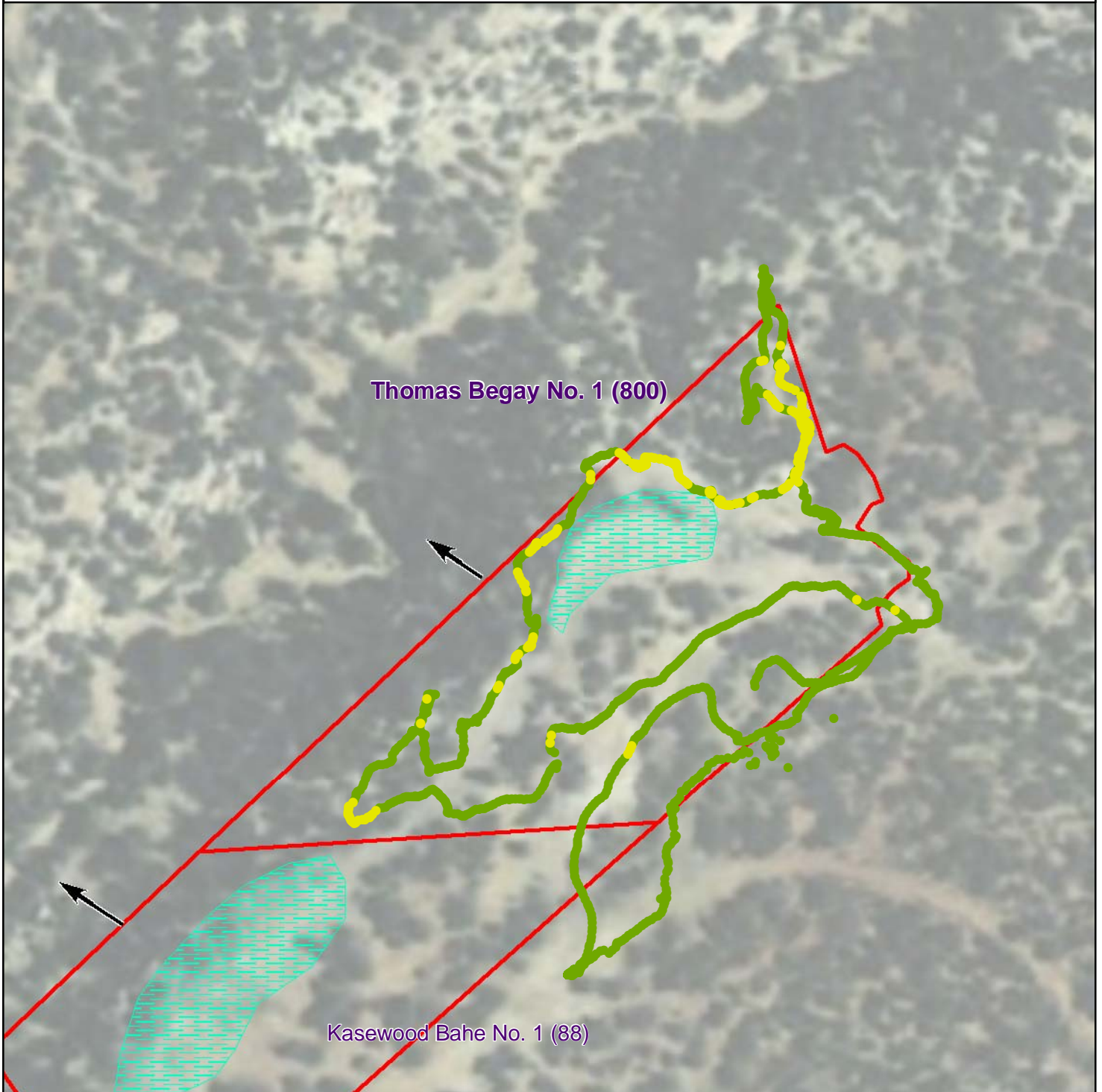
Figure 2 - Gamma Radiation Measurements Thomas Begay No. 1 (800) Black Mesa Chapter, Navajo Nation
