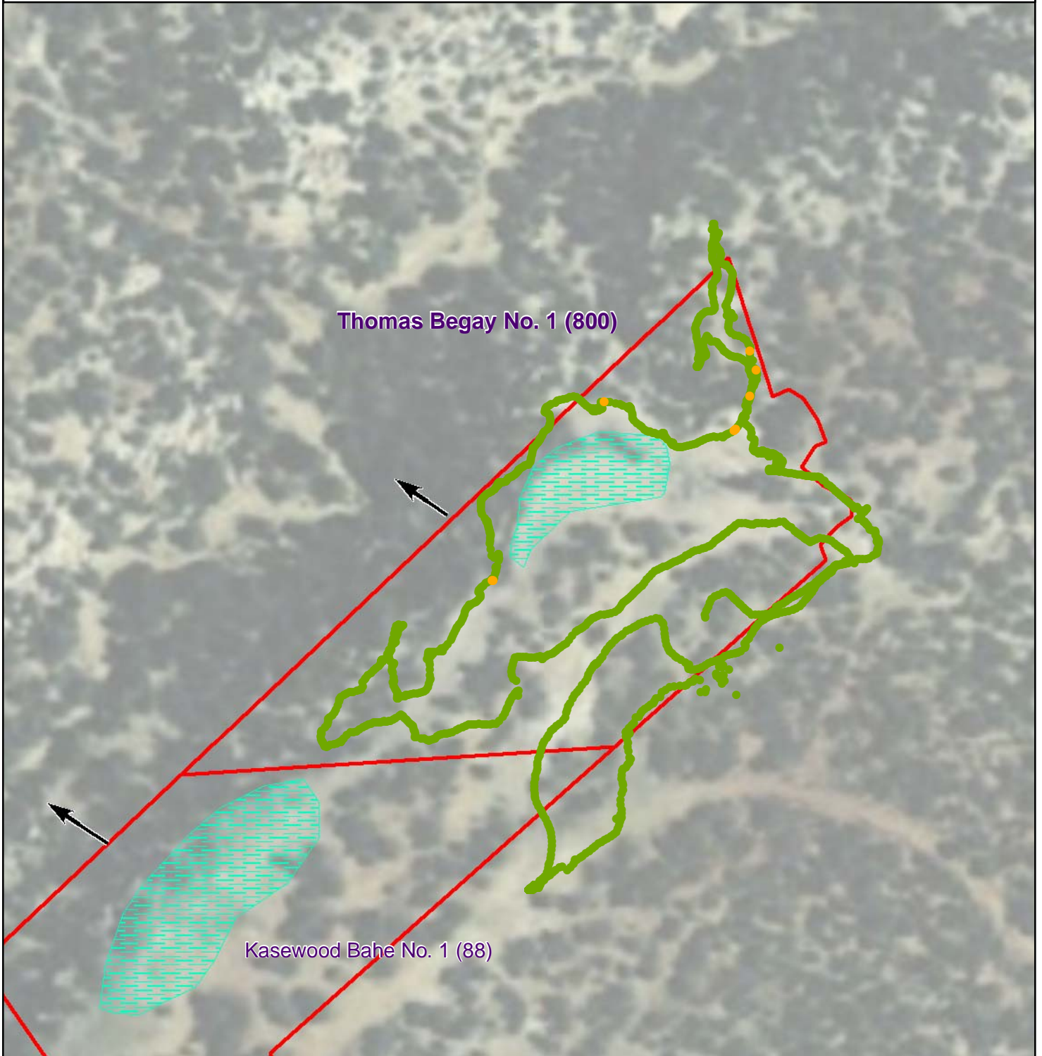
Figure 1 - Gamma Radiation Measurements, Above Two Times Background Thomas Begay No. 1 (800) Black Mesa Chapter, Navajo Nation
