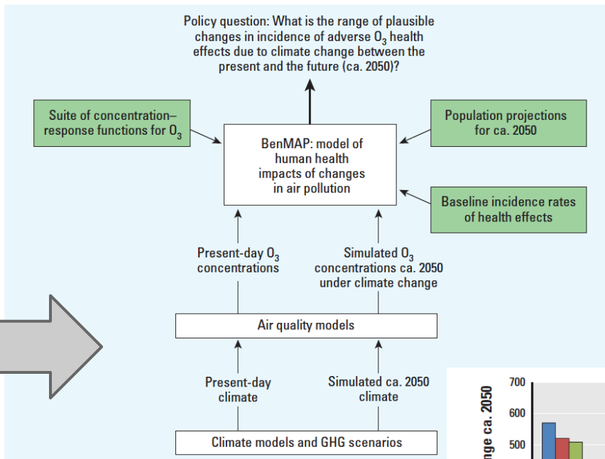
Figure 1. The structure of the analysis of O 3 -related impacts on human health. GHG, greenhouse gas.
